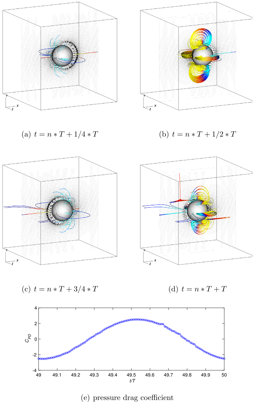
Fig. 15. In-line oscillating sphere at Re = 78.54 and St = 1.2732 . (a-d) instantaneous velocity vectors together with streamlines coloured by the pressure; (e) time history of the pressure drag coefficient plotted for every time step.
