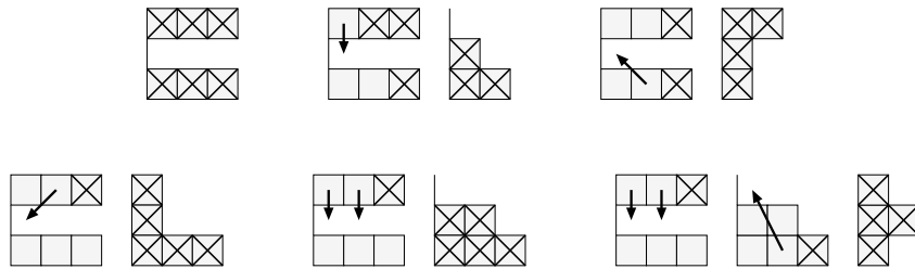
Fig. 7: The set \mathcal{G}(3, 0, 3) of all games on (3, 0, 3)
