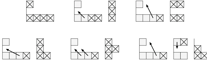
Fig. 6: The set \mathcal{G}(1, 0, 4) of all games on (1, 0, 4)
