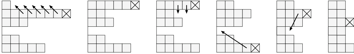
Fig. 5: A sequence of glissades in a game on (1,8,3,0,2,5)
