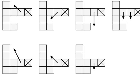
Fig. 4: All non-trivial glissades on (1,4,1,2) and (1,1,4,2) .
