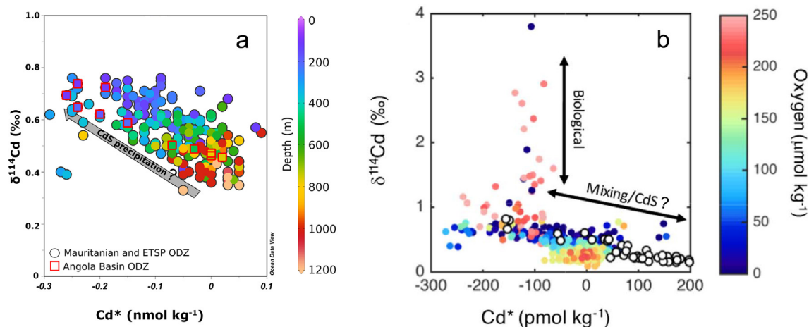
Fig. 2. Figures modified from (A) Guoinseau et al. (2019) showing tropical OMZ Cd*– \delta^{114}\text{Cd} correlations and (B) John et al. (2018) showing the similarity between the Peruvian OMZ Cd*– \delta^{114}\text{Cd} correlation (colours) and that in the Southern Ocean (white; data from Abouchami et al., 2011; Xue et al., 2013).
