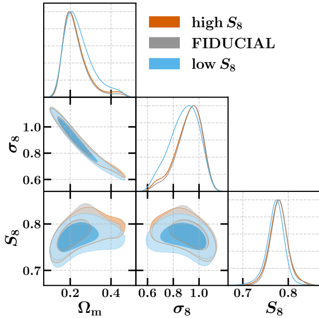
Figure H1. Comparison of the cosmological constraints obtained using peak counts. To illustrate the cosmology dependence of the marginalisation the polynomials in Equation 20 were fit using simulations at three different central cosmologies (low S_8 \sim 0.769 , fiducial S_8 \sim 0.782 and high S_8 \sim 0.815 ). The contour levels in both plots indicate the 68% and 95% confidence regions of the constraints.
