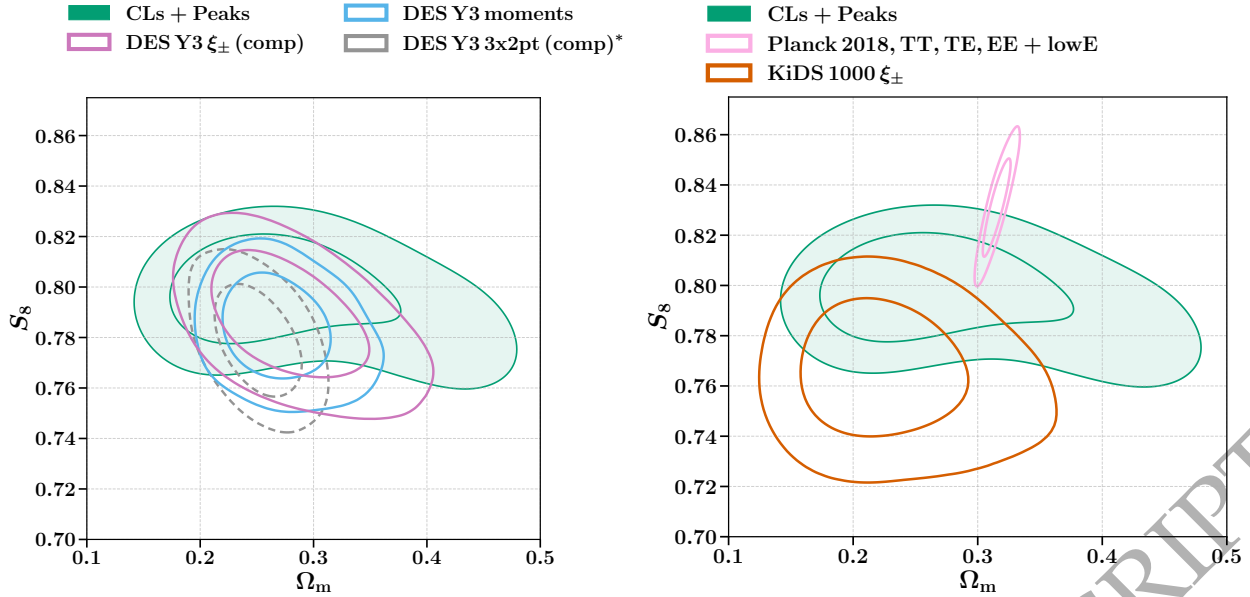
Figure 9. Left: A comparison between the fiducial \Omega_m - S_8 constraints inferred in this study using the combination of angular power spectra and peak counts (CLs + Peaks) and the results from other studies using DES Y3 data. The constraints labelled with ‘(comp)’ have been altered to enable a better comparison with our analysis (see Section 6.4). The DES Y3 3x2pt (comp) analysis does not pass the criteria defined in Dark Energy Survey Collaboration et al. (2021) and has been centered at the fiducial cosmology adapted in the simulations ( \Omega_m = 0.26 , \sigma_8 = 0.84 ) (see Section 6.4). Right: Another comparison between the fiducial \Omega_m - S_8 constraints inferred in this study using the combination of angular power spectra and peak counts (CLs + Peaks) and the results from external studies using data other than the DES Y3 data. The contour levels in both plots indicate the 68% and 95% confidence regions of the constraints.
