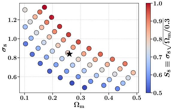
Figure 2. Distribution of the PKGRAV3 simulations in the \Omega_m - \sigma_8 plane. The remaining cosmological parameters were fixed to the ( \Lambda CDM, TT, TE, EE+lowE+lensing) results of Planck 2018 (Aghanim et al. 2020) in all simulations. Fifty simulations were run at the fiducial cosmology ( \Omega_m = 0.26 , \sigma_8 = 0.84 ); this cosmology is marked by the star. Five simulations were run at every other cosmology. The simulations are distributed around the fiducial cosmology along lines of approximately constant S_8 . The colour of the points indicates the value of the S_8 parameter.
