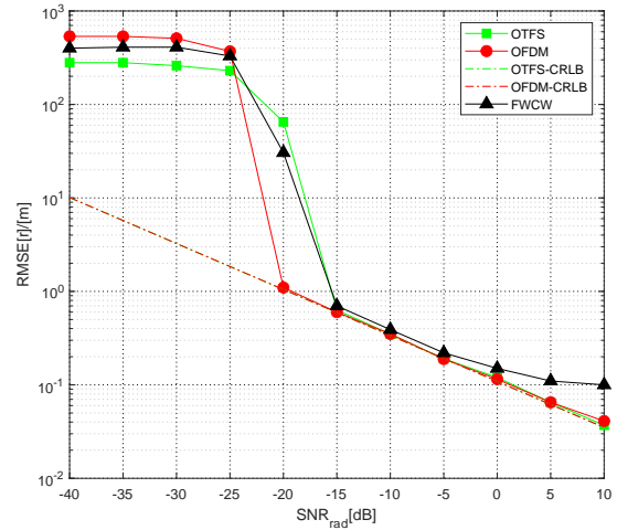
Fig. 37. Performance bound of OFDM and OTFS compared with FMCW.
