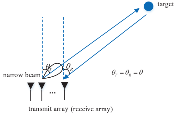
Fig. 21. Single-target sensing in the mono-static phased-array radar system.
