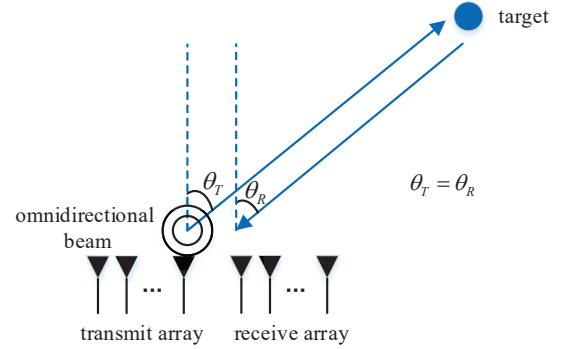
Fig. 22. Single-target sensing via colocated MIMO radar.
