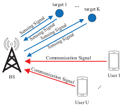
Fig. 12. Multiple access channel with mono-static BS sensing.
