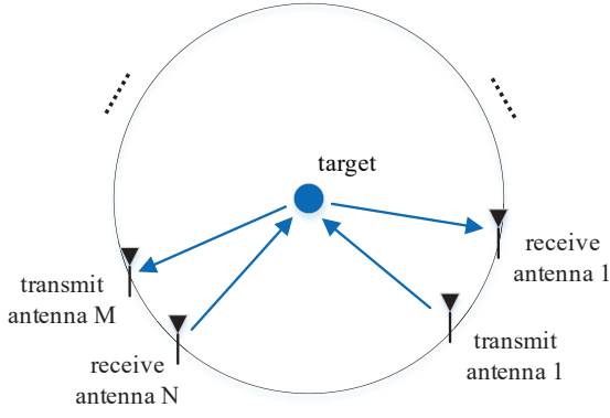
Fig. 24. Single-target sensing via distributed MIMO radar.
