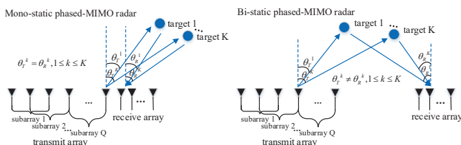
Fig. 8. Phased-MIMO radar.
