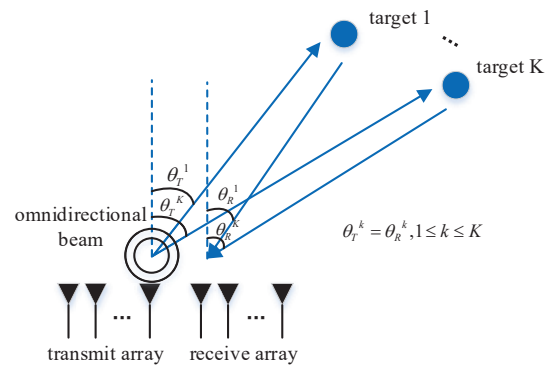
Fig. 6. An illustration of colocated MIMO radar.
