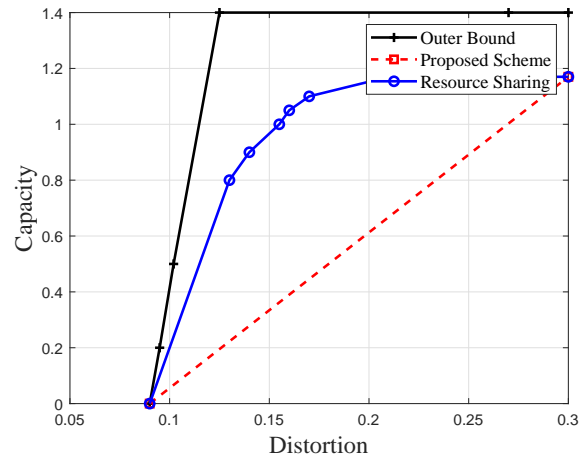
Fig. 32. Tradeoff between sum rate and distortion for p_s = 0.7 [19].
