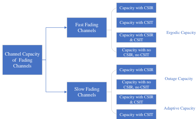
Fig. 20. An overview of performance metrics for fading channels.
