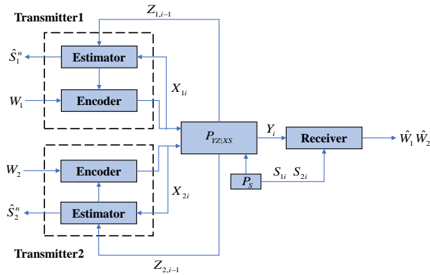
Fig. 31. The system model of multiple-access channel with mono-static sensing.
