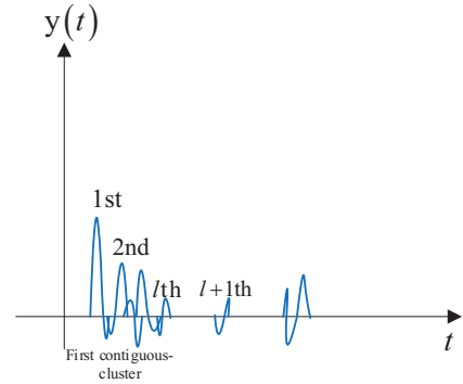
Fig. 27. An illustration of the first contiguous cluster (containing paths) in a LOS signal. The first contiguous cluster is defined to be the set of paths \{1, 2, \dots, l\} such that |\tau_i - \tau_{i+1}| < T_s for i = 1, 2, \dots, l-1 , and |\tau_l - \tau_{l+1}| > T_s where T_s is the duration of s(t) .
