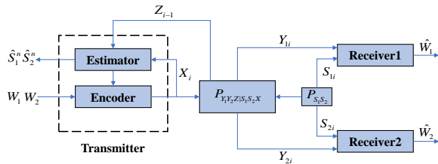
Fig. 33. The system model of broadcast channel with mono-static sensing.
