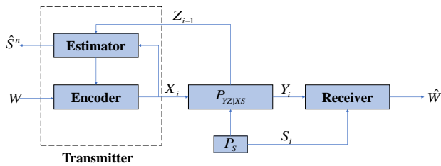
Fig. 29. The system model of point-to-point channel with mono-static sensing (generalized feedback).
