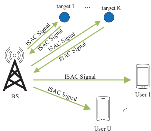
Fig. 14. Broadcast channel with mono-static BS sensing.
