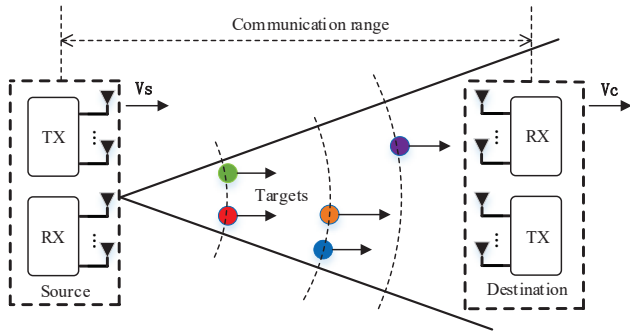
Fig. 36. A point-to-point communication system with mono-static sensing.
