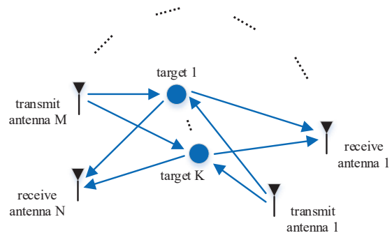
Fig. 7. An illustration of distributed MIMO radar.
