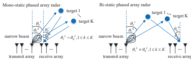
Fig. 5. An illustration of different classes of phased-array radar.
