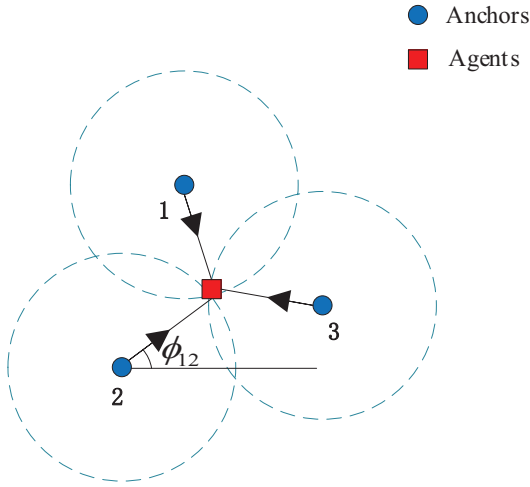
Fig. 26. An illustration of TOA-based localization.
