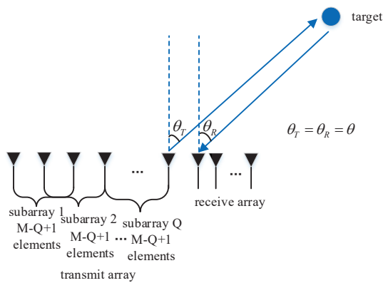
Fig. 25. Single-target sensing via phased-MIMO radar.
