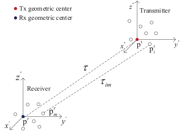
Fig. 28. Localization in a massive MIMO system [88].
