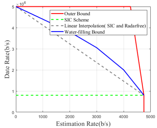
Fig. 35. The tradeoffs between communication information rate and estimation information rate under different schemes [103].
