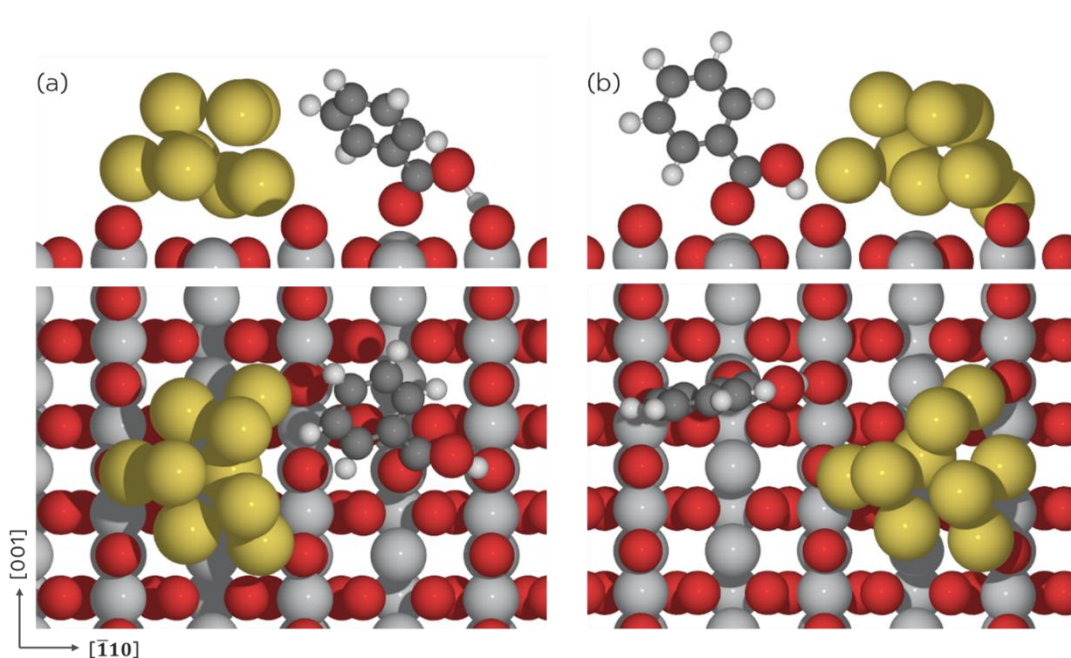
Figure 6. Side and top views of benzoic acid adsorption (with a coverage of ca. 0.07 ML) on (a) Au 9 / s -TiO 2 (110) and (b) Au 9 / r -TiO 2 (110). Colour code: carbon – dark grey; oxygen – red; hydrogen – white; titanium – grey; gold – yellow.
