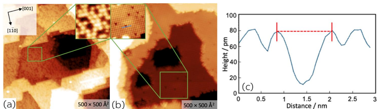
Figure 1. STM images of TiO 2 rutile (110) surface before and after exposure to 10 L benzoic acid: (a) large area image of clean rutile (110), ( V_s=+2.09 V, 0.03 nA). Inset of 50 \text{ \AA} \times 50 \text{ \AA} (see SI figure S3 for more details); (b) large area image of the near-pristine benzoate monolayer formed on the clean TiO 2 rutile (110); (+1.90 V, 0.03 nA). Inset of 100 \text{ \AA} \times 100 \text{ \AA} highlights the point (adsorbate) defect vacancies, seen as dark spots on the overlayer. This overlayer gives a coverage of 0.48 ML; and (c) line profile taken from the STM image, as depicted by the blue line in the inset of (b), across four benzoate molecules and a benzoate vacancy showing the (2 \times 1) spacing of 12 \text{ \AA} as measured by the red dotted line between two adjacent benzoate molecules, and an apparent height of the molecules of \sim 70 pm.
