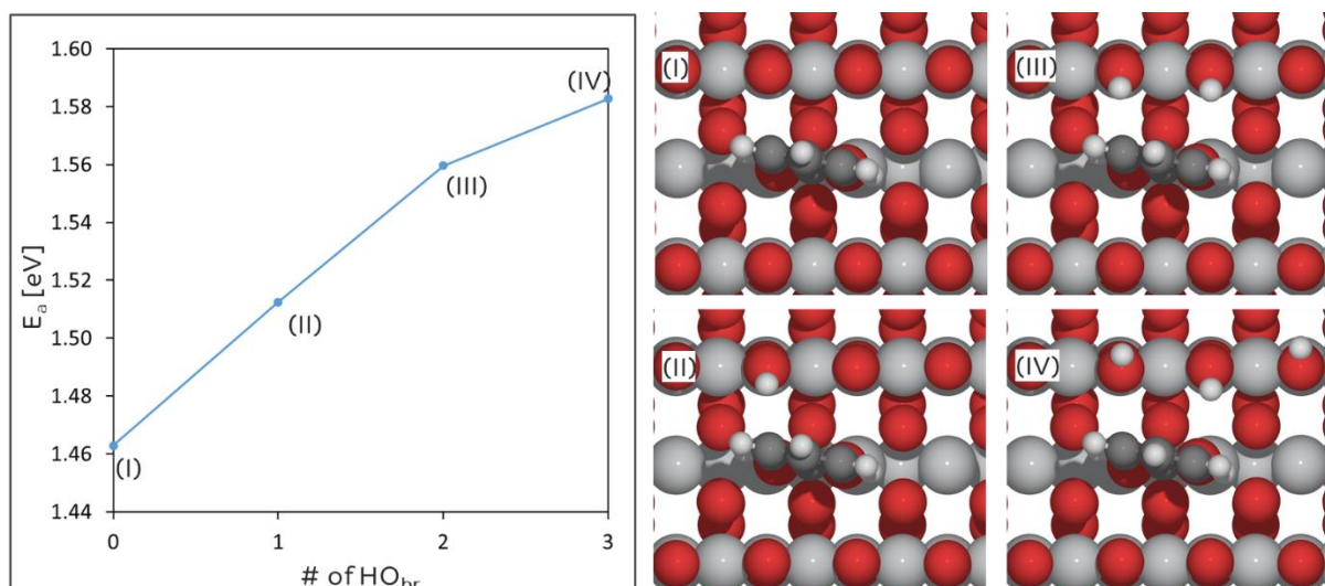
Figure 3. Calculated diffusion barriers for an isolated benzoate species along the [001] direction on the s -TiO 2 (110) surface with respect to the number of HO br . The roman numeral corresponds to each final state of benzoate diffusion: (I) benzoate on the TiO 2 (110), (II) benzoate on the HO br / s -TiO 2 (110), (III) benzoate on the 2HO br / s -TiO 2 (110), and (IV) benzoate on the 3HO br / s -TiO 2 (110). Colour code: carbon – dark grey; oxygen – red; hydrogen – white; titanium – grey.
