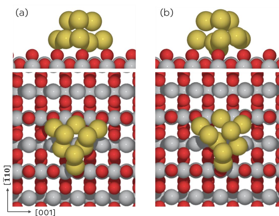
Figure 5. Top and side views of the relaxed \text{Au}_9 clusters on (a) s\text{-TiO}_2 and on (b) r\text{-TiO}_2 . Color code: oxygen – red; titanium – grey; and gold – yellow.
