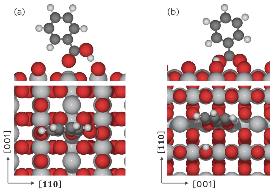
Figure 2. Side and top views of molecular (a) and dissociative (b) adsorption of benzoic acid over stoichiometric rutile TiO 2 (110). The surface coverage is around 0.06 ML. Colour code: carbon – dark grey; oxygen – red; hydrogen – white; titanium – grey.
