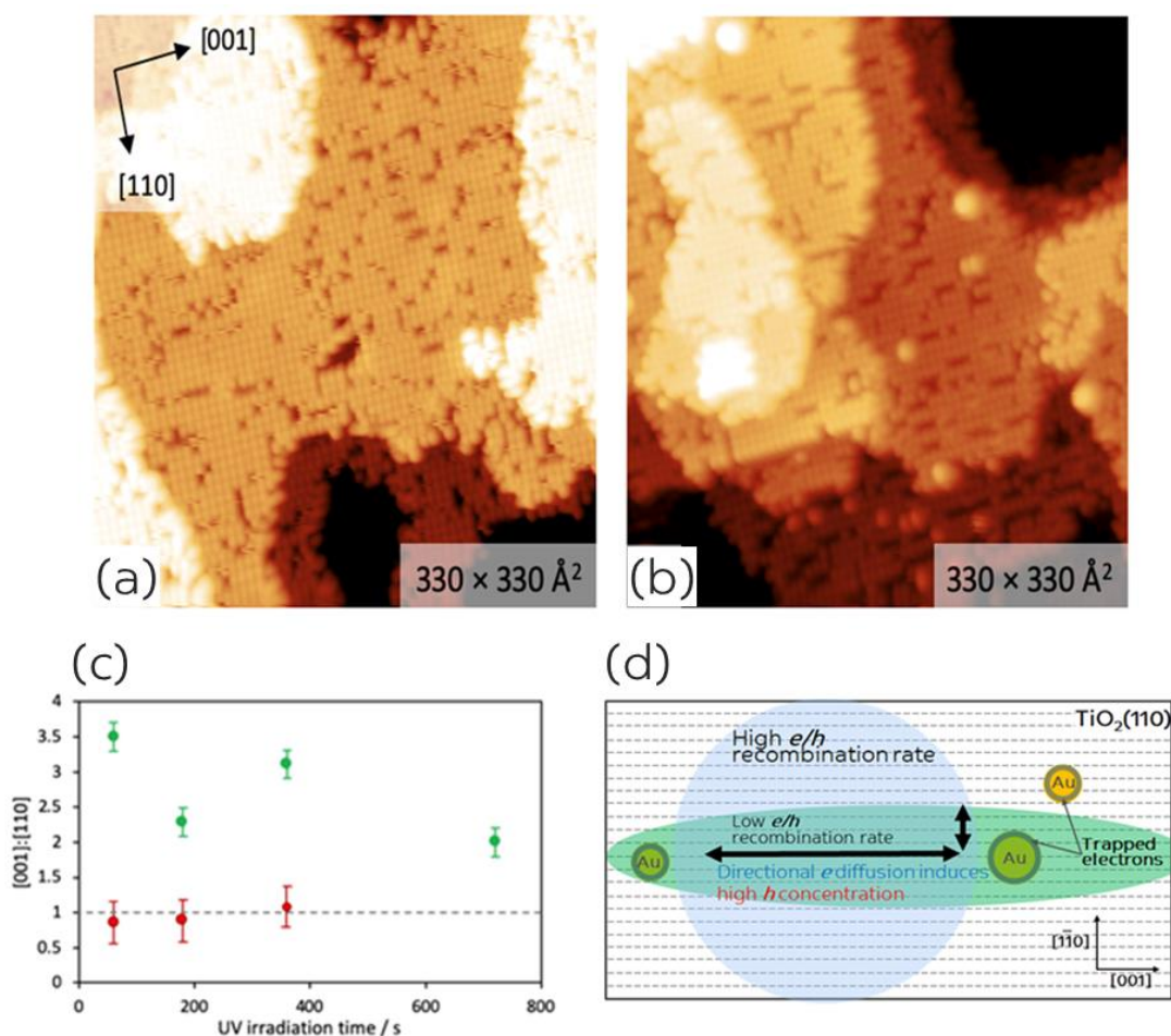
Figure 7. Images taken of benzoate overlayers (0.41 ML) following irradiation of TiO 2 (110) and Au/TiO 2 (110). (a) shows the bare benzoate covered (110) surface after three minutes of exposure to UV-Vis light and (b) shows the gold-doped surface after six minutes UV-Vis irradiation (both images are recorded at a tip voltage V_s = +2.0 V, I_t = 0.03 nA). The choice of different time is to compare “reaction selectivity” at a similar “coverage”. (c) is a scatter plot comparing the direction of ‘chains’ of empty benzoate sites at different irradiation times for the two surfaces, by recording the ratio of the number of chains along the [001] to those oriented along the [110]. There is a dotted line at [001]:[110] = 1, which indicates the value for an isotropic distribution. The values for the bare surface are plotted in red and the gold-loaded surface in green. (d) A schematic representation of the excited electronic state upon light excitation. The green area represents a high hole concentration area, because electrons are preferentially diffusing along [001] and are trapped at Au clusters. The blue area is a representation of a domain that does not contain Au clusters therefore will not have a preferential directional removal of benzoates. The length of black arrows represents the magnitude of electron conductivity along and perpendicular to the [001] direction. The dashed lines represent Ti cations on top of which benzoates are formed. To compute for the anisotropic reaction displayed in (c), we have counted each instance of two or more adjacent molecular vacancies as a ‘chain’, then compared the total number of chains in each direction, irrespective of length. Five images for each irradiation time were used from which the average ratio is taken.
