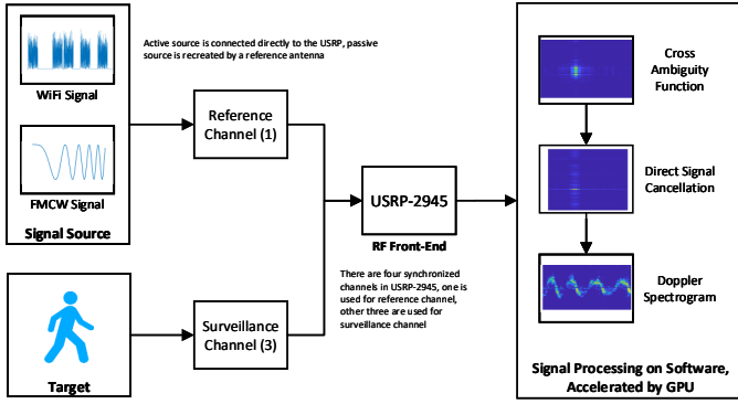
Fig. 1: Overview of proposed multichannel SDRadar system
