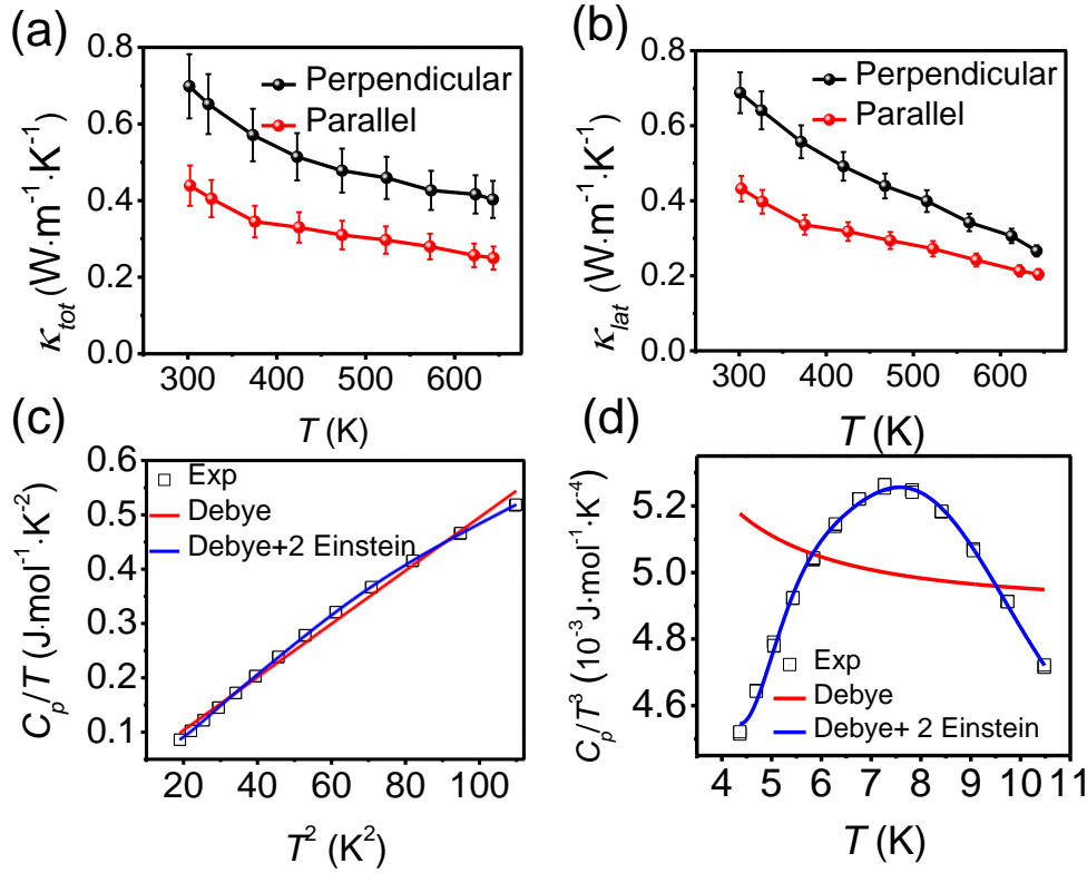
Figure 3. (a) Temperature dependence of total thermal conductivity for TiCuSe along two different directions (parallel and perpendicular to the pressing direction) and (b) temperature dependence of the lattice thermal conductivity in the two directions for TiCuSe. (c) C_p/T versus T^2 with fits shown using just the Debye model and a hybrid model combining both Debye and two Einstein vibrational modes. (d) C_p/T^3 versus T with fits shown using just the Debye model and a model incorporating both Debye and two Einstein vibrational modes.
