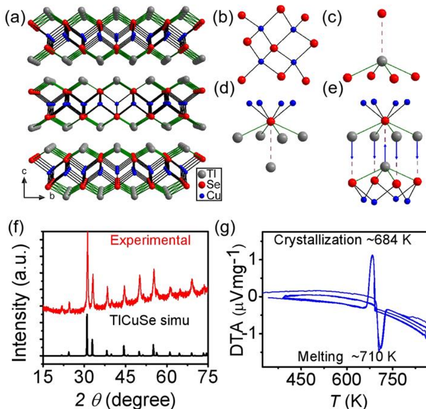
Figure 1. (a) Crystal structure of \text{TlCuSe} viewed along the a axis, (b) Antifluorite-type [\text{CuSe}]^- layers, (c) Coordination environment of the Tl atom, (d) Coordination environment of the Se atom, (e) Interlayer
