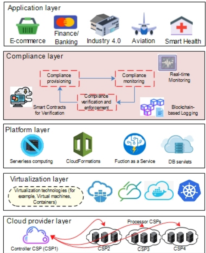
Fig. 1: Compliance-aware multi-layered service stack for Cloud services
