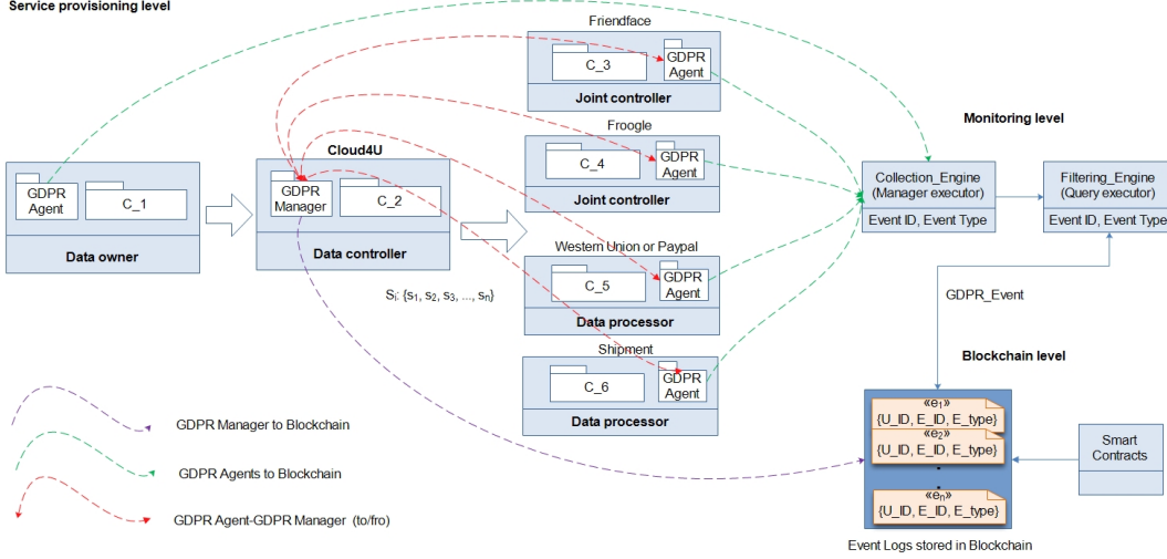
Fig. 4: Component interaction – showing how a GDPR agent can be deployed for each cloud service provider
