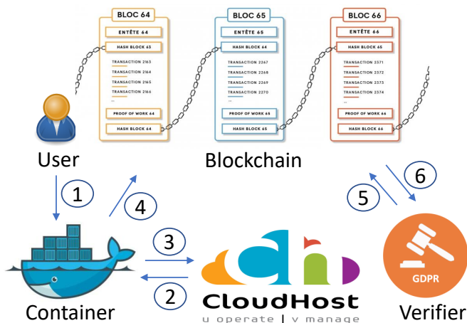
Fig. 3: Data flow in GDPR-compliance architecture
