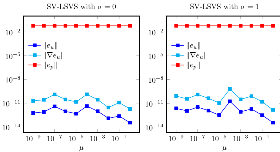
FIG. 4. Example 1: error plots of different norms versus the viscosity parameter \mu for Scott–Vogelius finite element method with LSVS stabilization on refinement level 2 ( \sigma = 0 left and \sigma = 1 right).
