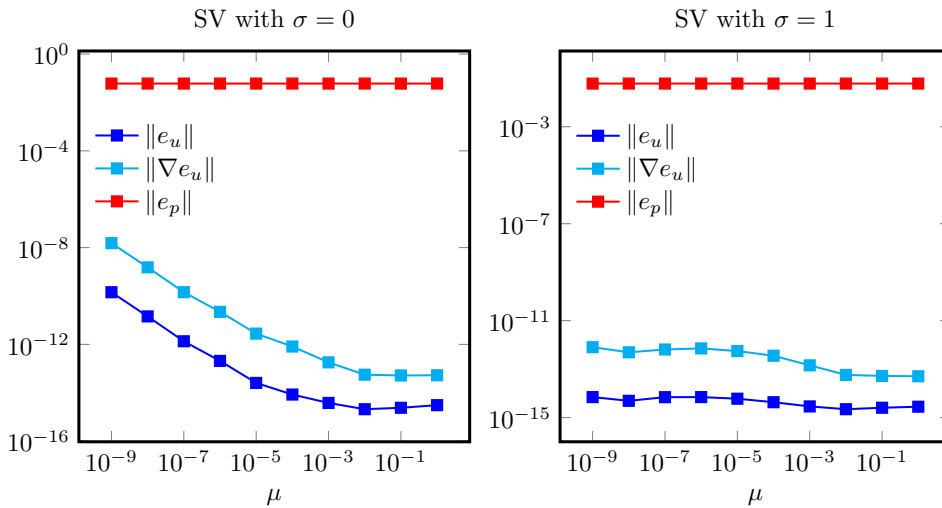
FIG. 2. Example 1: error plots of different norms versus the viscosity parameter \mu for Scott-Vogelius finite element methods on refinement level 2 ( \sigma = 0 left and \sigma = 1 right).
