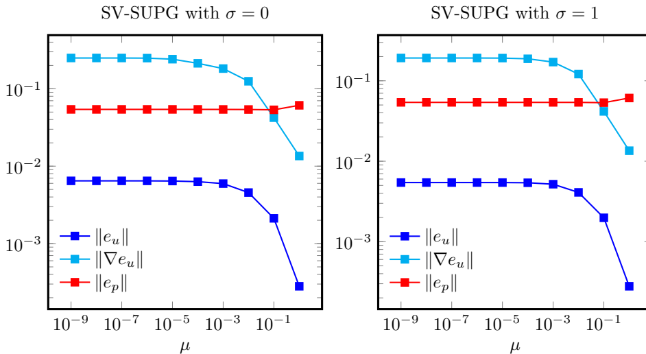
FIG. 3. Example 1: error plots of different norms versus the viscosity parameter \mu for Scott–Vogelius element with SUPG stabilization on refinement level 2 ( \sigma = 0 left and \sigma = 1 right).
