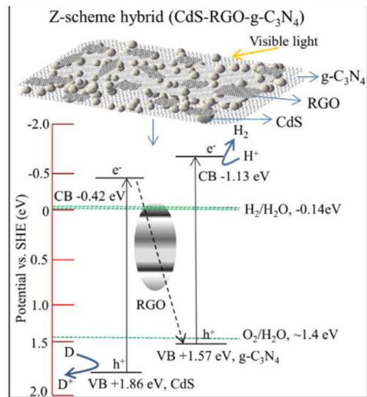
Figure 15. Z-scheme electron transfer mechanism; a) Schematic illustration of charge transfer mechanism in CdS-rGO-g-C 3 N 4 . Reproduced with permission from ref. [160] .
