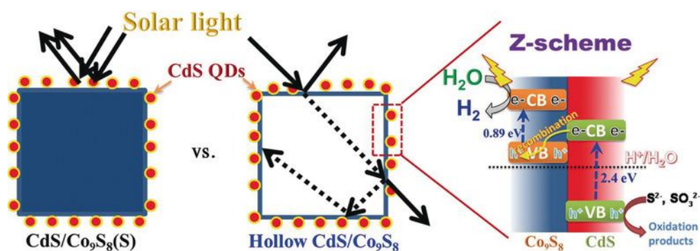
Figure 16. Systematic Illustration of multiple reflections within the \text{CdS}/\text{Co}_9\text{S}_8 hollow structure and the photoexcited charge-carrier distribution. Reprinted with permission from ref. [167].
