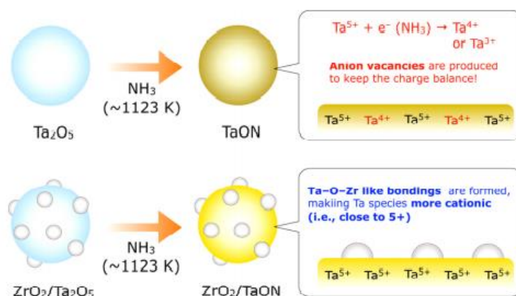
Figure 7. Synthetic protocol; \text{ZrO}_2/\text{TaON} synthesis through Nitridation of \text{ZrO}_2/\text{Ta}_2\text{O}_5 , a method of reducing the creation of tantalum species (reduced) near the surface. Reprinted with permission from ref. [109].
