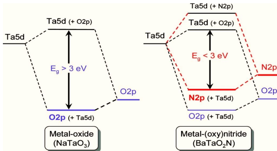
Figure 4. Schematic illustration of the band structure of metal oxide ( \text{NaTaO}_3 ) and metal (oxy)nitride ( \text{BaTaO}_2\text{N} ). Reproduced with permission from ref. [101].
