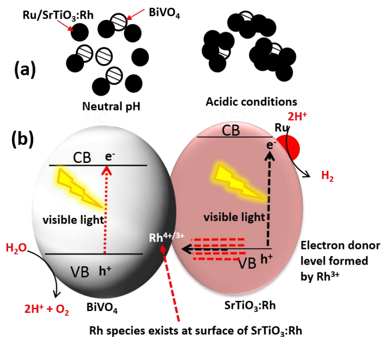
Figure 3. Schematic illustration of Z-scheme photocatalysis a) Suspension of Ru/SrTiO 3 :Rh and BiVO 4 at neutral and acidic conditions and b) Scheme of photocatalytic water splitting. Reproduced with permission from ref. [41].
