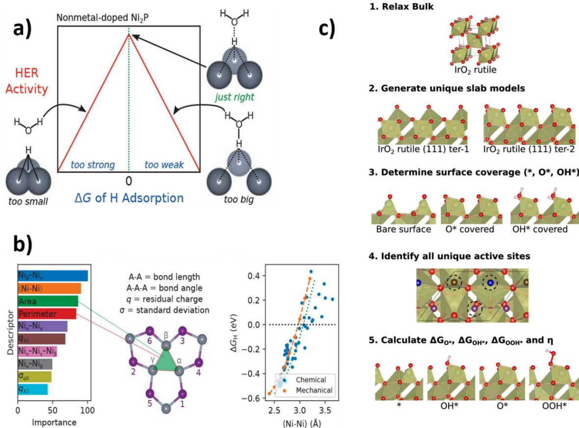
Figure 25. Machine learning; a) Effect of surface non-metal doping on the HER activity over Ni 3 P 2 termination of Ni 2 P(0001), b) Relative importance of descriptors calculated from RRF model. Only the top 10 features which definition of descriptors is shown in the inset. The three Ni atoms \alpha , \beta , and \gamma are labelled based on their distance from the first doping site. The Effect of average Ni–Ni bond length on \Delta G_H as induced by chemical pressure and mechanical pressure. Green dotted line adjusts for Ni–Ni bond contraction upon H adsorption in the mechanical case, and c) Workflow and atomic structure examples associated with each step to
