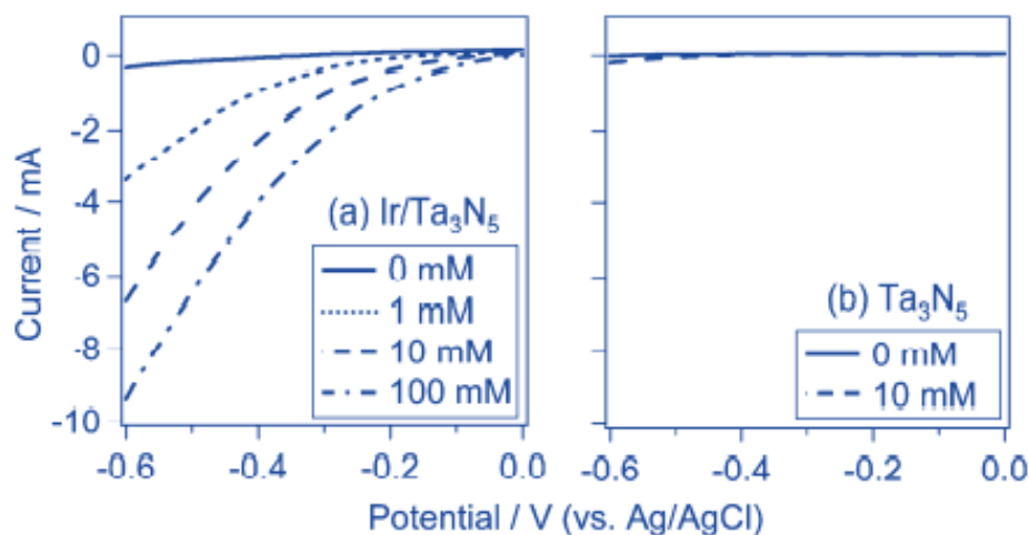
Figure 8. Comparison of currently produced from water splitting process by using \text{Ta}_3\text{N}_5 and Ir- \text{Ta}_3\text{N}_5 as electrode materials. Reprinted with permission from ref. [64].
