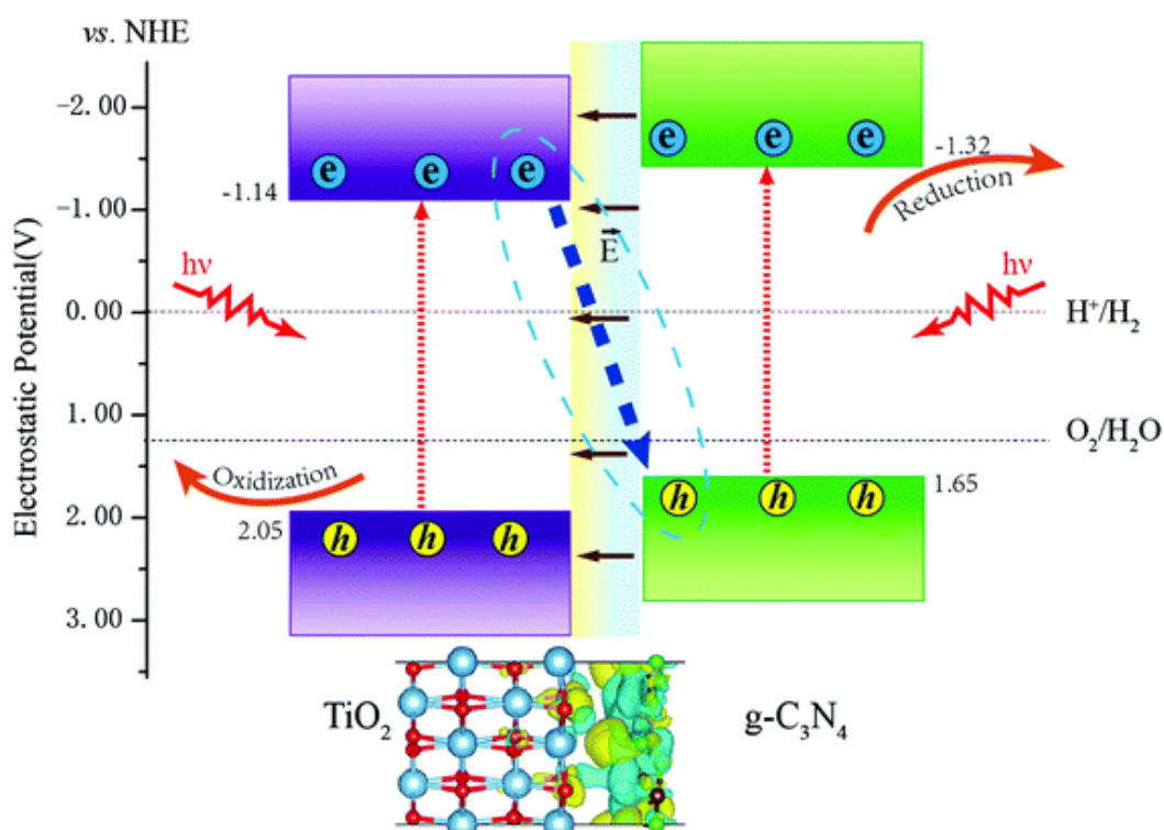
Figure 24. Proposed direct Z-scheme photocatalytic mechanism for the g-C 3 N 4 /TiO 2 heterostructure. Reprinted with permission from ref. [199].
