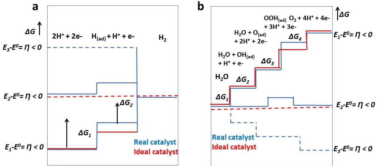
Figure 21. Plots of Gibbs free energies of reactive species and the chemisorptions of intermediates (horizontal lines) versus the reaction coordinate of (a) the HER and (b) OER. Blue lines and red lines indicate energetics of a typical (real) catalyst and ideal catalyst at three different electrode potentials ( E_1 , E_2 , E_3 ), respectively. Dashed lines indicate energetics at the electrode potential at which all thermochemical barriers disappear. \Delta G notes the free reaction energy of the two elementary reaction steps. The red case corresponds to an overpotential-free catalyst. E^0 denotes the standard reversible electrode potential of the HER, \eta is the overpotential. Reproduced with permission from ref. [227].
