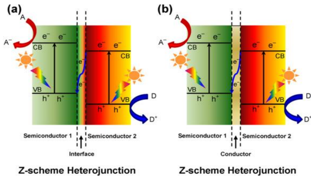
Figure 10. Systematic representation of two g-C 3 N 4 -based Z-scheme mechanisms. Reprinted with permission from ref. [122].
