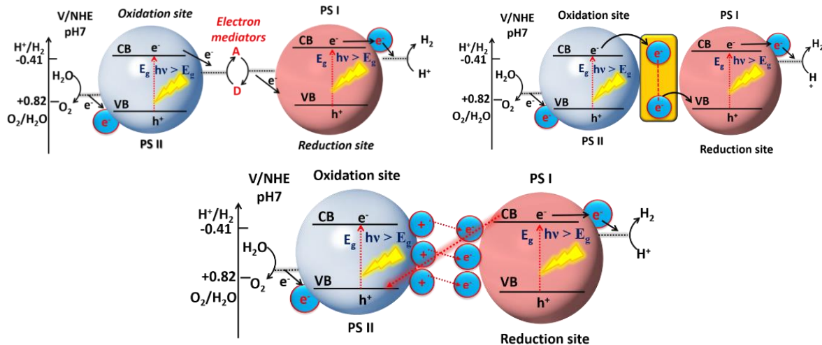
Figure 1. The schematic illustration of the band energy diagram of (a) PS-A/D-PS Z-scheme system (b) PS-C-PS Z-scheme system (c) PS-PS or direct Z-scheme system [1, 34, 39, 41, 42] .
