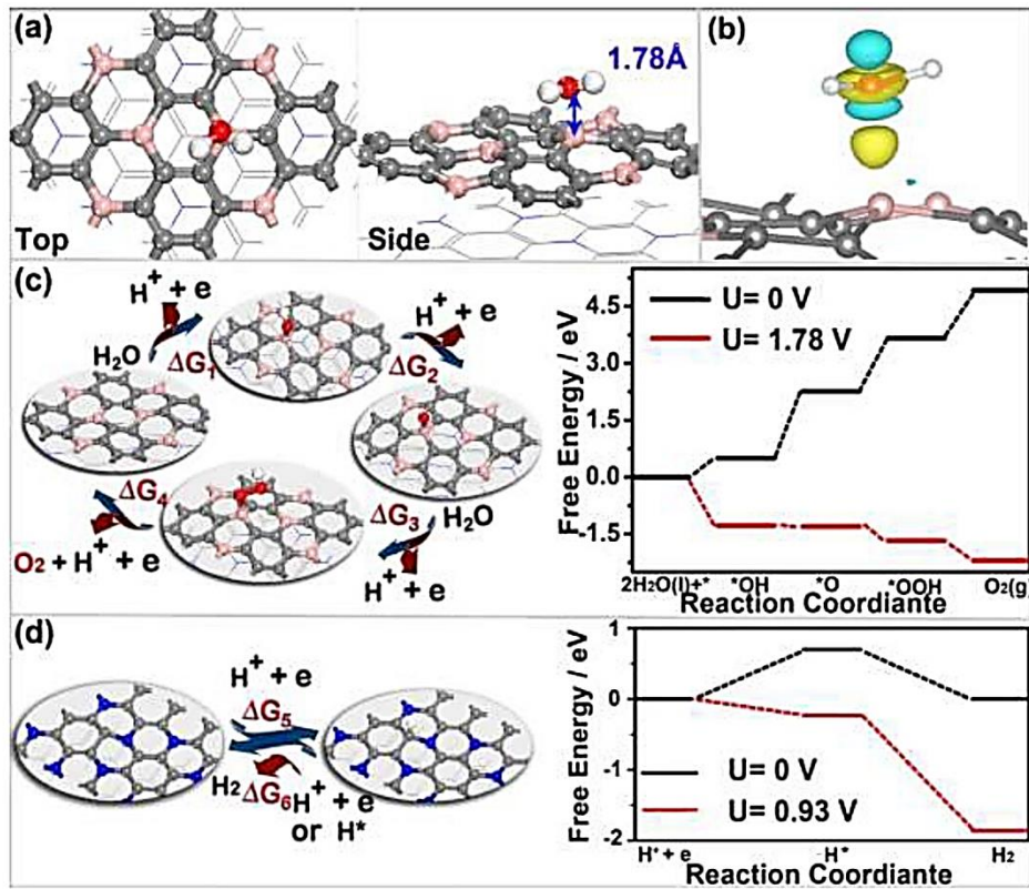
Figure 22. (a) Water adsorption on the C_3B sublayer of C_3N/C_3B heterostructure from the top and side views. (b) the charge density difference with the iso value is 0.008 e/\text{Bohr}^3 ; blue and yellow regions represent the e depletion and accumulation, respectively. (c) the reaction steps of water dissociations and free energy diagram denoted water oxidation (four-electron process) and hydrogen reduction (two-electron process) (d) the adsorption states of each species such as *OH , H^* , *O , and *OOH with the corresponding reactions. The photogenerated electron/ provide external potentials U = 1.78 ( 0.93 ) V for water oxidation (hydrogen reduction) reaction. Reprinted with permission from ref. [206].
