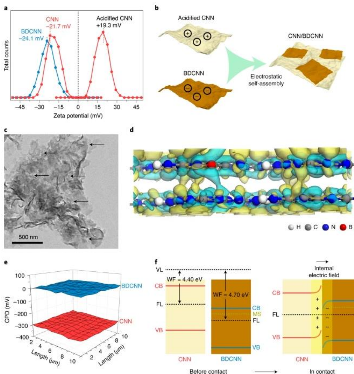
Figure 11. Construction of Z-scheme heterostructures, a) Zeta potential of the BDCNN, CNN, and acidified CNN dispersed in deionized water at pH 7, b) Schematic of the synthesis of the CNN/BDCNN heterostructure, c) TEM image of CNN/BDCNN. The arrows indicate the overlapped interfaces. d) Side-view differential charge density map of CNN and BDCNN. The iso-surface value is 0.012 e \text{ \AA}^{-3} . The yellow and blue regions represent net electron accumulation and depletion, respectively, e) Contact potential differences of CNN and BDCNN relative to a gold reference, f) The energy band offsets diagram and interfacial charge properties for the CNN/BDCNN heterostructure. VL, vacuum level; FL, Fermi level. Reprinted with permission from reference [131] .
