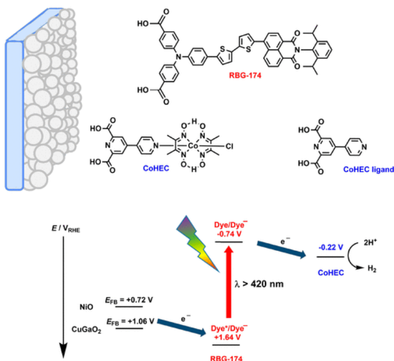
Figure 5. Photocathode illustration; the molecular structures and energy diagram. CoHEC redox potential is the onset of catalysis at pH 7. Electrochemical potentials are given vs RHE, flat band position of NiO corrected from V vs NHE (pH 7), and flat band position of CuGaO 2 corrected from V vs Ag/AgCl (pH 6.6) [104-106] . Reprinted with permission from ref. [104] .
