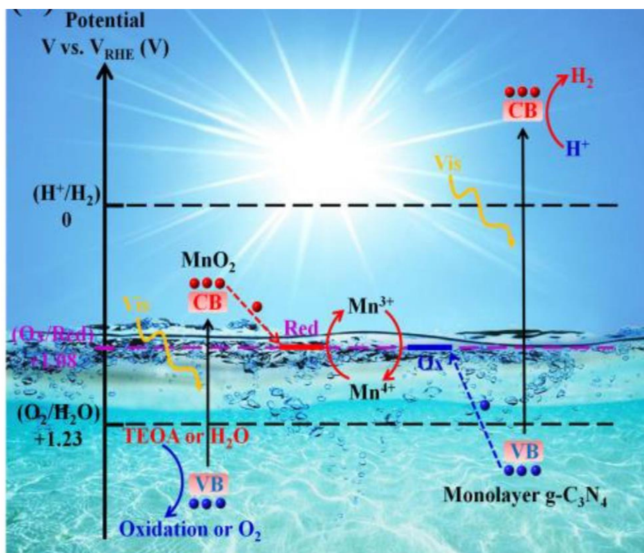
Figure 12. Z-Scheme charge transfer mechanism diagram of MnO 2 /Monolayer g-C 3 N 4 . Reprinted with permission from ref. [90].
