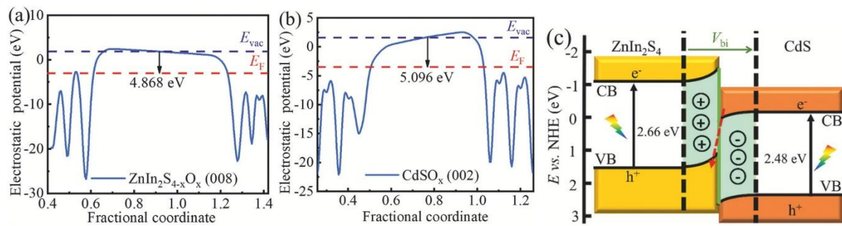
Figure 18. (a) Electrostatic potential illustration computed through DFT for \text{ZnIn}_2\text{S}_{4-x}\text{O}_x (008) surface and (b) \text{CdSO}_x (002) surface, and (c) the charge carrier migration schematic illustration in Z-scheme \text{ZnIn}_2\text{S}_4/\text{CdS} heterojunction. Reprinted with permission from ref. [201].
