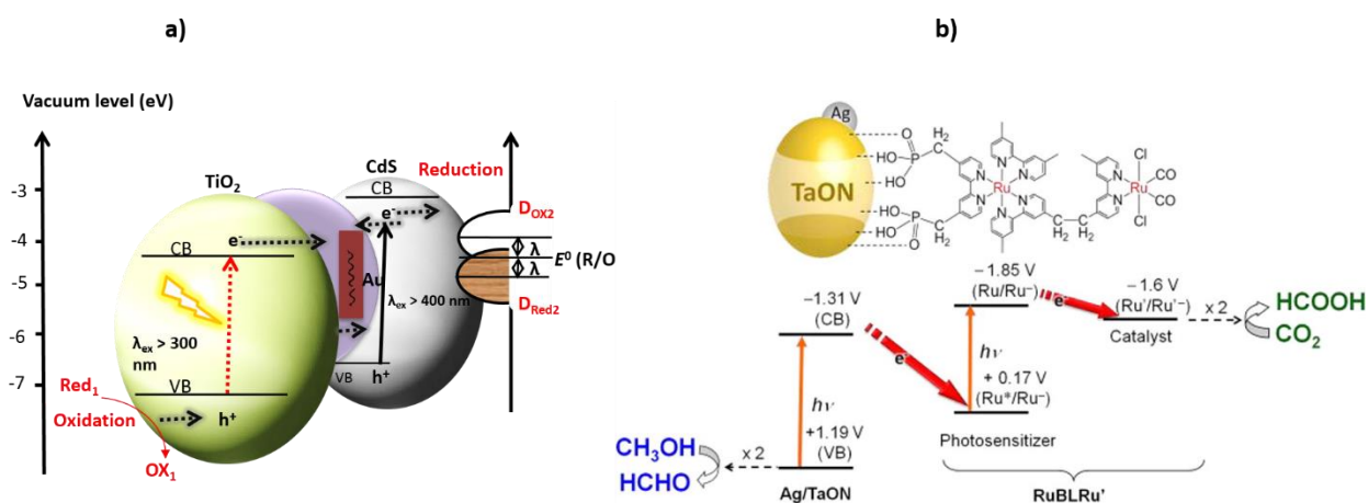
Figure 17. a) The band alignment illustration of CdS–Au–TiO 2 Z-system where the standard electrode potential of MV + /MV 2+ is represented by E^0 (R/O) while the occupied and unoccupied states are denoted as D_{Red2} and D_{Ox2} , respectively. Reproduced with permission from ref. [171], and b) Artificial Z-scheme for the catalysis of CO 2 and methanol. Reprinted with permission from ref. [175].
