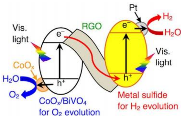
Figure 9. rGO induced Z-scheme water splitting by using CoO-loaded BiVO 4 as OEC and metals sulfides as HEC in the presence of Pt. Reprinted with permission from ref. [117] .
