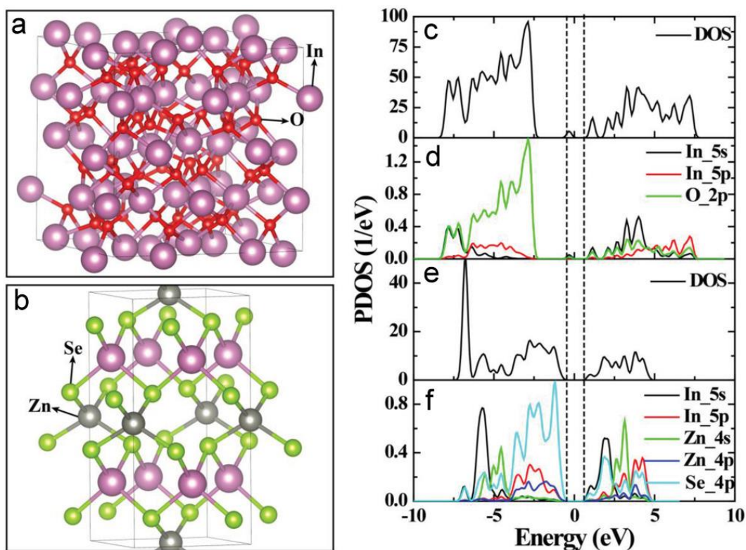
Figure 20. a,b) Optimized geometry structures of (a) \text{In}_2\text{O}_3 and (b) \text{ZnIn}_2\text{Se}_4 , and c–f) the corresponding density of state (DOS) plots. The dashed line represents the Fermi level. All electronic states were normalized by the deep In 4d states. Reprinted with permission from ref. [211].
