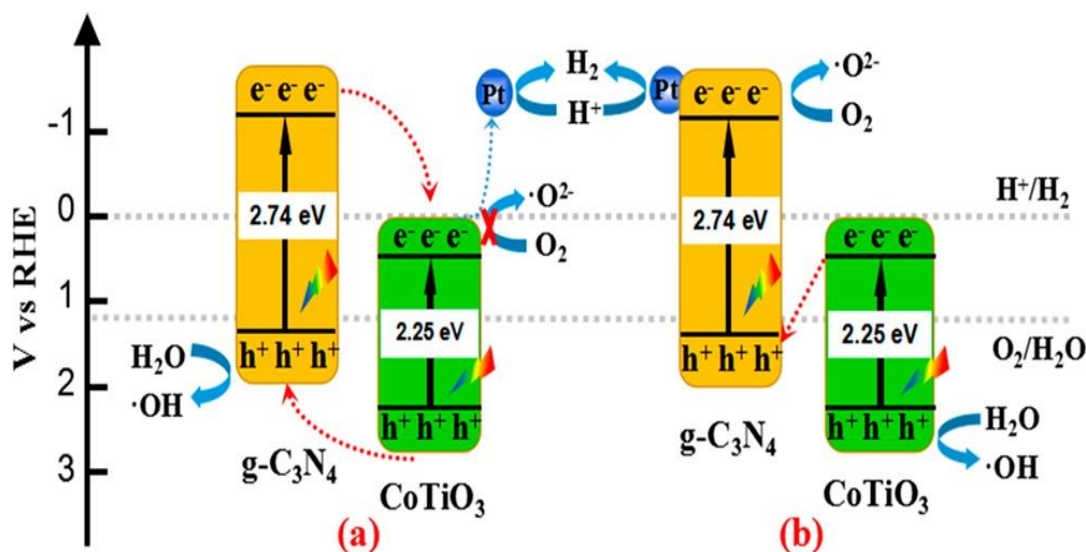
Figure 13. Schematic illustration for charge separation by traditional heterojunction-type (a) and direct Z-scheme (b) mechanisms. Reprinted with permission from ref. [126] .
