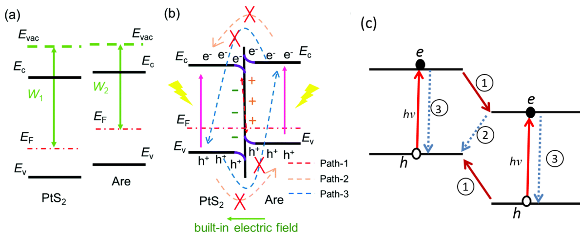
Figure 19. Schematic illustration of direct Z-scheme PtS 2 /Are vdW heterostructure: (a) before contact, (b) photoinduced charge carrier illustration after contact Reprinted with permission from ref. [188], and (c) Schematic diagram of photoexcitation and charge transfer dynamics 1) between heterostructure, 2) interlayer e–h recombination, and 3) intralayer e–h recombination. Reproduced with permission from ref. [40].
