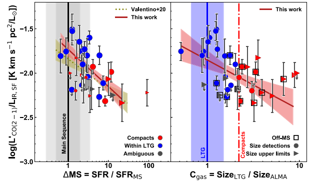
Figure 9. L'_{\text{CO}(2-1)} / L_{\text{IR, SF}} [ \text{K km s}^{-1} \text{pc}^2 / L_{\odot} ] as a function of the main sequence offset (left-hand panel) and the compactness (right-hand panel). The green dotted line and shaded area in the left-hand panel represent the best-fitting model and 1\sigma confidence interval from Valentino et al. (2020). The dark red solid line and shaded area in the left-hand panel indicate the L'_{\text{CO}(2-1)} / L_{\text{IR, SF}} - \Delta\text{MS} trend and 1\sigma confidence interval obtained after excluding compact and ambiguous main sequence galaxies from the fit. The dark red solid line and shaded area in the right-hand panel mark the best-fitting model and 1\sigma confidence interval of the L'_{\text{CO}(2-1)} / L_{\text{IR, SF}} - C_{\text{gas}} trend. The colour-code and symbols are analogous to Fig. 3. We measure the uncertainty on the L'_{\text{CO}(2-1)} / L_{\text{IR, SF}} ratio by propagating the 1\sigma errors on the CO(2-1) flux measurements and on L_{\text{IR, SF}} .
