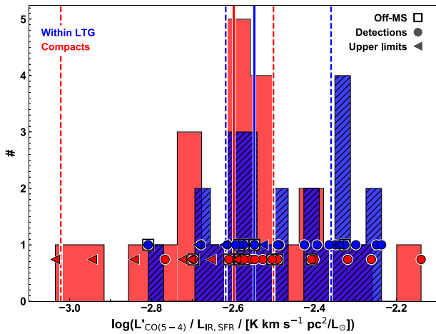
Figure 18. Distribution of the L'_{\text{CO}(5-4)}/L_{\text{IR,SFR}} logarithmic ratio for submillimetre compact (red) and extended (hatched blue) galaxies in our sample. The solid and dashed lines indicate the median and interquartile range of each distribution, respectively. The \log(L'_{\text{CO}(5-4)}/L_{\text{IR,SFR}}) measurements and upper limits are highlighted with circles and triangles, respectively. The open black squares indicate galaxies above the main sequence, with \Delta\text{MS} \geq 3.5 .
