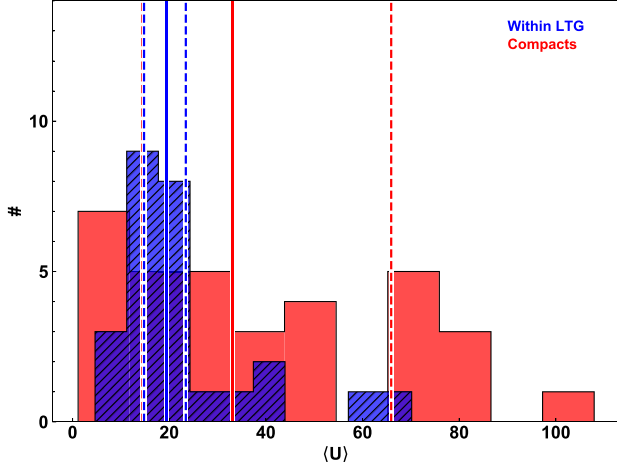
Figure 12. Distribution of the intensity of the radiation field for compact (red) and extended (hatched blue) galaxies in our sample. The solid lines indicate the median of each distribution. The dashed lines represent the interquartile ranges.
