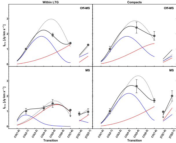
Figure 7. LVG fit to the observed CO + [CI] SLEDs for extended (left-hand panel) and compact (right-hand panel) galaxies in our sample, split according to their main sequence position as in Fig. 5. Colour code is analogous to Fig. 6.
