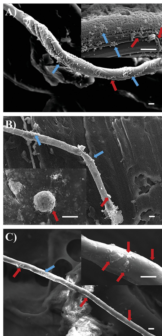
FIG. 9. SEM images of wound dressing samples after cell viability (indicated with red arrows) and bacterial colony counts (indicated with blue arrows) following co-culture. (a) Control material (bacterial cellulose–PMMA), (b) bacterial cellulose–PMMA–1 wt.% combination of Cu–Ag–Zn/CuO NPs (UHNP)-1, and (c) bacterial cellulose–PMMA–1 wt.% combination of Cu–Ag–Tungsten carbide NPs (AVNP)-2. (Scale bars indicate 10 \mu m). Reprinted from E. Altun et al. , Macromol. Mater. Eng. 304 , 1800537 (2019). Under a CC BY License, Copyright 2018, the Author(s). 133
