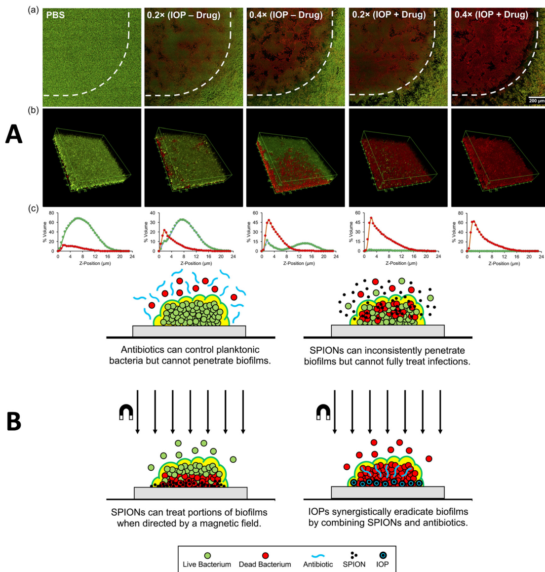
FIG. 5. Anti-biofilm activity of SPIONs-methicillin/PEG- b -PLA copolymer against S. epidermidis . (a) LIVE/DEAD staining of biofilms treated with different dilutions of IOPs (1× stock = 100 μg/mL SPION; 50 μg/mL methicillin) for 24h. (a) Tile scans collected halfway through the biofilm show concentration-dependent bacteria death within the boundary of the external applied magnetic field (dashed line). (b) 3D reconstructions of z-stacks collected across the biofilm thickness inside the magnetic field. (c) The percentage of biofilm volume occupied by live and dead bacteria as a function of biofilm depth (0 μm = bottom) as quantified from image slices. Viable and dead cells appeared green and red, respectively. 99 (B) Current mechanisms for biofilm treatment using the ternary system. Reprinted with permission from Geilich et al. , Biomaterials 119 , 78 (2017), Copyright 2017, Elsevier.
