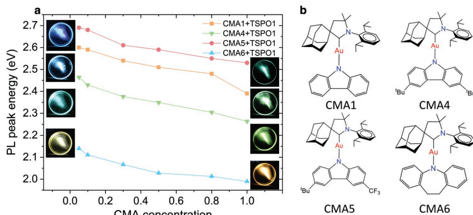
Figure 6. a) Dependence of PL peak energy of various CMA on the doping concentration in TSPO1 host. Photographs show photoluminescence of neat CMA1, CMA4, CMA5, and CMA6 and 5% weight concentration of CMA in TSPO1 thin films under UV illumination. b) Chemical structures of CMA1, CMA4, CMA5, and CMA6.
