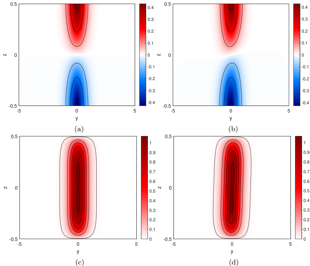
Figure 6: Comparison between the TTW and modified TTW solutions for E = 0.01 and T = 1 . Solutions are shown correct to O(\delta) . (a) b'/(Ro Pr) for \delta = 0 , (b) b'/(Ro Pr) for \delta = 0.4 , (c) N^2/(Ro Pr) for \delta = 0 , and (d) N^2/(Ro Pr) for \delta = 0.4 .
