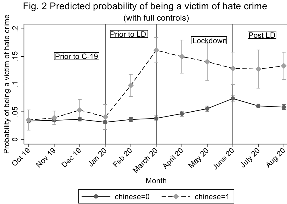
Figure 2. Predicted probability of being a victim of hate crime for Chinese people and others after before during and after the UK national lockdown
