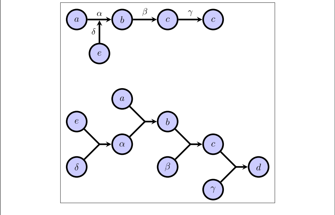
Figure 9: (Top) A HLAFA with a higher-order attacks, where Greek letters denote the labels of the attacks; and (Bottom) its corresponding frame with joint attacks
