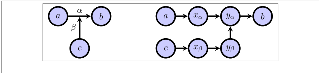
Figure 7: (LHS) HLAFA with attacks \alpha = (a, b) and \beta = (c, \alpha) ; and (RHS) the translation into a series of AF attacks
