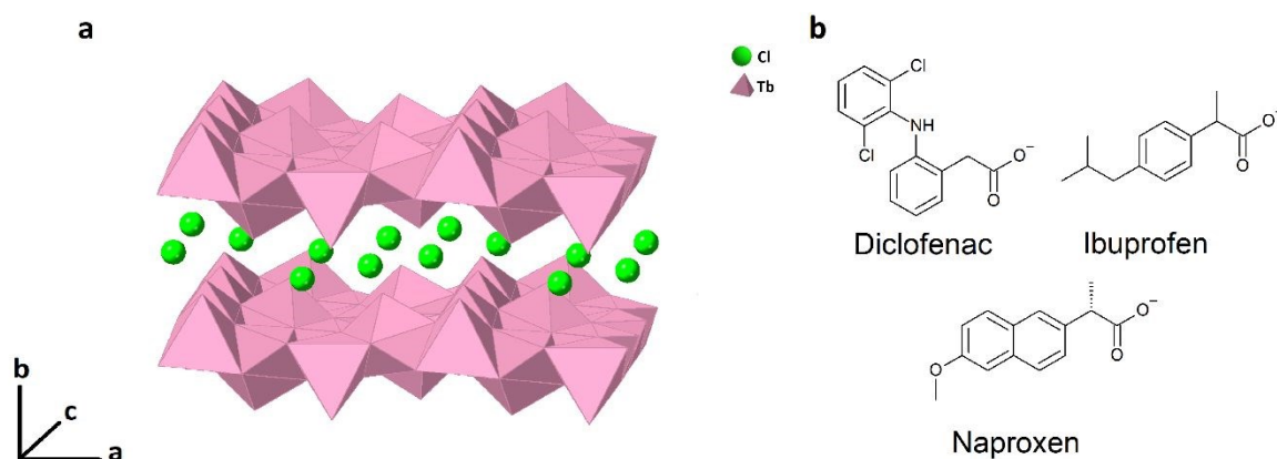
Figure 1 a.) A schematic diagram showing the lamellar structure of LTbH with intercalated Cl - anions. b.) The chemical structures of the anions of diclofenac, ibuprofen, and naproxen.
