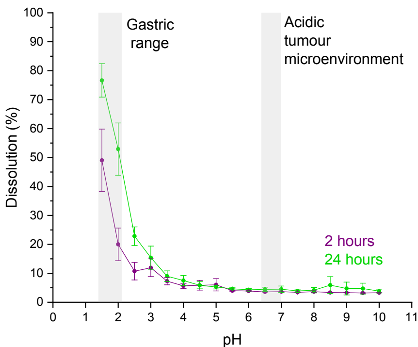
Figure 8 pH stability assay of LTbH-Cl in aqueous suspension, after 2 and 24 hours. Three independent experiments were performed, each in triplicate, and the results are shown as mean \pm standard deviation.
