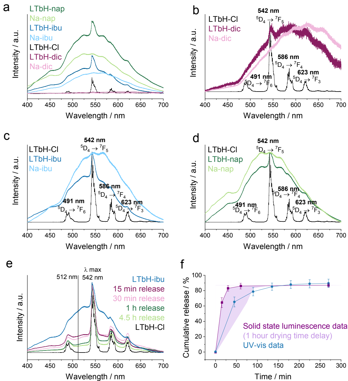
Figure 10 Solid state photoluminescence emission spectra of LTbH-Cl, LTbH-drug intercalates, and the pure drug salts (Na-dic, Na-ibu, Na-nap) obtained by solid state photoluminescence at an excitation wavelength of 325 nm and laser power of 1 %. a.) Raw data, b-d.) Normalised data. e.) Normalised solid state photoluminescence emission spectra of LTbH-ibu (pure) and LTbH-ibu at different stages of release (15 min, 30 min, 1 h, and 4.5 h) as compared to LTbH-Cl. f.) Drug release curve obtained from photoluminescence compared to the drug release curve obtained by UV-vis. Results presented as mean \pm standard deviation.
