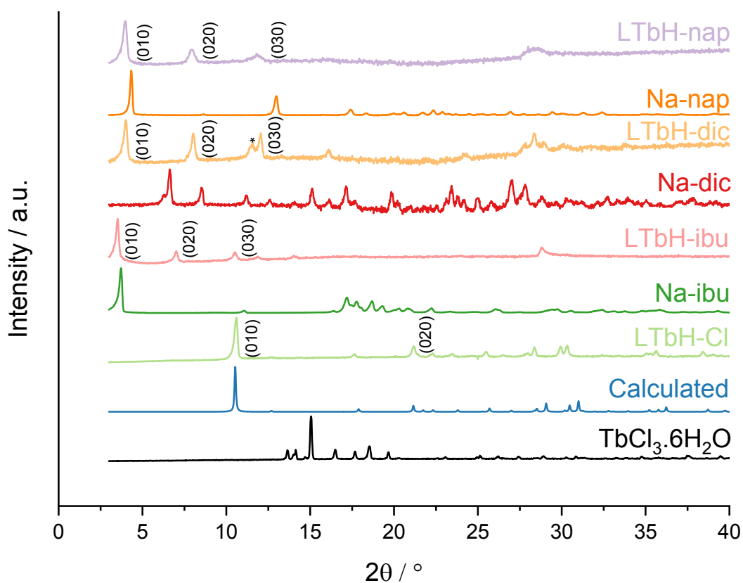
Figure 3 XRD patterns for starting materials and intercalation compounds of LTbH prepared by ion exchange. *: The (030) reflection of LTbH-dic is seen to partially overlap with the (011) reflection. Calculated pattern based on LYbH-Cl (ICSD collection code 419745).
