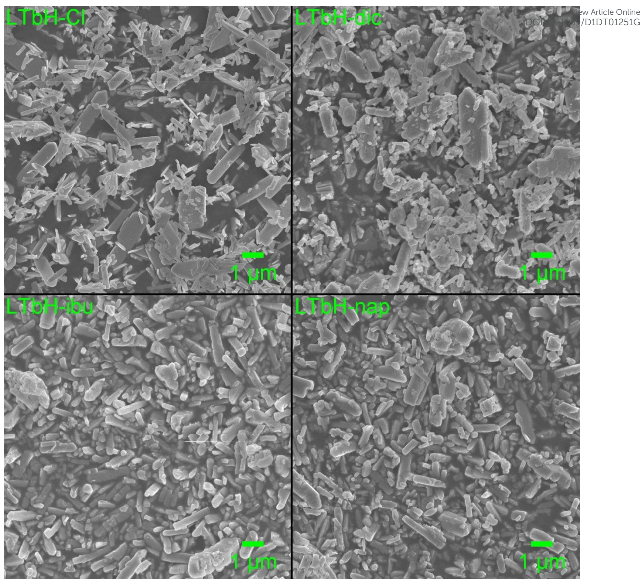
Figure 2 SEM images of the LTbH-Cl and LTbH-drug intercalates.
