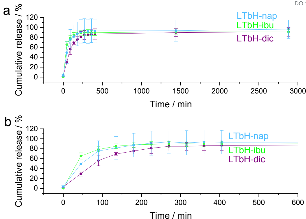
Figure 9 Drug release curves for LTbH-dic, LTbH-ibu, and LTbH-nap in phosphate buffered saline (PBS, pH = 7.4) a.) over 48 h and b.) an enlarged view of the first 10 h. Results are presented as mean \pm standard deviation.
