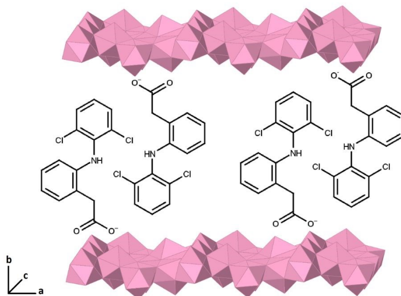
Figure 4 Schematic diagram illustrating the bilayer arrangement of intercalated diclofenac within the LTbH interlayer gallery.
