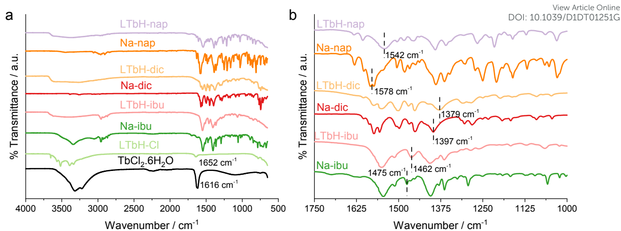
Figure 5 a.) FTIR spectra for starting materials and the intercalation compounds of LTbH prepared by ion exchange. b.) Enlarged view showing band shifting in LTbH-drug intercalate spectra relative to the pure drug spectra.
