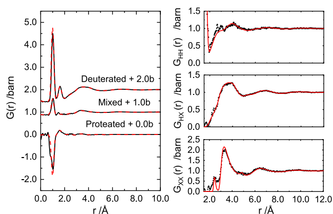
Figure 2. Left: Real space function G(r) for isotopically unique 4 MPM Ca–NH 3 samples. Data are offset by a given amount for clarity. From top to bottom: deuterated, mixed, and proteated. Right: Partial pair distribution function data for 4 MPM Ca–NH 3 . From top to bottom: G_{\text{HH}}(r) , G_{\text{HX}}(r) , and G_{\text{XX}}(r) . EPSR refinements to the data are shown by red lines.
