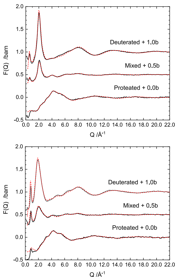
Figure 1. Total structure factor F(Q) data for isotopically unique Ca–NH 3 samples at concentrations 4 MPM (top) and 10 MPM (bottom). Data are offset by a given amount for clarity. From top to bottom: deuterated, mixed, and proteated. EPSR refinements to the data are shown by dashed red lines.
