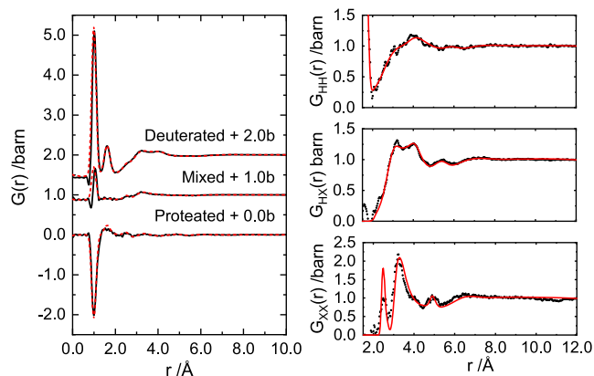
Figure 3. Left: Real space function G(r) for isotopically unique 10 MPM Ca–NH 3 samples. Data are offset by a given amount for clarity. From top to bottom: deuterated, mixed, and proteated. Right: Partial pair distribution function data for 10 MPM Ca–NH 3 . From top to bottom: G_{\text{HH}}(r) , G_{\text{HX}}(r) , and G_{\text{XX}}(r) . EPSR refinements to the data are shown by red lines.
