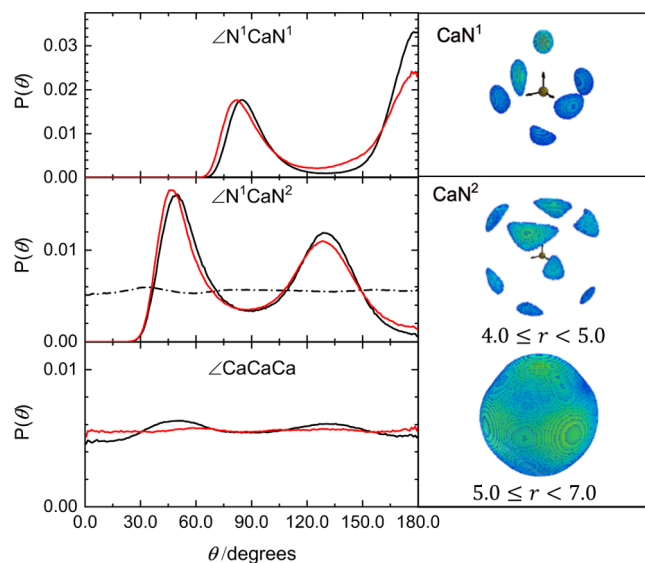
Figure 5. Left: Angular probability densities for 4 MPM (red) and 10 MPM (black) Ca–NH 3 solutions. Labels indicate primary solvation environment around Ca ( N^1 , 2 \leq r \leq 3 Å), secondary solvation ( N^2 , 4 \leq r \leq 7 Å) where the full and dashed lines for the 10 MPM system are integrated in the ranges 4 \leq r \leq 5 and 5 \leq r \leq 7 Å, respectively, and Ca ion–ion orientations. Right: Corresponding spatial density maps for N atoms around a central Ca ion in the 10 MPM system.
