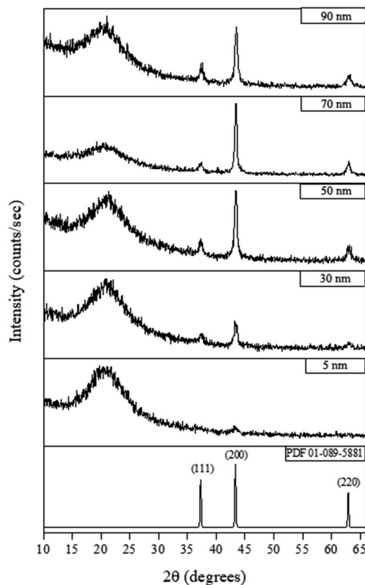
Fig. 4 Typical XRD patterns for different thickness of NiO films deposited by CVD from [\text{Ni}(\text{dmamp}')_2] at 300 °C. NiO reference pattern included [PDF 01-089-5881].
