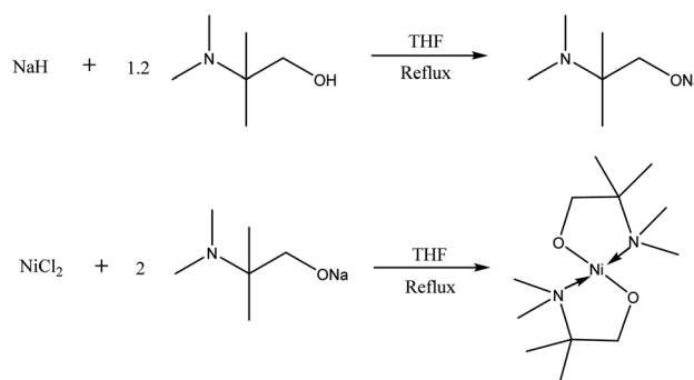
Fig. 8 Synthesis of [Ni(dmamp') 2 ].
