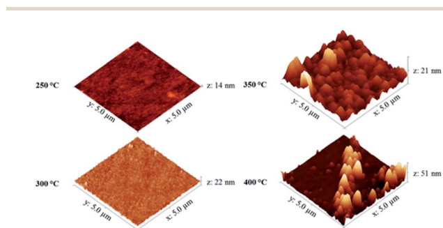
Fig. 3 AFM images of NiO films deposited by CVD of [\text{Ni}(\text{dmamp}')_2] at different substrate temperatures.
