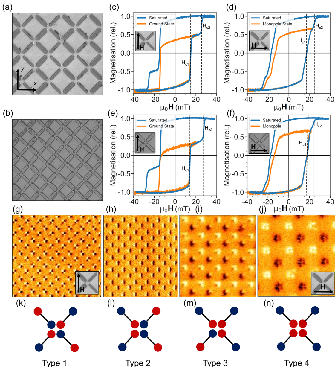
Fig. 1 Schematic of width-modified square and high-density square reconfigurable magnonic crystals and their type 1-4 microstates and hysteresis loops. y and x array axes are referred to as ‘ground-state’ and ‘monopole’ orientations throughout this work. a Scanning electron micrograph of the square sample. Bars are 830 nm long, 230 nm (wide-bar) and 145 nm (thin-bar) wide, 20 nm thick with 120 nm vertex gap (bar-end to vertex-centre). b Scanning electron micrograph of the high-density square sample. Bars are 600 nm long, 200 nm (wide-bar) and 125 nm (thin-bar) wide, 20 nm thick with 100 nm vertex gap. c–f MOKE hysteresis loops of S sample in ‘ground state’ ( c ) and ‘monopole’ ( d ) orientations, HDS sample in ‘ground state’ ( e ) and ‘monopole’ ( f ) orientations. Blue points show fully-saturating hysteresis loop, orange points show minor loops with maximum positive field value chosen to prepare sample in type 1 ( c , e ), type 4 ( d ) and type 3 ( f ) states before sweeping back to negative saturation. g–j Magnetic force microscope images of type 1–4 microstates. Type 1 and 4 states have inset SEM images showing the relative orientation of \mathbf{H}_{\text{ext}} to the width-modified subsets required for state preparation. Type 2 and 3 states may be prepared in either \pm 90^\circ field orientation. Type 1 and 4 states are often termed ‘ground state’ and ‘monopole’ state in artificial spin ice. k–n Magnetic charge dumbbell schematic of type 1–4 microstates.
