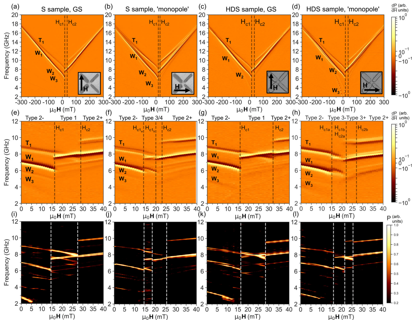
Fig. 2 Differential ferromagnetic resonance spectra of square (S) and high-density square (HDS) samples with corresponding micromagnetic simulations. Peak amplitude occurs at boundary between white and black bands. Samples were saturated in 1000 mT negative field then swept in positive field direction, with relative field orientation indicated in inset scanning electron micrographs. Measurements were performed at room temperature. Fields were swept from \pm 300 mT, with full sweeps (a–d), 0–40 mT sweeps around the coercive fields (e–h) and micromagnetic MuMax3 simulations of the coercive field region (i–l) presented. Sample geometry and \mathbf{H}_{ext} orientation are shown inset. Switching fields are labelled by vertical dashed lines, a and b subscripts refer to separate \pm 45^\circ subset reversal where applicable, type 3- and 3+ refer to thin-bar majority and wide-bar majority type 3 states respectively. From left to right, vertical columns of spectra relate to samples: S ('ground-state' orientation), S ('monopole' orientation), HDS ('ground-state' orientation), HDS ('monopole' orientation).
