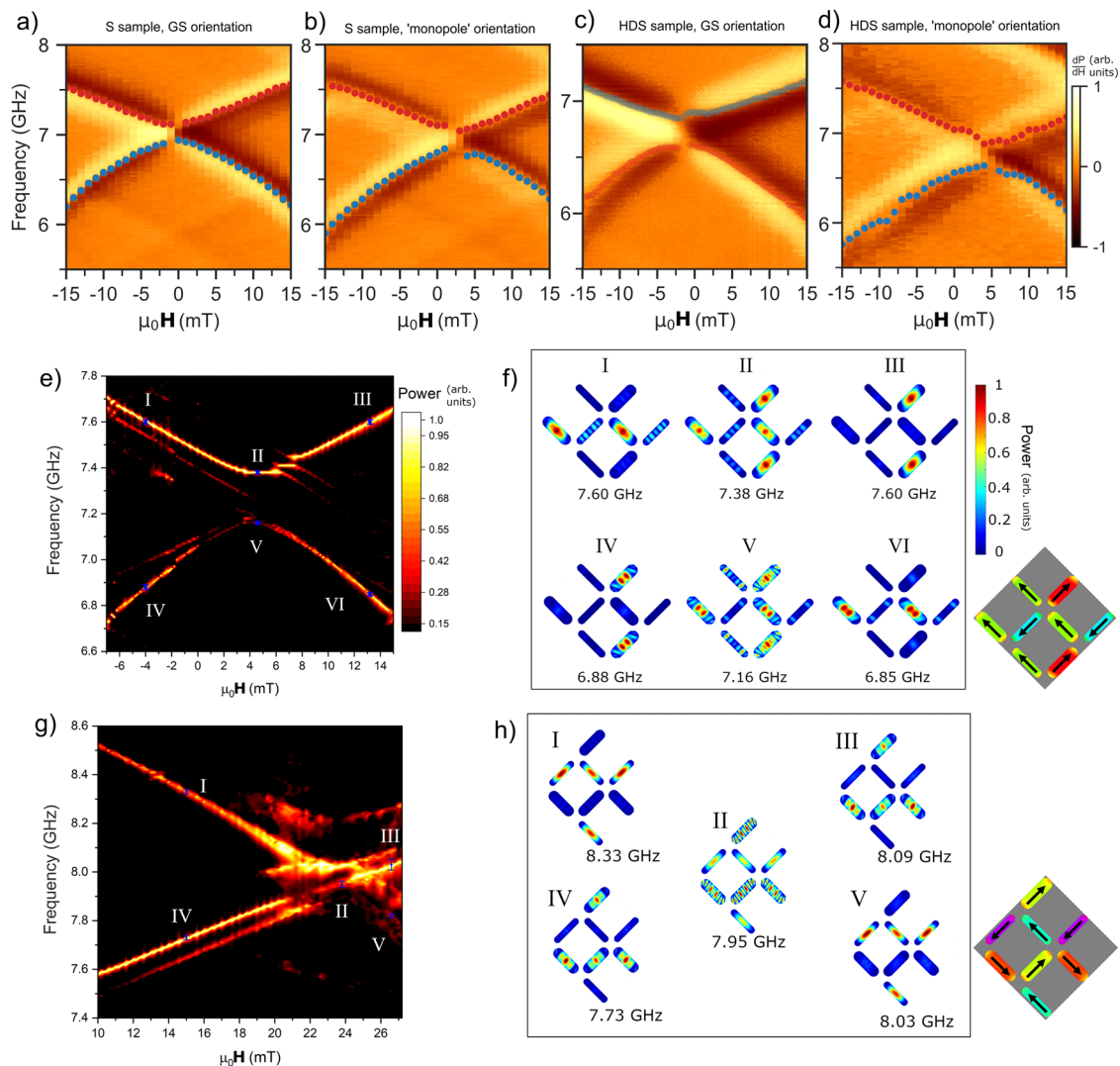
Fig. 4 Mode-hybridisation and anticrossings. a–d Negative-swept field dependent experimental FMR spectra of type 3 states for S and HDS samples in ground-state and 'monopole' orientations. Red scatter points are peak extractions of the upper mode branch, blue points extractions of the lower branch. Mode frequency gaps and anticrossings and mode bending in the field range around the crossing point are observed in all samples and orientations. Monopole-orientation crossing points (panels b and d ) are offset in positive H_{ext} due to the net H_{loc} at the vertex, ground state orientation crossings ( a and c ) are offset at lower magnitude, negative H_{ext} due to the different H_{loc} profile along this axis. e Simulated spectra of monopole-orientation HDS sample. Anticrossing gap of 0.32 GHz is observed at 4.3 mT. Error bars correspond to frequency range integrated over to produce spatial mode plots shown in f . f Simulated spatial mode-power maps for monopole-orientation HDS sample. Maps I–VI relate to corresponding points labelled on spectra in panel e . High-frequency, single-node mode branch is seen in I–III. Low-frequency, multi-node branch is IV–VI. g Simulated type 1 spectra of ground-state orientation HDS sample. Crossing occurs at 24 mT with no observable gap. Error bars correspond to frequency range integrated over to produce spatial mode plots shown in h . h Simulated spatial mode-power maps for ground-state orientation type 1 HDS sample. Maps I–V relate to corresponding points labelled on spectra in panel e . Mode-hybridisation is not observed, with matching profile pairs I and V, IV and III.
