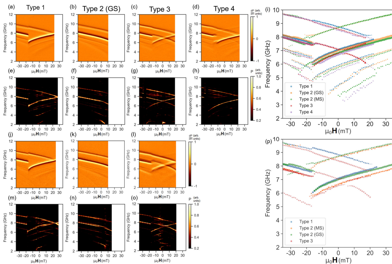
Fig. 3 Differential ferromagnetic resonance spectra taken while negatively sweeping H_{ext} after microstate preparation in positive field. Microstates were prepared by -1000 mT saturation then applying the positive field required to reverse the desired bars, hence differing positive field limits for different microstate spectra. a–d Experimental spectra for S sample microstates taken in ‘ground-state’ ( a, b ) and ‘monopole’ ( c, d ) orientations. e–h Simulated S sample microstate spectra for ‘ground-state’ ( e, f ) and ‘monopole’ ( g, h ) orientations. i Mode peak-extractions for all S sample microstate-spectra. j–l Experimental spectra for HDS sample microstates taken in ‘ground-state’ ( j, k ) and ‘monopole’ ( l ) orientations. ‘Monopole’ orientation signal-to-noise is lower due to array-waveguide alignment issues. Modes are still well-resolved and correspond well with simulation. m–o Simulated HDS sample microstate spectra for ‘ground-state’ ( m, n ) and ‘monopole’ ( o ) orientations. p Mode peak-extractions for all HDS sample microstate-spectra.
