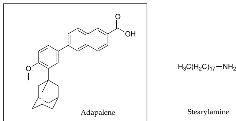
Figure 18. Adapalene and stearylamine counter ion.
