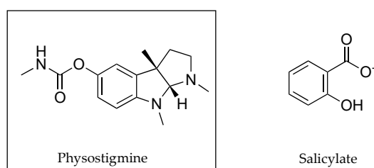
Figure 12. Counter ions PHY and Salicylate.
