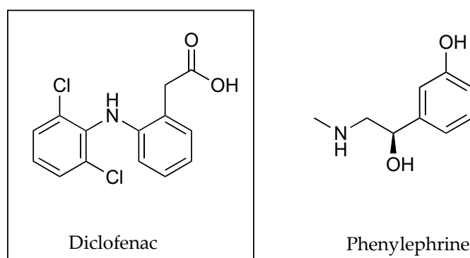
Figure 17. DIC and phenylephrine counter ion.
