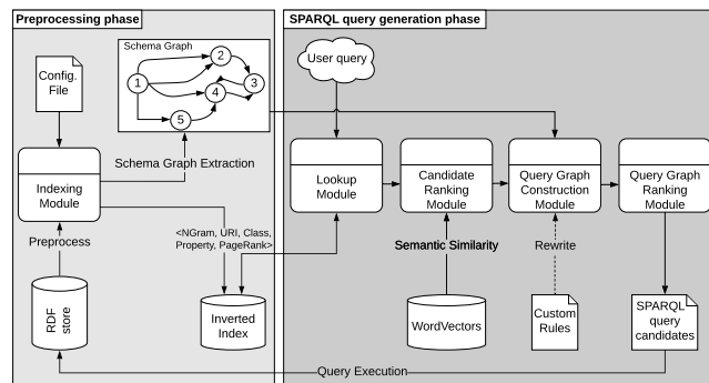
Figure 4: Bio-SODA System Architecture
