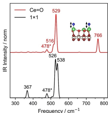
Figure 4. Calculated IR spectra for the Ce=O-terminated (\sqrt{3}\times\sqrt{3})\text{R}30^\circ -reconstructed and (1\times 1) unreconstructed \text{CeO}_2(111) surfaces. The model for the Ce=O-terminated (\sqrt{3}\times\sqrt{3})\text{R}30^\circ surface is the same as that in Figure 3. The 478\text{ cm}^{-1} mode observed for both is ascribed to vibrations against the fixed layer of the DFT slab. [22]
