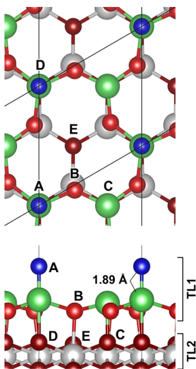
Figure 3. Top and side views of the proposed Ce=O termination of \text{CeO}_2(111)-(\sqrt{3}\times\sqrt{3})\text{R}30^\circ . The larger spheres are Ce and the smaller are O. The Ce=O bond is between the green Ce to blue O, with a calculated bond distance of 1.89 Å. The inequivalent O atoms in the outermost three oxygen layers are denoted A (Ce=O in TL1), B (TL1) and C–E (TL2).
