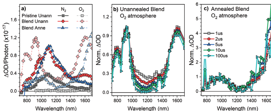
Figure 8. a) TA spectra obtained at 1 \mu s for the unannealed pristine DRCN5T (black squares), and the unannealed (red diamonds) and annealed (blue triangles) DRCN5T:PC70BM 1:0.8 blend under nitrogen (solid line and darker color symbols) and oxygen (dashed line and lighter color symbols) atmospheres. These spectra were normalized per photon absorbed. Normalized TA spectra recorded over a time range from 1 to 100 \mu s for b) unannealed and c) annealed blend samples under oxygen atmosphere. Spectra were recorded with a pump wavelength of 500 nm, at 10–15 \mu J \text{ cm}^{-2} excitation density.
