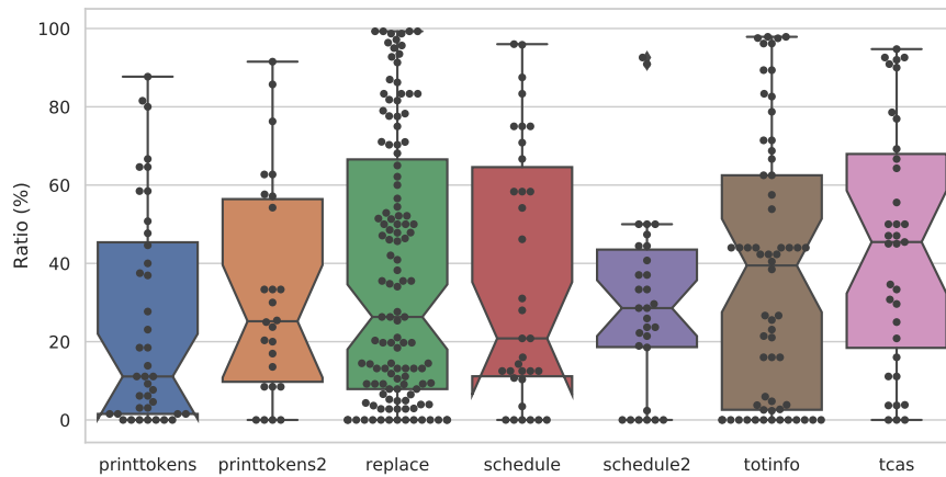
Figure 10: Distribution of the ratio of the number of lines only in a CodeSurfer slice to the CodeSurfer slice size.
