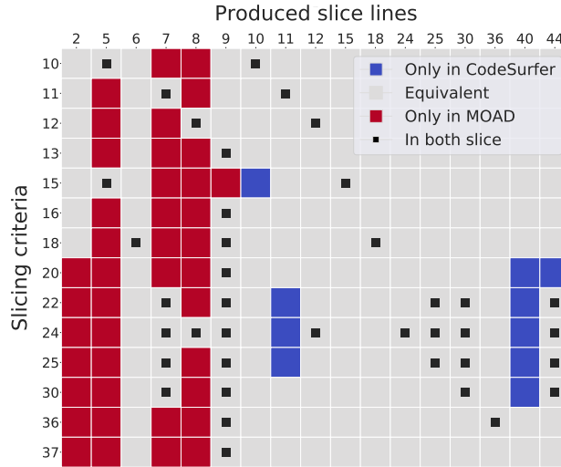
Figure 6: Difference of the backward slices of MOAD and CodeSurfer of wc
