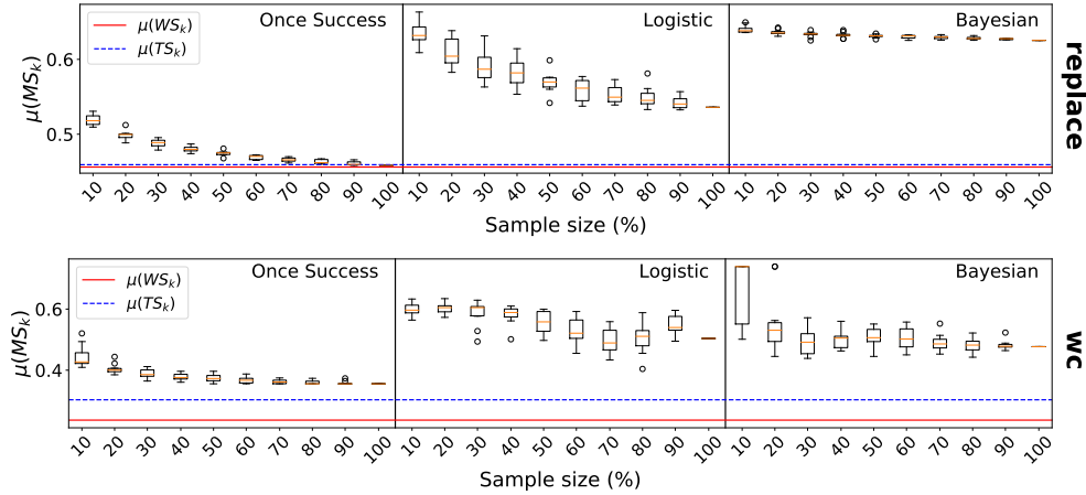
Figure 7: Averaged over all slicing criteria for replace (top) and wc (bottom), the figure presents the mean slice size of MOAD, \mu(MS_k) , given as a percentage of the size of the original program for a range of 2-hot sample sizes (shown on the x -axis). Each boxplot summarizes the performance of a model built using ten different random samples. The red and blue lines represent the means for W-ORBS and T-ORBS slice size, averaged over all slicing criteria in the program.
