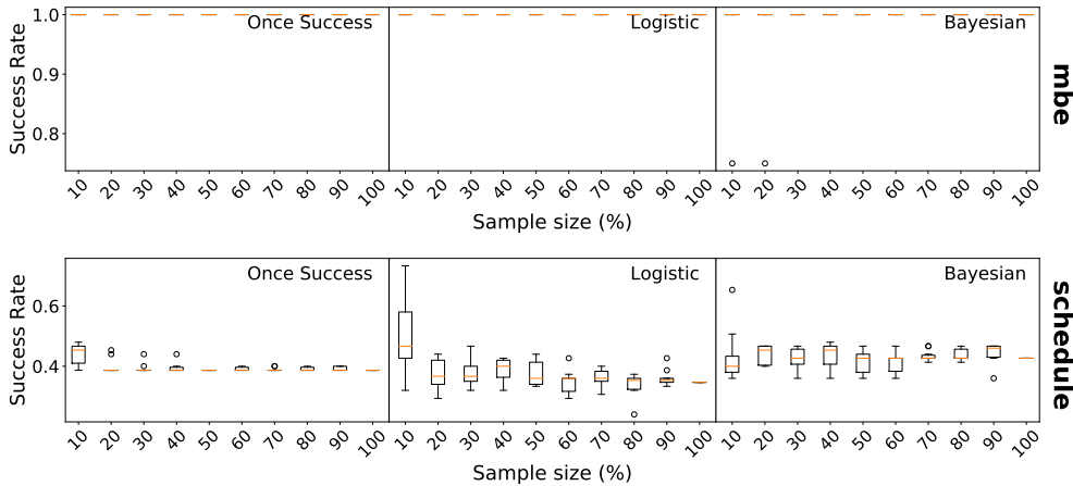
Figure 8: The figure presents MOAD’s mean success rate averaged over all slicing criteria for mbe (top) and sched (bottom). Each boxplot summarizes the performance of a model built using ten different random samples.
