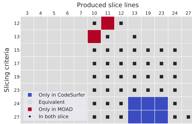
Figure 4: Difference of the backward slices of MOAD and CodeSurfer of mbe
