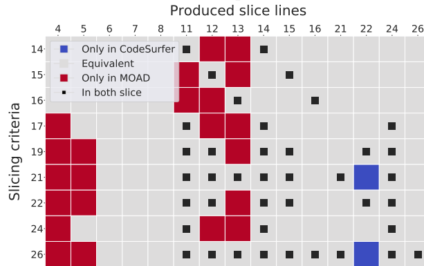
Figure 5: Difference of the backward slices of MOAD and CodeSurfer of mug
