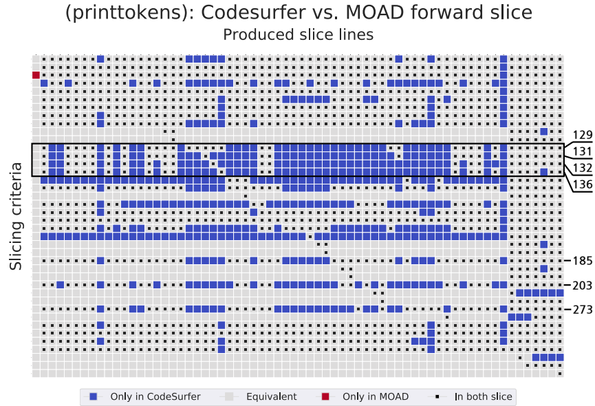
Figure 9: Difference of the forward slices of MOAD and CodeSurfer of prttokens
