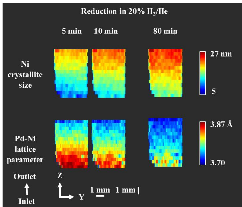
Figure 6. Phase distribution maps of Ni crystallite size and Pd-Ni lattice parameter obtained through Rietveld analysis of the XRD maps collected during reduction step. XRD maps are presented from the inlet of reactor towards the outlet of reactor. Corresponding diffraction patterns can be found in the Supporting Information (Figure S14).
