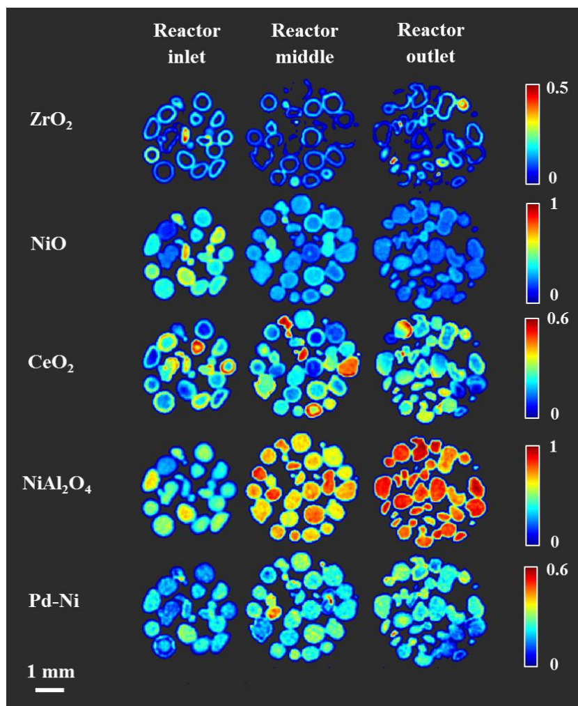
Figure 4. Phase distribution maps created from the Rietveld analysis of XRD-CT data collected (normalised scale factors) collected at three different positions: reactor inlet, middle of reactor and outlet of reactor under atmosphere of He at 800 °C (according to the order of data collection).
