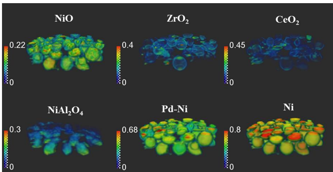
Figure 7. Volume rendering of the normalised scale factors data volume (normalised over the maximum value of scale factor in the entire process) obtained from the Rietveld analysis of the 3D-XRD-CT data collected during the reduction process at 800 °C under 20 % of H_2/He .
