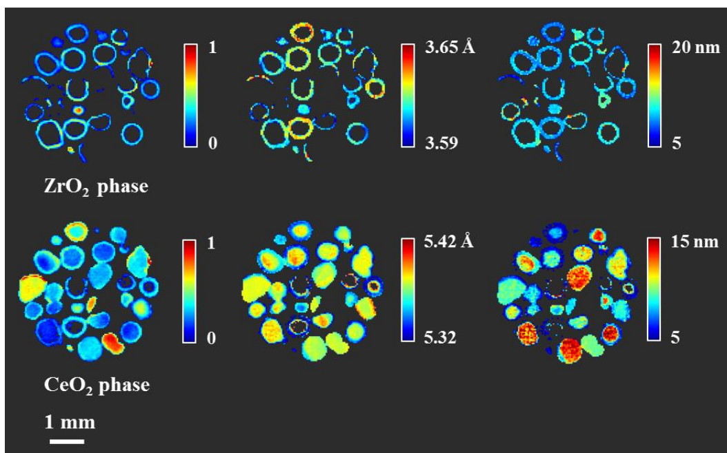
Figure 2. Spatial distribution of normalised scale factor (in respect to maximum value in this XRD-CT image), spatial distribution of crystallite size and lattice parameter a for \text{CeO}_2 and \text{ZrO}_2 collected at room temperature (fresh catalyst).
