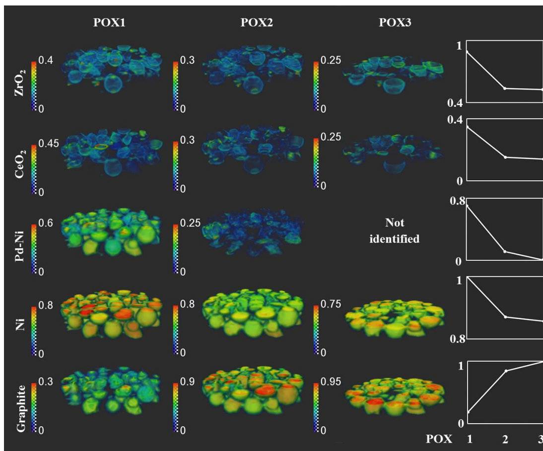
Figure 9. Volume rendering of the normalised scale factors data volume (normalised over the maximum value scale factor reading in the entire process) obtained from the Rietveld analysis of the 3D-XRD-CT data collected during the reaction mixture POX1, POX2 and POX3. Plots on the right corresponds to normalise mean scale factors 3D volume during the POX reaction conditions (for normalised mean scale factors during the entire experiment see Figure S24). The normalisation was done with respect to maximum value for the entire experiment. Note that only five XRD-CT slices were collected for POX3 reaction mixture.
