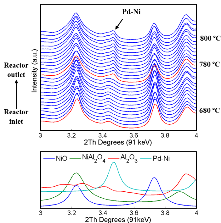
Figure 3. Top: summed diffraction patterns collected with diffraction mapping (150 diffraction patterns summed for one line scan) during the temperature ramp in He. The chosen region of interest shows the two last maps (from 680 °C to 800 °C with the step of around 5 °C between the line scans). The red lines indicate the beginning of each map and the data are presented from the inlet of reactor towards the outlet of reactor. Bottom: simulated diffraction patterns for NiO, NiAl 2 O 4 , Al 2 O 3 and Pd-Ni.
