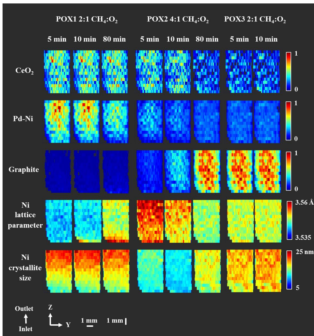
Figure 8. Phase distribution maps of normalised scale factors for \text{CeO}_2 , Pd-Ni and graphite, Ni lattice parameter and Ni crystallite size obtained through Rietveld analysis of the XRD maps collected during POX reaction. XRD maps are presented from the inlet of reactor towards the
