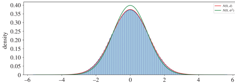
Figure 1. Steady-state distribution of opinions. N(0, d) is a better fit of the data than N(0, \sigma^2) .
