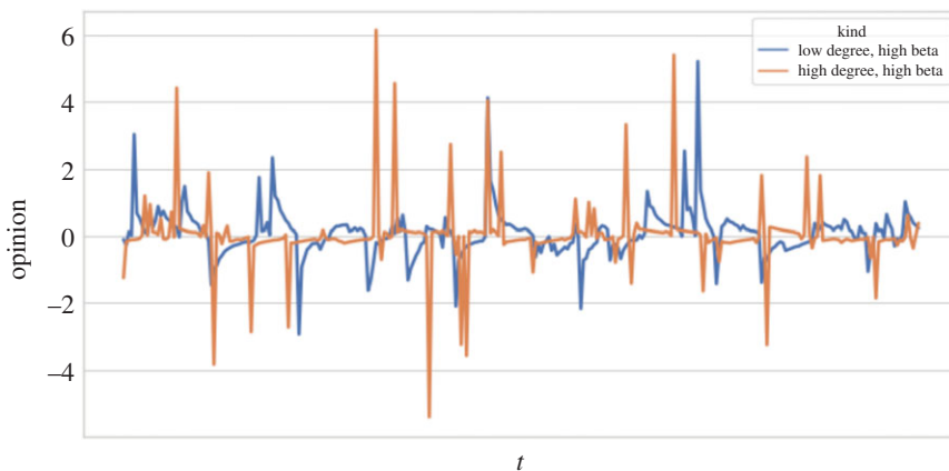
Figure 8. Example highlighting why d increases with p when \beta \gg 0 .
