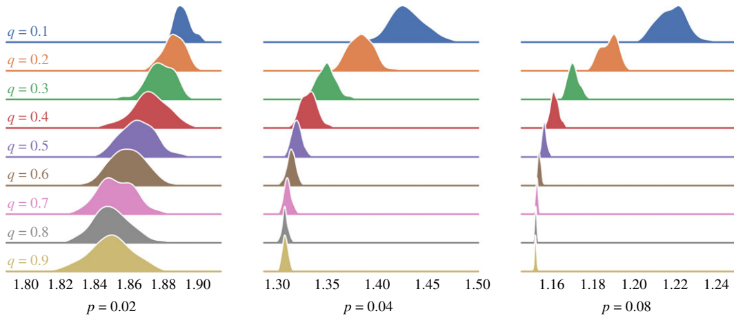
Figure 5. Distribution of opinion diversity grouped by q (rows) and p (columns).
