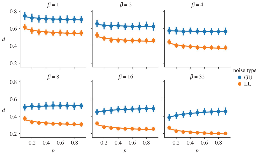
Figure 7. How opinion diversity varies with connectivity for the GU and LU model depending on \beta .
