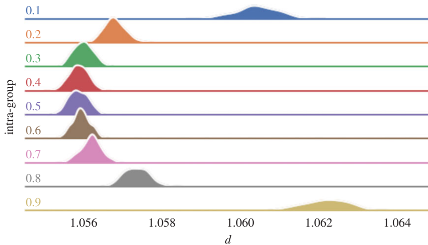
Figure 6. Distribution of opinion diversity for networks with average degree k = 0.5N .
