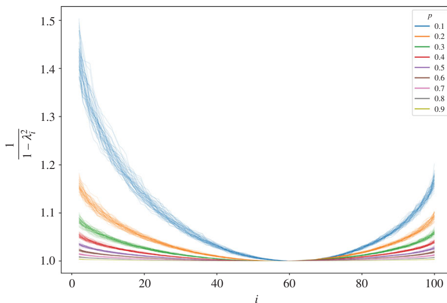
Figure 4. The marginal contribution of \lambda_i to d for each network.
