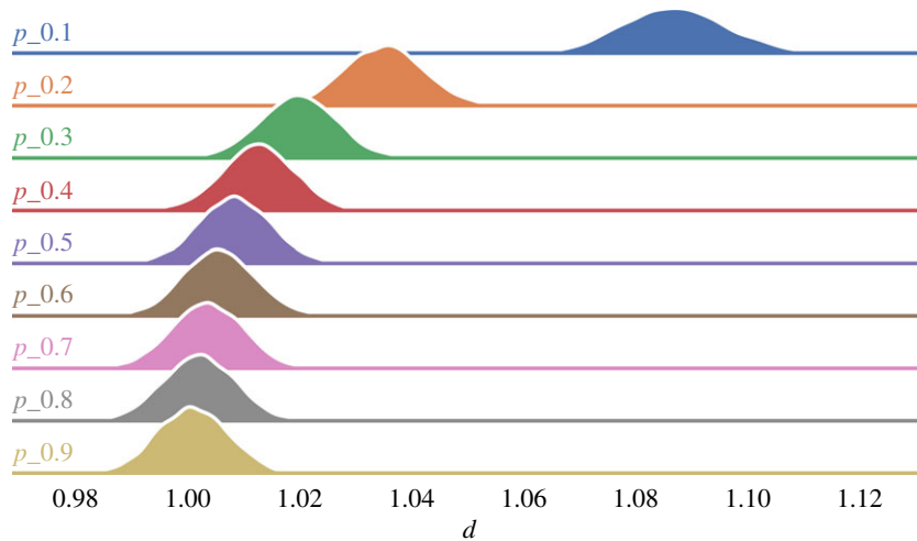
Figure 3. Distribution of opinion diversity, d , grouped by network connectivity, p .
