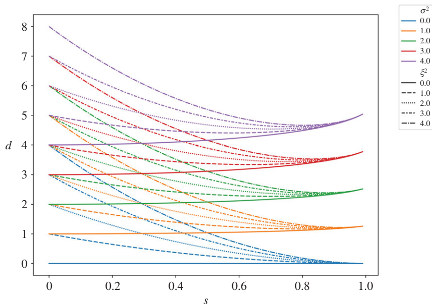
Figure 2. How opinion diversity varies with the susceptibility for different configurations of noise.
