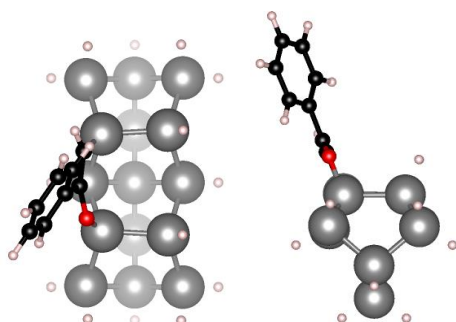
c) End-bridge flagpole
