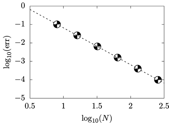
FIG. 3. Four roll mill: the slope of the line fitting our results (triangles) indicates a convergence rate of 1.998.
