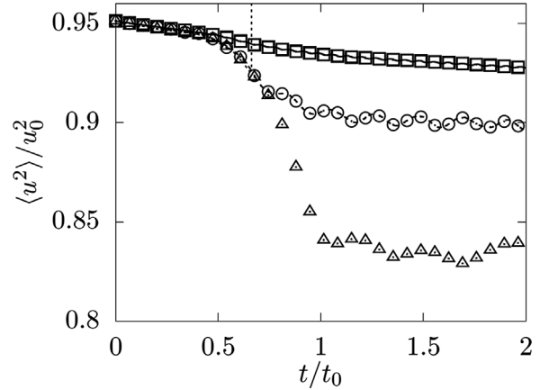
FIG. 4. Double shear layer: evolution of the normalized kinetic energy computed by the present scheme (lines) and the BGK LBM (symbols) for different values of the Mach number: 0.1 (solid line and squares), 0.3 (dashed line and circles), and 0.6 (dotted line and triangles).
