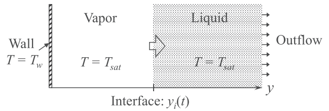
FIG. 8. Schematic representation of the Stefan problem.
