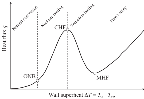
FIG. 1. Typical boiling curve representing the relation between heat flux and wall superheat. ONB, CHF, and MHF denote the onset of nucleate boiling, critical heat flux, and minimum film boiling, respectively.
