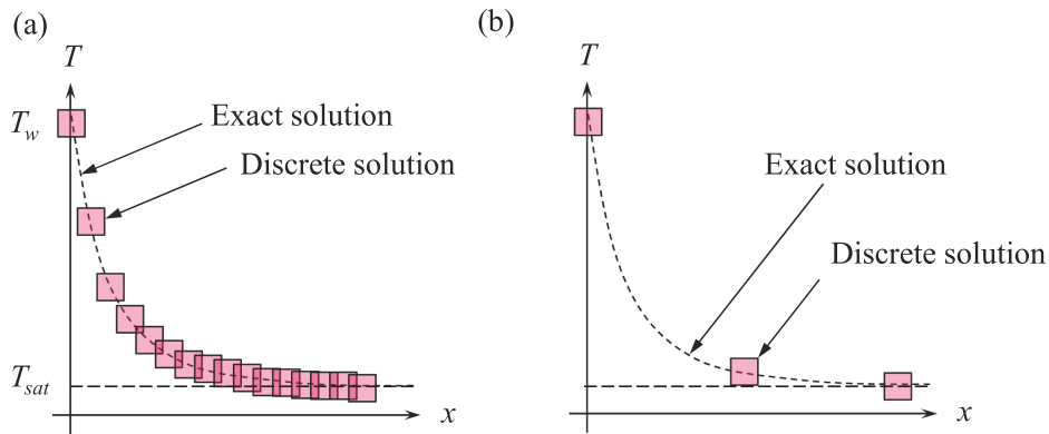
FIG. 18. One-dimensional concept of the relation between exact and discrete solutions: (a) low Reynolds number and (b) high Reynolds number.
