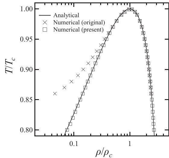
FIG. 6. Simulation of the two-dimensional circular bubble with \nu = 0.1 . Line: Maxwell's equal rule area. Symbol: lattice Boltzmann simulation with \sigma = 0 and \sigma = 0.38 . The case of \sigma = 0 corresponds to the original consistent scheme. 70
