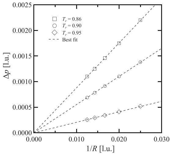
FIG. 7. Laplace's law for several reduced temperatures: T_r = 0.86 , T_r = 0.90 , and T_r = 0.95 .
