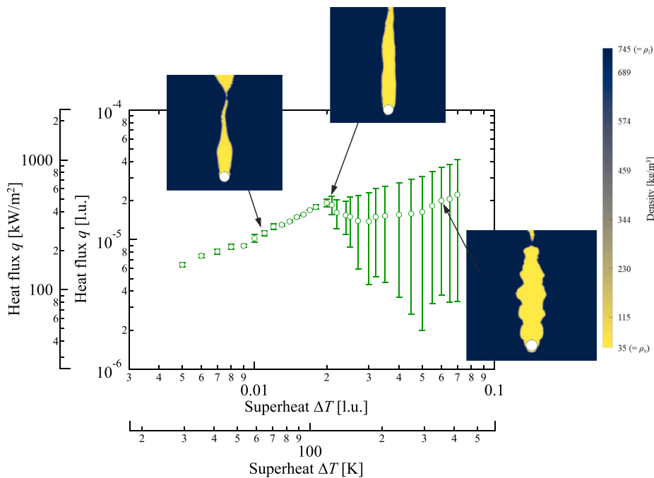
FIG. 15. Boiling curve for Re=30\,000 and Pr=1.5 . The snapshot of density distributions for \Delta T = 0.012 l.u. ( =71 K), \Delta T = 0.021 l.u. ( =125 K), and \Delta T = 0.060 l.u. ( =356 K) is included in the figure.
