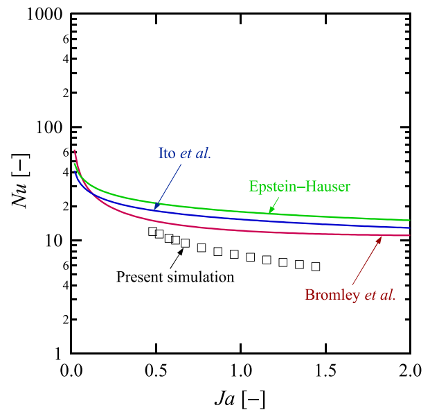
FIG. 19. Comparison of the low-Prandtl-number simulation results (open symbols) with mode 1 8 and mode 2 5,10 correlations for cylinders.
