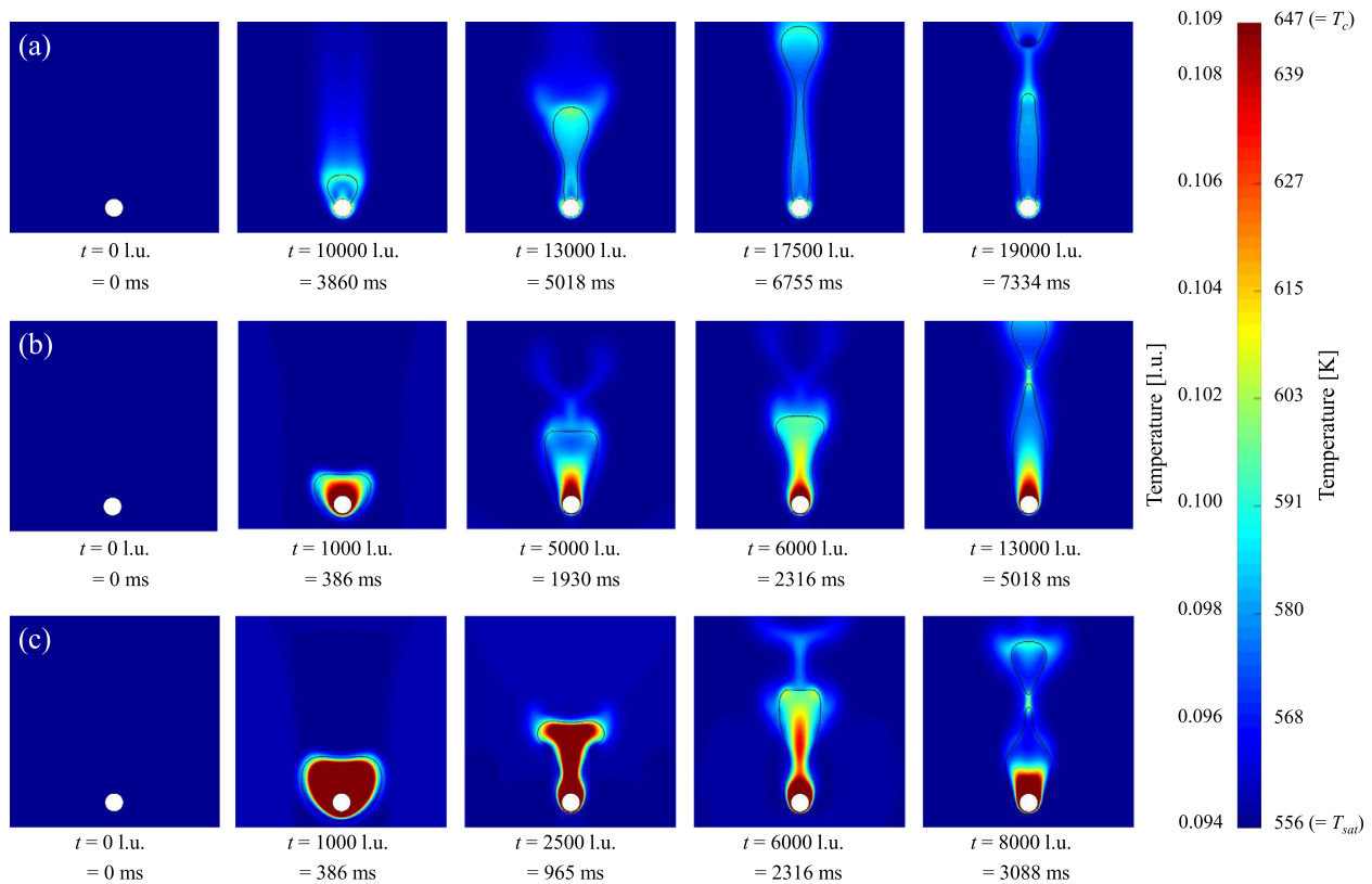
FIG. 12. Snapshots of temperature distribution during convection boiling on a cylindrical body at Re = 30 and Pr = 1.5 : (a) \Delta T = 0.010 l.u. ( = 59 K), (b) \Delta T = 0.023 l.u. ( = 137 K), and (c) \Delta T = 0.060 l.u. ( = 356 K). Solid lines in the pictures represent the interface defined by (\rho_l + \rho_v)/2 .
