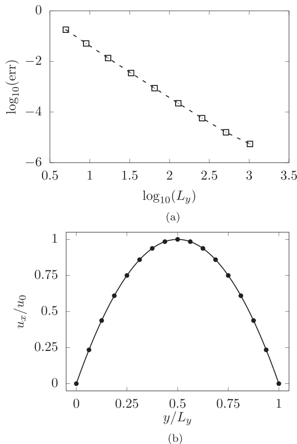
FIG. 5. Poiseuille flow: (a) convergence analysis showing an optimal convergence rate equal to 2.04 and (b) profile of the horizontal component of the velocity, u_x , normalized with respect to u_0 from the analytical predictions (continuous line) and our numerical scheme (circles).
