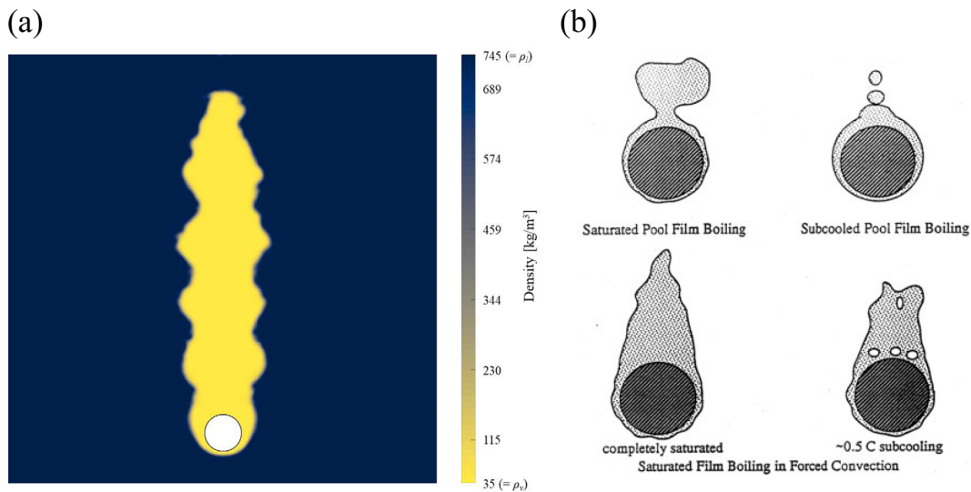
FIG. 16. Comparison of simulation results and conceptual illustration of several film-boiling regimes reproduced from Liu and Theofanous. 8 (a) Snapshot of simulation results for Re = 30\,000 and (b) conceptual illustration of the film-boiling regime, including saturated pool film boiling, subcooled pool film boiling, completely saturated film boiling in forced convection, and slightly subcooled film boiling in forced convection.
