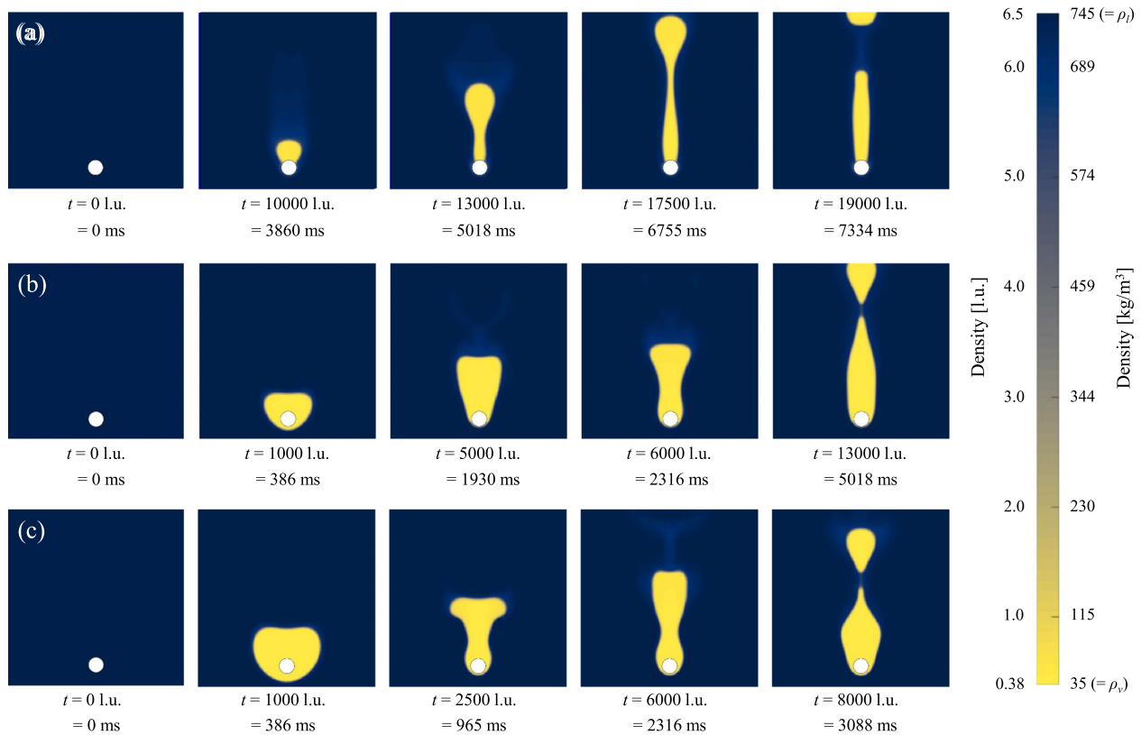
FIG. 11. Snapshots of density distribution during convection boiling on a cylindrical body at Re = 30 and Pr = 1.5 : (a) \Delta T = 0.010 l.u. ( = 59 K), (b) \Delta T = 0.023 l.u. ( = 137 K), and (c) \Delta T = 0.060 l.u. ( = 356 K).
