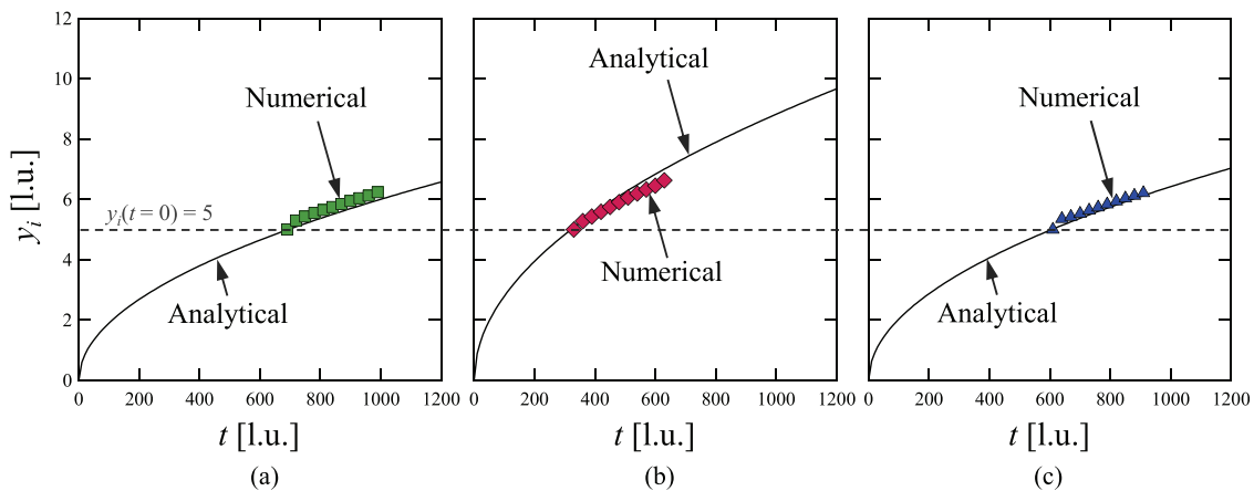
FIG. 9. Comparison of the present LBM results with the analytical solutions to the Stefan problem under several conditions: (a) T_r = 0.86 , \Delta T = 0.010 ; (b) T_r = 0.86 , \Delta T = 0.023 ; and (c) T_r = 0.90 , \Delta T = 0.010 . Solid lines represent the analytical solution [Eq. (41)].
