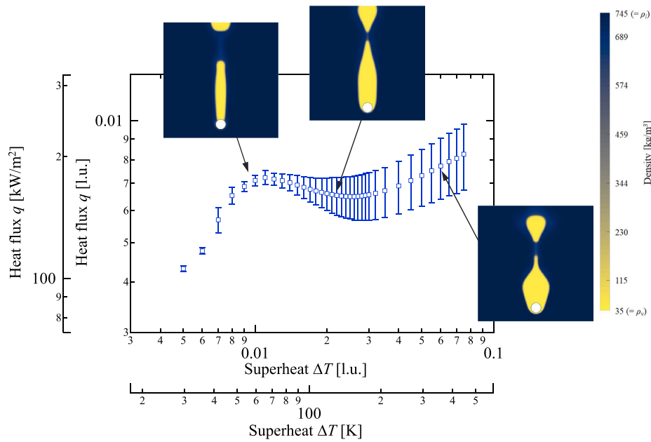
FIG. 14. Boiling curve for Re=30 and Pr=1.5 . The snapshot of density distributions for \Delta T = 0.010 l.u. ( =59 K), \Delta T = 0.023 l.u. ( =137 K), and \Delta T = 0.060 l.u. ( =356 K) is included in the figure.
