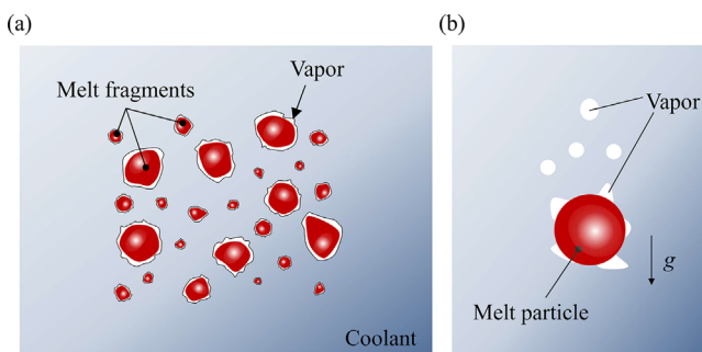
FIG. 2. Schematic diagram of the possible FCI scenario: (a) melt fragments distributed in the coolant and (b) a simplified situation with a single melt particle in a coolant.
