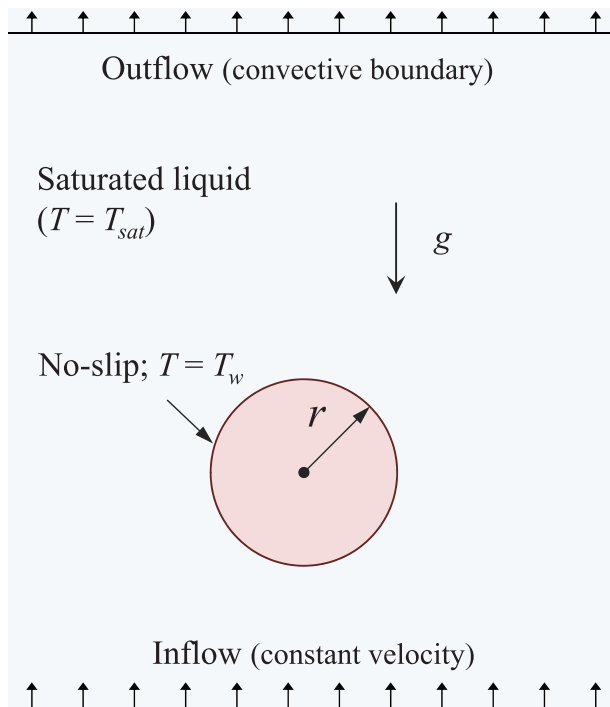
FIG. 10. Boundary conditions for the boiling simulations.
