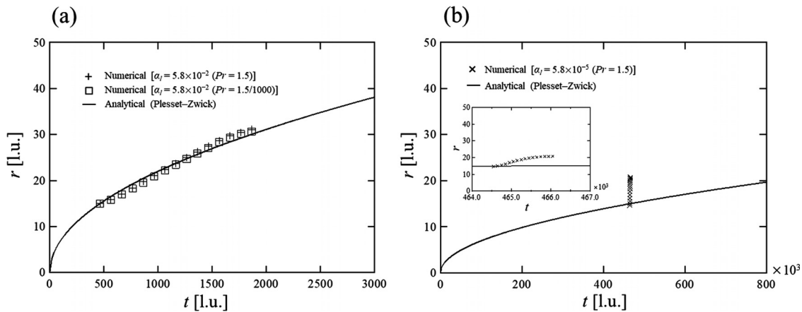
FIG. 21. Comparison of the present simulation results with the Plesset–Zwick equation: (a) \alpha_l = 5.8 \times 10^{-2} and (b) \alpha_l = 5.8 \times 10^{-5} in lattice units.
