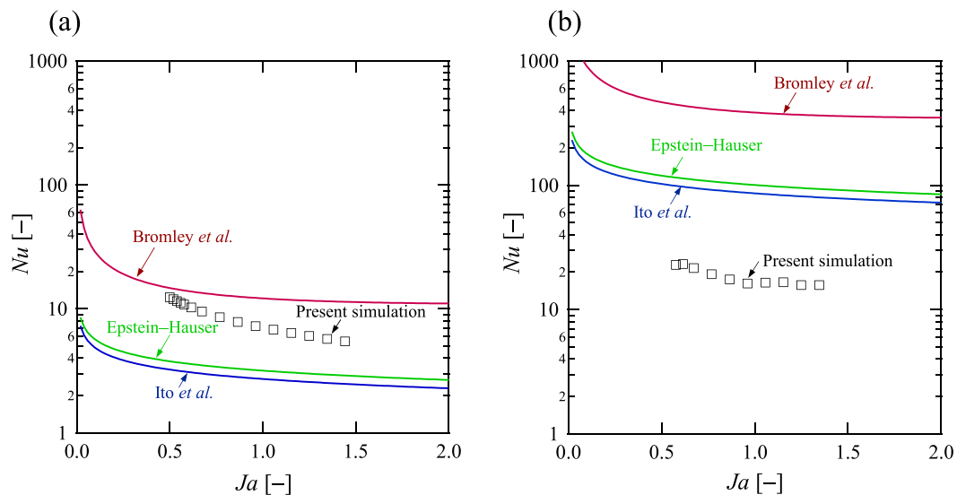
FIG. 17. Comparison of the simulation results (open symbols) with mode 1 8 and mode 2 5,10 correlations for cylinders. (a) Re = 30 and (b) Re = 30\,000 .
