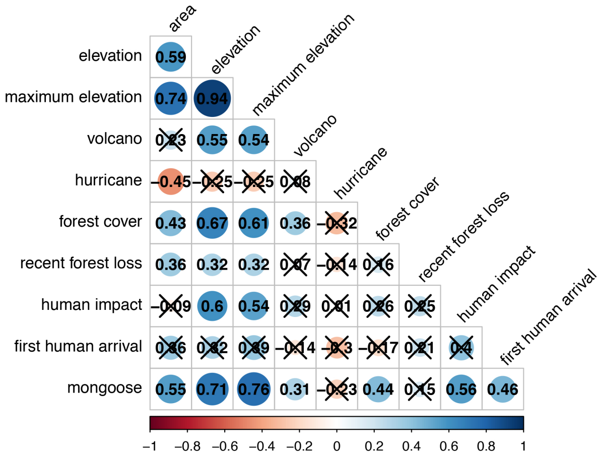
Figure S1. Correlation coefficients among island variables, with colour intensity corresponding to stronger negative (red) or positive (blue) correlation. Crossed-out values were not significant at \alpha = 0.01 .
