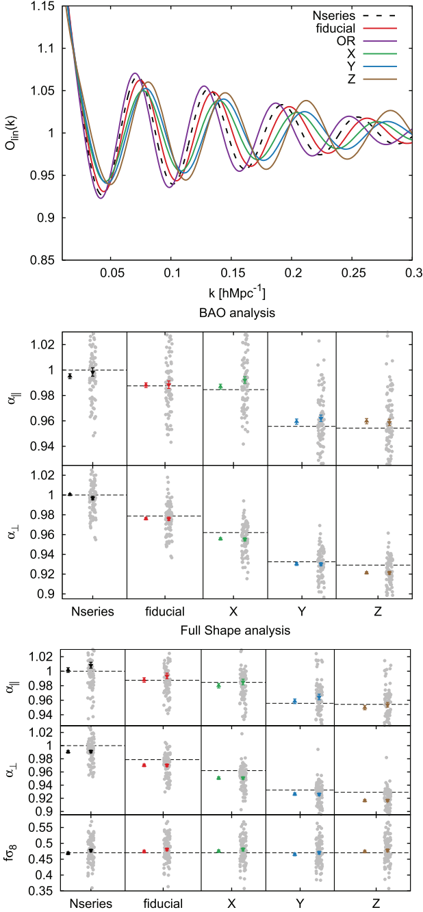
Figure 10. Top panel: BAO signal, O_{\text{lin}}(k) of the cosmologies listed in Table 1 (except for \Theta_{\text{EZ}} ), used to test the cosmology dependence of the BAO and FS analyses with the reference cosmology displayed in the middle panel (BAO analysis on post-recon catalogues and listed in Table F4) and in the bottom panel (FS analysis on pre-recon catalogues listed in Table F5). Middle panel: BAO scale factors along ( \alpha_{\parallel} ) and across ( \alpha_{\perp} ) the LOS measured on the reconstructed Nseries mocks. The \Delta symbols display the fit on the mean of the 84 realizations, the grey symbols display the fit on the individual 84 realizations, and the \nabla symbols the mean of the 84 individual fits. The error associated is the error of the mean and the rms among the 84 realizations divided by \sqrt{84} , respectively. Bottom panel: same notation than the middle panel applied to FS analysis on the same mocks. The x-axis shows the results for different cosmologies used for the template (and for mapping redshifts into comoving distances when computing the power spectrum). The horizontal dashed lines mark the expected value of \alpha_{\parallel, \perp} , and f\sigma_8 .
