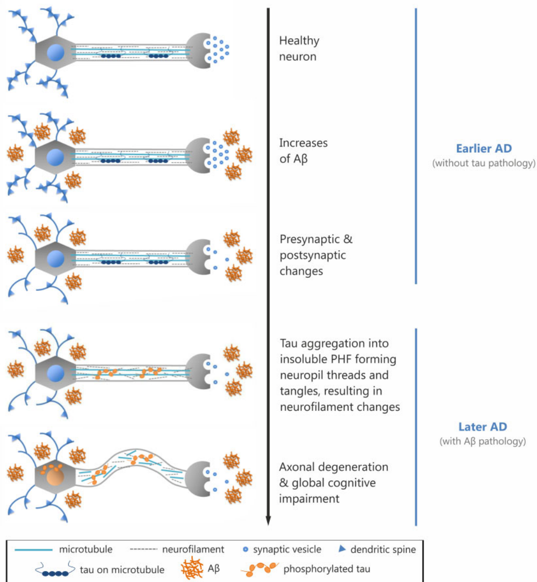
Figure 6 Schematic hypothetical representation of the downstream effects of amyloid- \beta and tau on synaptic and axonal function in earlier and later Alzheimer's disease stages. In earlier disease stages (amyloid- \beta + Tau- and amyloid- \beta -Tau-), the accumulation of amyloid- \beta into plaques reduces the number of postsynaptic spines and the number of presynaptic vesicles, altering local synaptic communication. In later disease stages (amyloid- \beta + Tau+ and amyloid- \beta + Tau-), as synaptic changes become more pronounced, tau becomes phosphorylated and aggregates into insoluble paired helical filaments (PHF), which form neurofilament threads and neurofibrillary tangles. These changes are followed by the dissociation of neurofilaments from microtubules, axonal degeneration and ultimately global cognitive impairment. A \beta = amyloid- \beta ; AD = Alzheimer's disease.
