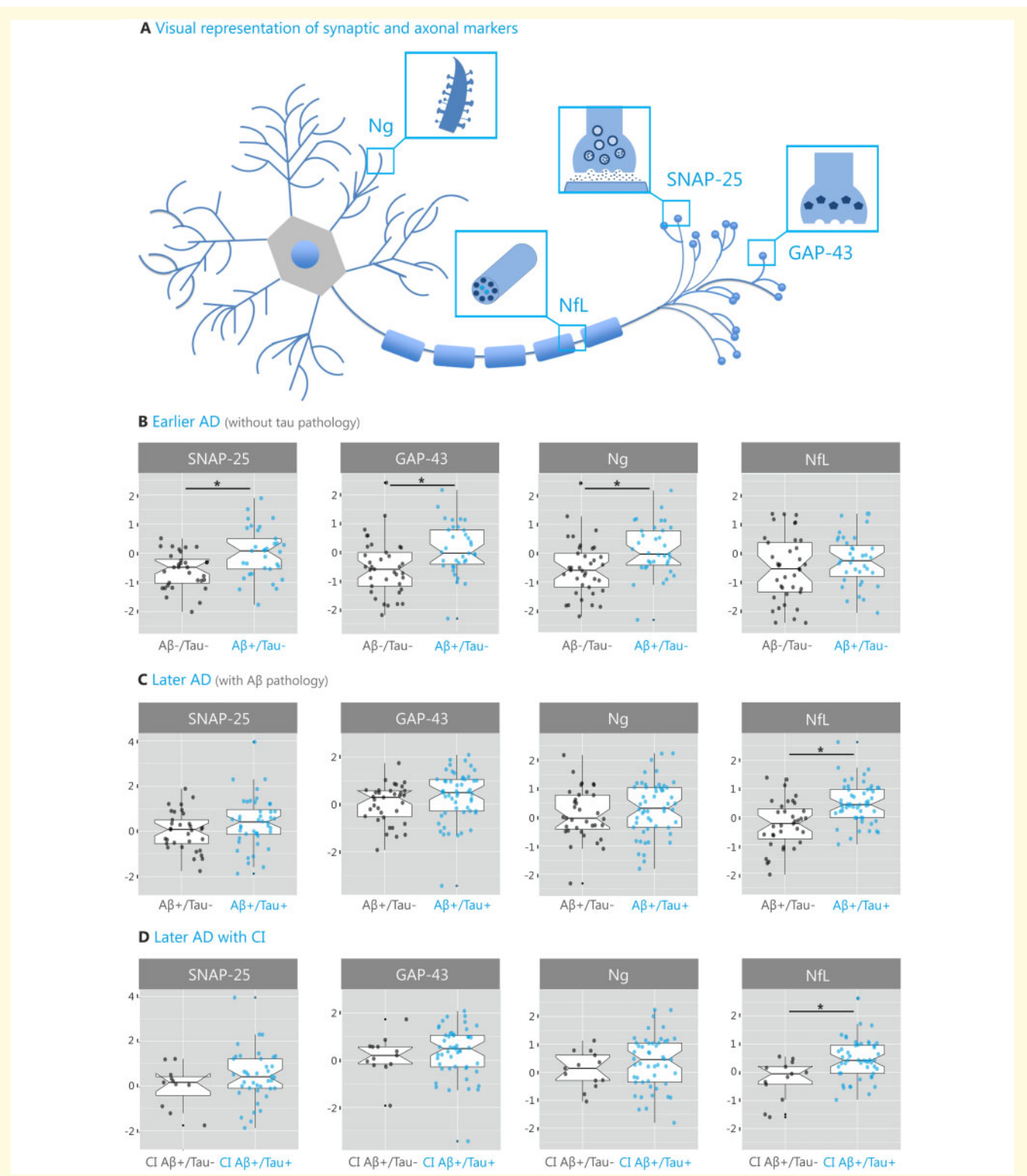
Figure 1 Synaptic and axonal markers change in earlier and later Alzheimer's disease stages. (A) Representation of the neuronal aspects measured by the postsynaptic [NRGN (Ng)], axonal (NfL) and presynaptic markers (SNAP25; GAP43). (B) In early Alzheimer's disease stages, SNAP25, GAP43 and NRGN show significant increases in amyloid- \beta + ( A\beta +) compared to amyloid- \beta - ( A\beta -) individuals without evidence of tau PET retention (Tau-). (C) In later Alzheimer's disease stages, NfL shows significant increases in Tau+ compared to Tau- individuals who are all amyloid- \beta +. (D) The increases in NfL in the previous groups can still be observed when only cognitively impaired (CI) individuals are considered. These analyses were performed using t -tests, while controlling for covariates. The values presented in the plots are the residuals of SNAP25, GAP43, NRGN and NfL after regressing out the effects of age (all CSF markers) in addition to sex (NfL).
