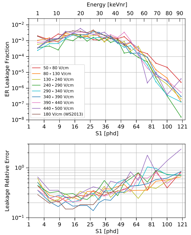
FIG. 31. Top: an estimate of the electronic recoil two-factor leakage fraction for a flat energy spectrum in S1 bins, for various values of drift field. The leakage fraction is estimated by multiplying the charge-to-light leakage by the ratio of two-factor to charge-to-light leakage (i.e., the results in Figs. 28 and 30, respectively). This is an estimate for two reasons: first, the two calculations use different S1 bins; second, the charge-to-light leakage is a skew-Gaussian extrapolation, while the ratio is based on counting individual events, so they are not perfectly consistent. The S1 axis is proportional to \sqrt{S1} . The equivalent nuclear recoil energy for an S1 is calculated by using the S1 and S2c at the median of the NR band; this varies by field, but not significantly, so we report the energy averaged over the eight field bins. Bottom: the relative error on these leakage fraction values, defined as \text{leakage\_fraction\_error}/\text{leakage\_fraction} . Note that the leakage relative error can be greater than 1, indicating that the leakage fraction is consistent with 0.
