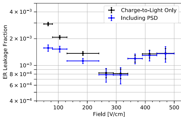
FIG. 16. The integrated electronic recoil leakage for a flat recoil energy spectrum from 1 to 80 S1 photons detected (equivalent to 2–65 keVnr), while varying drift field in WS2014–16 data. The leakage is calculated using only the charge-to-light ratio, i.e., \log_{10}(S2c/S1) , and using both charge-to-light and pulse-shape discrimination in tandem. Both leakage values are based on the “counting” method described in Fig. 13, where we count the number of electronic recoils leaking into the nuclear recoil 50% acceptance region.
