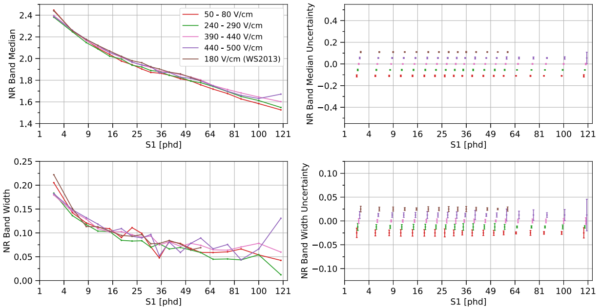
FIG. 9. The median and width \sigma_- of the NR band for several drift fields. The left plots show measurements, and the right plots display error bars corresponding to these measurements. The S1 axis is proportional to \sqrt{S1} . The NR band for WS2013 is adjusted, so g_2 is consistent for the WS2013 and WS2014–16 results. In each row, the y-axes have the same range; the size of the error bars on the right plot can be directly translated to the points on the left plot. For ease of visualization on the right plots, the S1 values are slightly shifted relative to their true value, and the error bars are centered at a different y-value for each field bin. See Fig. 25 for the NR band median and width for all the field bins we considered.
