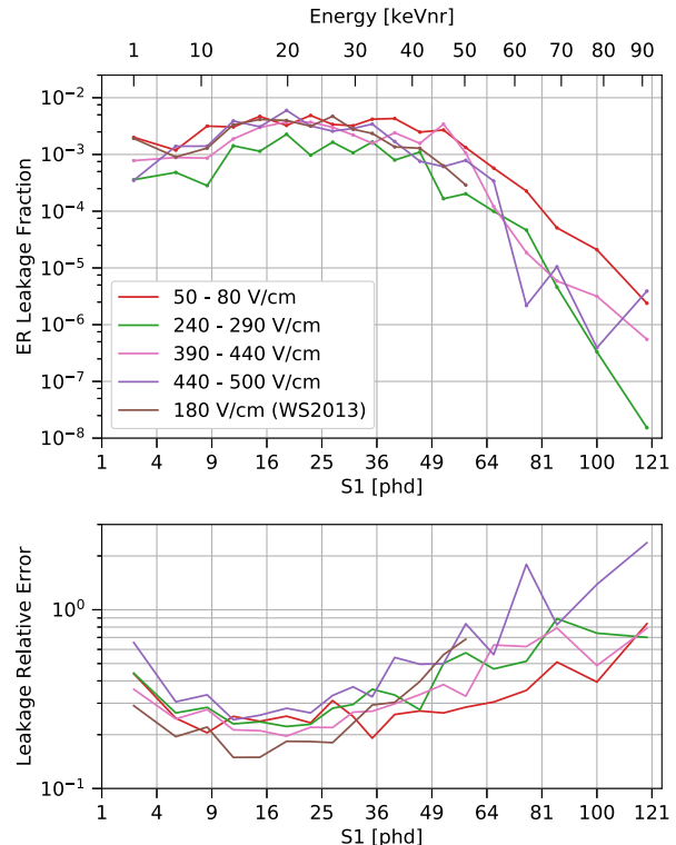
FIG. 12. Top: the electronic recoil leakage fraction for a flat energy spectrum in S1 bins, for various values of drift field, calculated from a skew-Gaussian extrapolation of the ER band below the NR band median. The S1 axis is proportional to \sqrt{S1} . The equivalent nuclear recoil energy for an S1 is calculated by using the S1 and S2c at the median of the NR band; this varies by field, but not significantly, so we report the energy averaged over the eight field bins. The leakage fraction calculated in this way is consistent with the real counted leakage, except in the lowest S1 bin; see Fig. 29 for a comparison between the two leakage calculations in this S1 bin. Bottom: the relative error on these leakage fraction values, defined as \text{leakage\_fraction\_error}/\text{leakage\_fraction} . Note that the leakage relative error can be greater than 1, indicating that the leakage fraction is consistent with 0. See Fig. 28 for the leakage across all the field bins in the data set.
