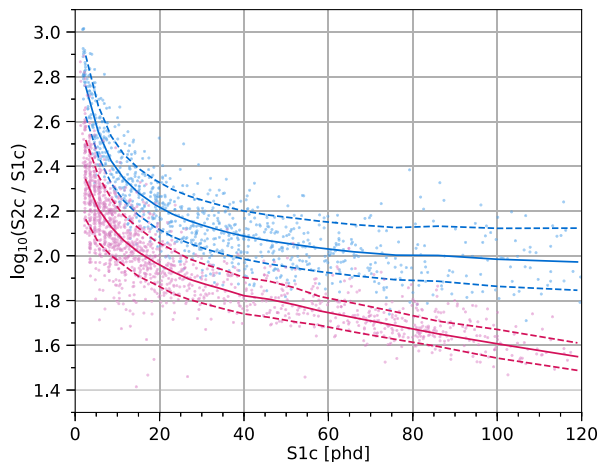
FIG. 5. A sample of electronic and nuclear recoils along with the associated bands. A randomly selected 1500 electronic (nuclear) recoils from WS2014–16 are shown in blue (red) dots, the median of the ER (NR) band is shown as a solid blue (red) line, and the 15.9th percentile and 84.1th percentile of the ER (NR) band are shown as dashed blue (red) lines. Details on the calculation of the ER and NR band can be found in Secs. III A and III B, respectively.
