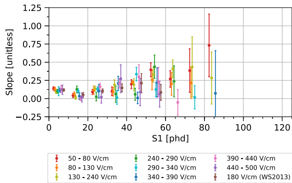
FIG. 32. The slope of the two-factor discrimination line in \log_{10}(S2c/S1) vs prompt fraction space for each S1 and field bin. Missing points represent bins for which charge-to-light discrimination alone gives zero electronic recoils falling below the NR band. The plotted S1 values are slightly shifted relative to their true value (by up to 2.6 phd) for ease of visualization. The true S1 coordinates are 5, 15, 25 phd, etc.
