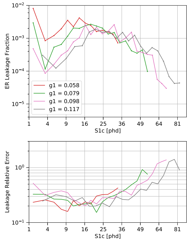
FIG. 10. Top: the electronic recoil leakage fraction for a flat energy spectrum in S1c bins, for various values of g_1 , calculated from a skew-Gaussian extrapolation of the ER band below the NR band median. The S1c axis is proportional to \sqrt{S1c} . The leakage fraction calculated in this way is consistent with the real counted leakage, except in the lowest S1c bin; see Fig. 27 for a comparison between the two leakage calculations in this S1c bin. Bottom: the relative error on these leakage fraction values, defined as leakage_fraction_error/leakage_fraction . Note that the leakage relative error can be greater than 1, indicating that the leakage fraction is consistent with 0. See Fig. 26 for the leakage across all the g_1 bins in the data set.
