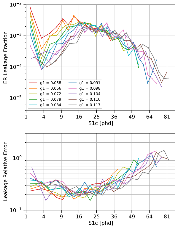
FIG. 26. Top: the electronic recoil leakage fraction for a flat energy spectrum in S1c bins, for various values of g_1 , calculated from a skew-Gaussian extrapolation of the ER band below the NR band median. The S1c axis is proportional to \sqrt{S1c} . The leakage fraction calculated in this way is consistent with the real counted leakage, except in the lowest S1c bin; see Fig. 27 for a comparison between the two leakage calculations in this S1c bin. Bottom: the relative error on these leakage fraction values, defined as \text{leakage\_fraction\_error}/\text{leakage\_fraction} . Note that the leakage relative error can be greater than 1, indicating that the leakage fraction is consistent with 0.
