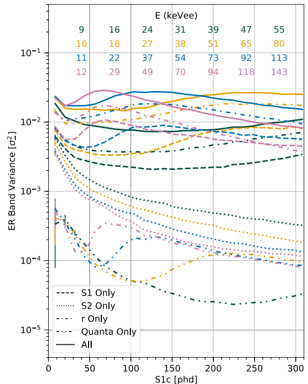
FIG. 21. The ER band variance \sigma_{-}^2 for different types of fluctuations and fields, based on simulation from LUX-NESTv2. Color represents electric field: dark green, gold, blue, and magenta represent 180, 500, 1000, and 2000 V/cm, respectively. Line style represents the types of fluctuations that are turned on in the simulation: dot-dot-dashed lines are fluctuations in the number of quanta, dotted lines are S2 fluctuations, dashed lines are S1 fluctuations, dot-dashed lines are recombination fluctuations, and solid lines are all fluctuations turned on simultaneously (i.e., the default status for LUX-NESTv2). All points have associated error bars, but most are too small to be visible, except for points in the lowest S1c bin. If the fluctuations were uncorrelated, the solid lines would represent the sum of all the other lines for each field, but there are small correlations, so this is not quite true. For a given field, the difference between the solid line and the sum of the other lines is at most 12% except in the lowest S1c bin, where the total variance can be as much as double the sum of the individual component variances. At the top of the figure, we show the electronic equivalent energy for S1c in multiples of 40 phd, for each electric field.
