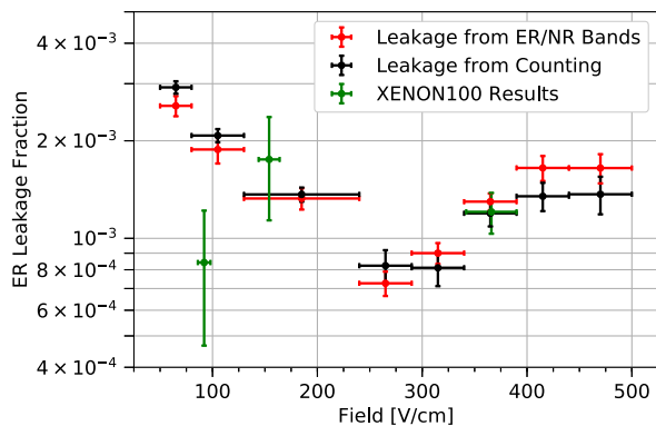
FIG. 13. The integrated electronic recoil leakage for a flat recoil energy spectrum from 1 to 80 S1 photons detected (equivalent to 2–65 keVnr), while varying drift field in WS2014–16 data. The leakage is calculated by either counting the number of electronic recoils falling below the NR band (black), or by integrating the electronic recoil skew-Gaussian fits below the NR band (red). Our optimal field over the range examined is \sim 300 V/cm, which is within the expected drift field range of the forthcoming LZ experiment and matches LZ’s design specification of 310 V/cm. However, an exact quantitative prediction of the LZ leakage is impossible because of the higher expected g_1 and g_2 in LZ [10]. Results from XENON100 [34] are shown in green, where we use their leakages at g_1 = 0.081 (our results are at g_1 = 0.087 ). The XENON100 leakages correspond to 8–32 photons detected, i.e., 11–34 keVnr.
