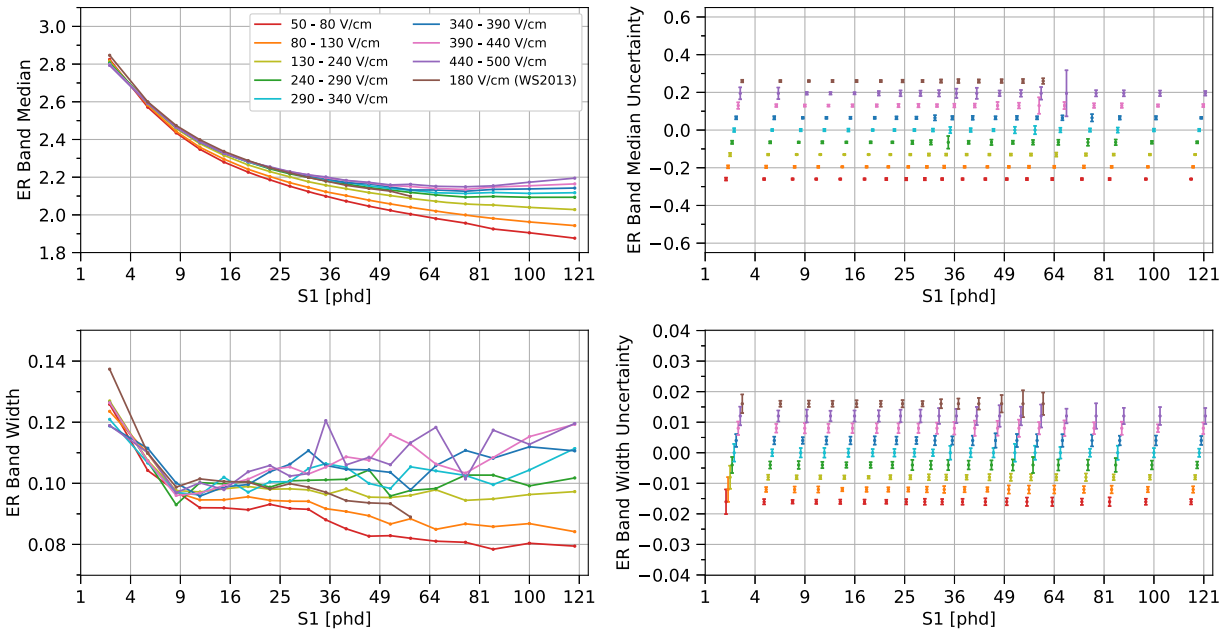
FIG. 24. The median and width \sigma_- of the ER band for several drift fields. The left plots show measurements, and the right plots display error bars corresponding to these measurements. The S1 axis is proportional to \sqrt{S1} . The ER band for WS2013 is adjusted so g_2 is consistent for the WS2013 and WS2014–16 results. In each row, the y-axes have the same range; the size of the error bars on the right plot can be directly translated to the points on the left plot. For ease of visualization on the right plots, the S1 values are slightly shifted relative to their true value, and the error bars are centered at a different y-value for each field bin.
