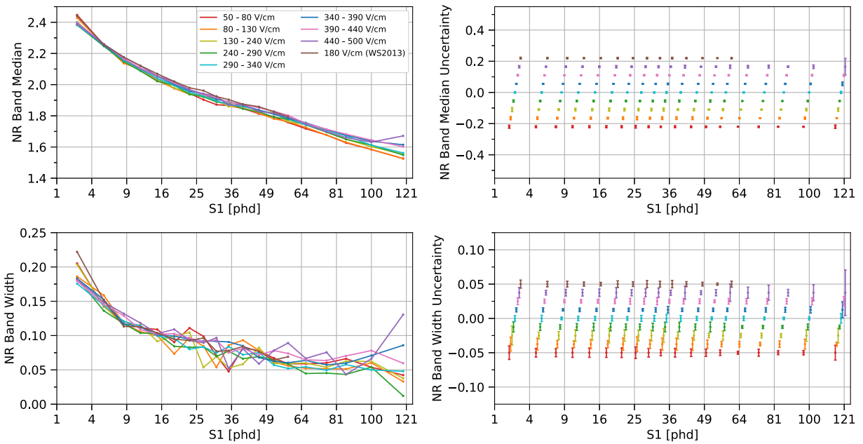
FIG. 25. The median and width \sigma_- of the NR band for several drift fields. The left plots show measurements, and the right plots display error bars corresponding to these measurements. The S1 axis is proportional to \sqrt{S1} . The NR band for WS2013 is adjusted so g_2 is consistent for the WS2013 and WS2014–16 results. In each row, the y-axes have the same range; the size of the error bars on the right plot can be directly translated to the points on the left plot. For ease of visualization on the right plots, the S1 values are slightly shifted relative to their true value, and the error bars are centered at a different y-value for each field bin.
