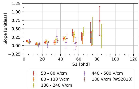
FIG. 17. The slope of the two-factor discrimination line in \log_{10}(S2c/S1) vs prompt fraction space, for each S1 and field bin. Missing points represent bins for which charge-to-light discrimination alone gives zero electronic recoils falling below the NR band. The plotted S1 values are slightly shifted relative to their true value (by up to 2 phd) for ease of visualization. The true S1 coordinates are 5, 15, 25 phd, etc. See Fig. 32 for the slopes across all the field bins in the data set.
