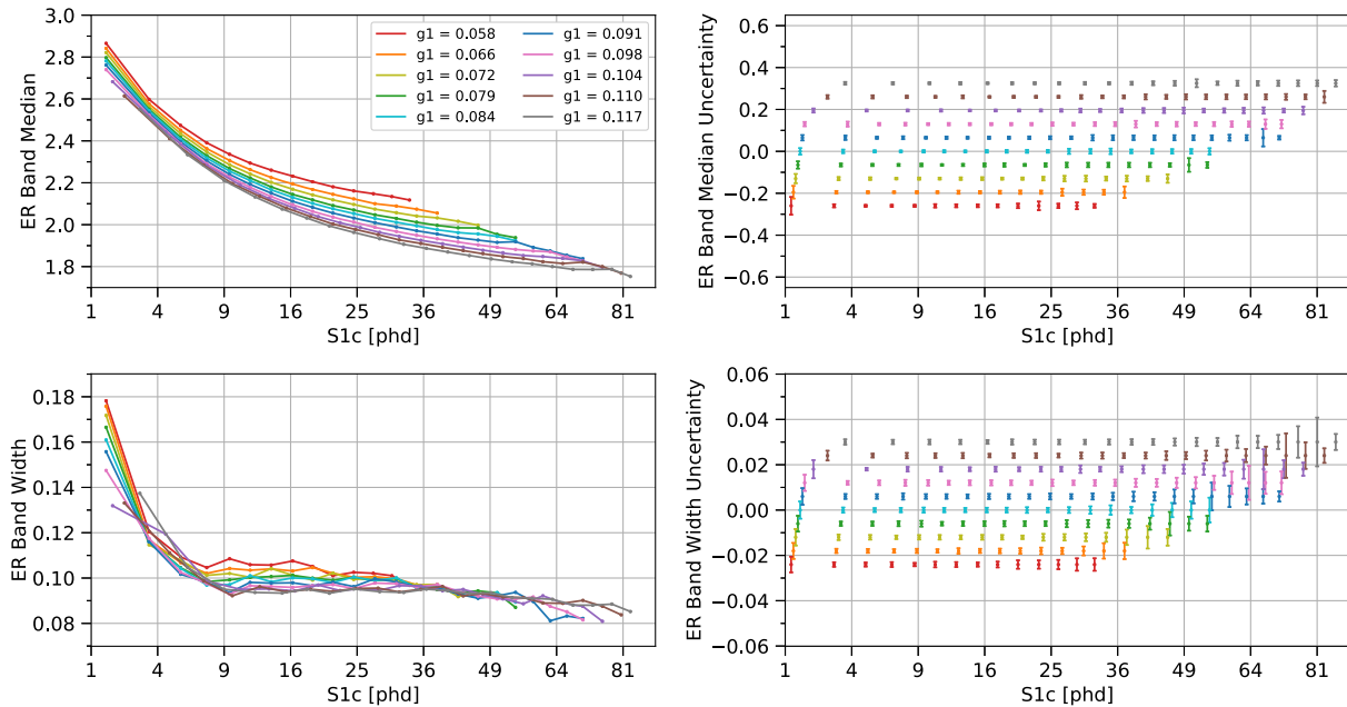
FIG. 22. The median and width \sigma_- of the ER band for several values of g_1 , using WS2013 data. The left plots show measurements, and the right plots display error bars corresponding to these measurements. The S1c axis is proportional to \sqrt{S1c} . In each row, the y-axes have the same range; the size of the error bars on the right plot can be directly translated to the points on the left plot. For ease of visualization on the right plots, the S1c values are slightly shifted relative to their true value, and the error bars are centered at a different y-value for each g_1 . Note the S1c range varies for each g_1 because as g_1 decreases, the {}^3\text{H} end point in S1c space decreases.
