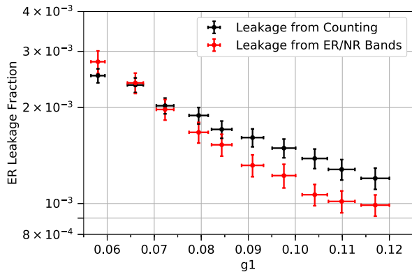
FIG. 11. The integrated electronic recoil leakage for a flat recoil energy spectrum from 0 to 9.7 keVee, while varying g_1 in WS2013 data. The max S1c is proportional to 50 photons detected at g_1 = 0.117 . The leakage is calculated by either counting the number of electronic recoils falling below the NR band (black), or by integrating the electronic recoil skew-Gaussian fits below the NR band (red). The discrepancy between the two methods is explained by a poor fit of the data to a skew-Gaussian distribution in the lowest S1c bin. Statistical errors from Poisson fluctuations are shown.
