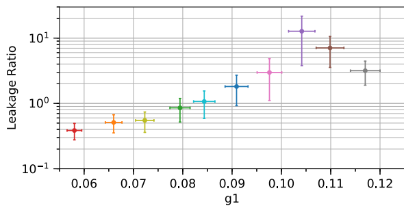
FIG. 27. The ratio of the real (counted) electronic recoil leakage fraction to the estimated leakage fraction from a skew-Gaussian extrapolation of \log_{10}(S2c/S1c) in the lowest S1c bin. This ratio is shown vs g_1 , using WS2013 data. The color of each data point is degenerate with the g_1 value; it is included for consistency with other figures.
