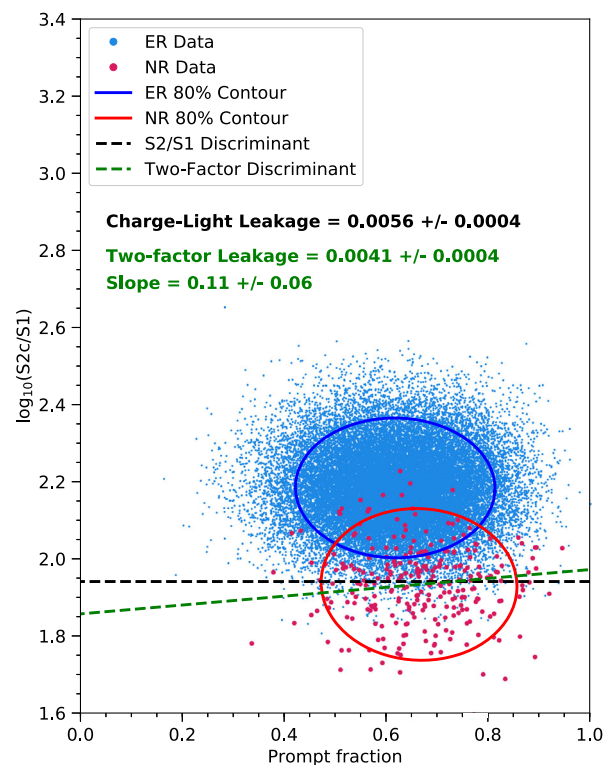
FIG. 14. An example of how the two-factor leakage is calculated, using data for 80–130 V/cm and 20–30 phd. The electronic recoil and nuclear recoil data are plotted on axes of charge-to-light vs prompt fraction. Ellipses containing 80% of the data are shown. The black dashed line shows the nuclear recoil median in \log_{10}(S2c/S1) only, and the black text shows the corresponding electronic recoil leakage fraction. The green dashed line shows the optimized discriminating line between the two distributions; the green text shows the resulting electronic recoil leakage, as well as the slope of this line. We note about 27% improvement in the leakage fraction. Further details on this calculation can be found in the text.
