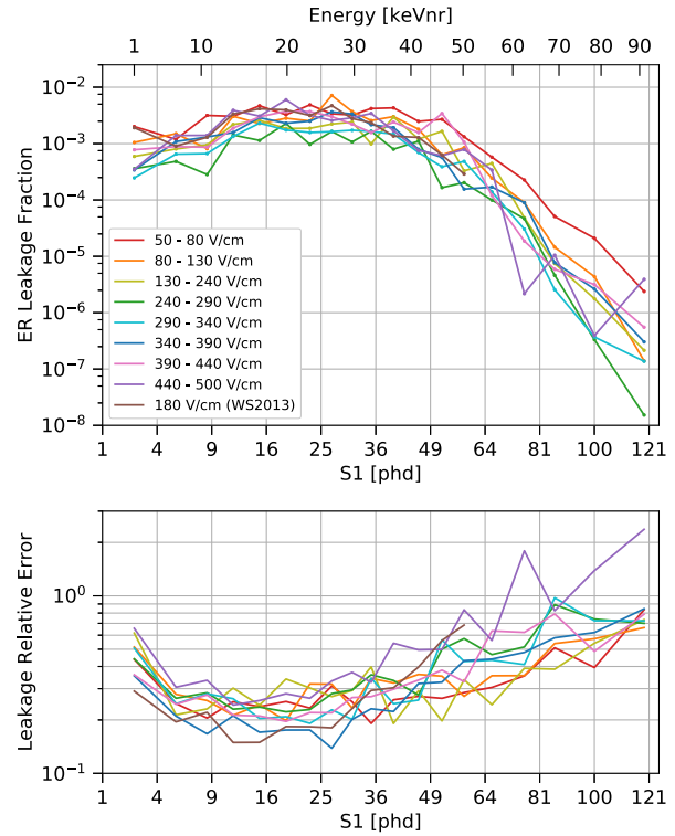
FIG. 28. Top: the electronic recoil leakage fraction for a flat energy spectrum in S1 bins, for various values of drift field, calculated from a skew-Gaussian extrapolation of the ER band below the NR band median. The S1 axis is proportional to \sqrt{S1} . The equivalent nuclear recoil energy for an S1 is calculated by using the S1 and S2c at the median of the NR band; this varies by field, but not significantly, so we report the energy averaged over the eight field bins. The leakage fraction calculated in this way is consistent with the real counted leakage, except in the lowest S1 bin; see Fig. 29 for a comparison between the two leakage calculations in this S1 bin. Bottom: the relative error on these leakage fraction values, defined as \text{leakage\_fraction\_error}/\text{leakage\_fraction} . Note that the leakage relative error can be greater than 1, indicating that the leakage fraction is consistent with 0.
