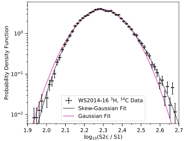
FIG. 4. An example histogram of \log_{10}(\text{S2c/S1}) for electronic recoil data, and associated fits to a skew-Gaussian and Gaussian distribution. The events have an S1 signal between 13 and 16 phd and a drift field between 80 and 130 V/cm; they are weighted based on their energy as described in Sec. III A. The best-fit skew-Gaussian parameters are \xi = 2.222 \pm 0.003 , \omega = 0.128 \pm 0.002 , and \alpha_B = 1.14 \pm 0.06 . The best-fit Gaussian parameters are \mu = 2.2941 \pm 0.0010 and \sigma = 0.1018 \pm 0.0010 .
