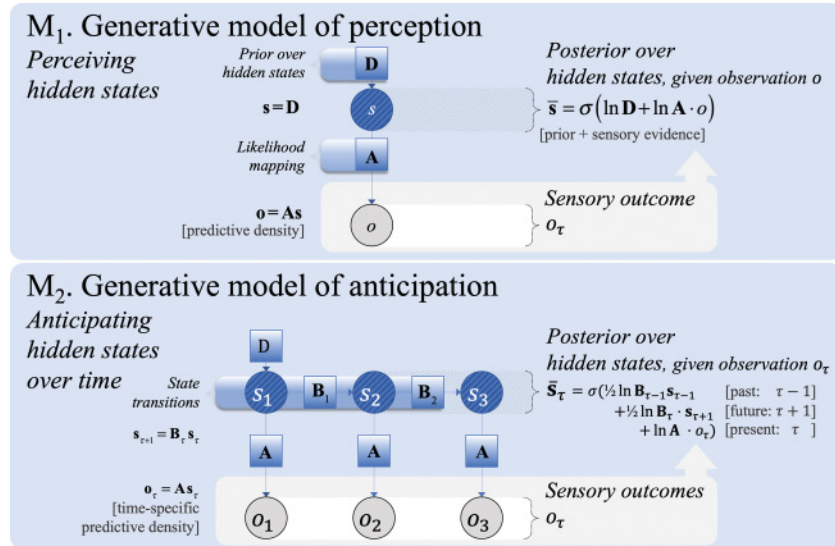
Figure 1: The first ( M_1 , top panel) and second steps ( M_2 , bottom panel) of a generative model of increasing complexity. M_1 : A minimal generative model of perception can infer hidden states s from an observation o , based on prior beliefs ( \mathbf{D} ) and a likelihood mapping ( \mathbf{A} ). M_2 : A generative model of anticipation extends perception (as in M_1 ) forward into the future (and backward into the past) using a transition matrix ( \mathbf{B}_t ) for hidden states.
