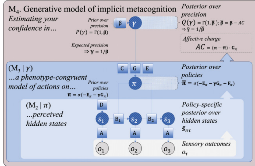
Figure 3: The fourth step ( M_4 ) of our incremental description of active inference in terms of the nested processes of perception ( M_{1-2} in Figure 1), action ( M_3 in Figure 2), and implicit metacognition ( M_4 in this figure), emphasizing the inherently hierarchical, recurrent nature of these generative models. This generative model infers confidence in its own action model in terms of the expected precision ( \gamma ), which modulates reliance on G_\pi for policy selection (as in M_3 ), based on perceptual inferences (as in M_2 ). Expected precision ( \gamma ) changes when inferred policies differ from expected policies. This term increases when posterior (policy-averaged) expected free energy is lower than when averaged under the policy prior ( AC = (\pi - \bar{\pi}) \cdot G_\pi < 0 ), and decreases when it is higher ( AC > 0 ).
