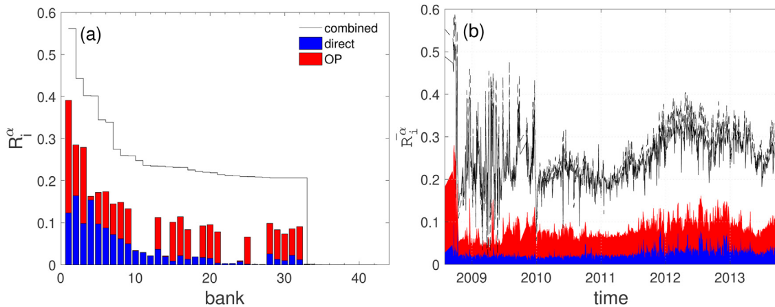
Fig. 3. (a) SR profile for the different layers. Normalized DebtRank \hat{R}_i^{\alpha} (see Section 2.2) from different layers are stacked for each bank. SR contribution due to overlapping portfolios are shown in red and due to direct exposures in blue. Banks are ordered according to their DebtRank in the combined network from all layers (line). (b) Time series for the average DebtRank \bar{R}^{\alpha}(t) = \frac{1}{b} \sum_{i=1}^b \hat{R}_i^{\alpha}(t) for all layers from 31 July 2008 to 30 September 2013. The black and the dashed lines show the average and the median DebtRank for all layers combined, respectively. (For interpretation of the references to color in this figure legend, the reader is referred to the web version of this article.)
