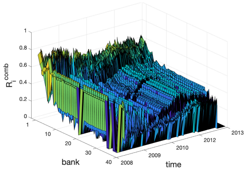
Fig. 4. SR surface for the combined network from all layers. DebtRanks in the combined network from all layers ( \hat{R}_i^{\text{comb}}(t) ) are shown for each bank from 31 July 2008 to 30 September 2013. Banks are ordered according to their DebtRanks from 30 September 2013.
