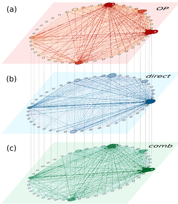
Fig. 2. Multi-layer banking network of Mexico. (a) Network of indirect external exposures from overlapping portfolios, X_{ij}^{OP}(t) , (b) network of direct interbank exposures X_{ij}^{direct}(t) , and (c) combined banking network X_{ij}^{comb}(t) . The network of indirect exposures is the bank-projection of the bipartite network, S_{ia}(t) , of banks and assets. Nodes (banks) are colored according to their systemic importance, R_i^\alpha , in the respective layer (see Section 2.2): from systemically important banks (red) to systemically safe (green). Node size represents banks' total assets. Link width is the exposure size between banks (re-scaled), link color is taken from the counterparty. (For interpretation of the references to color in this figure legend, the reader is referred to the web version of this article.)
