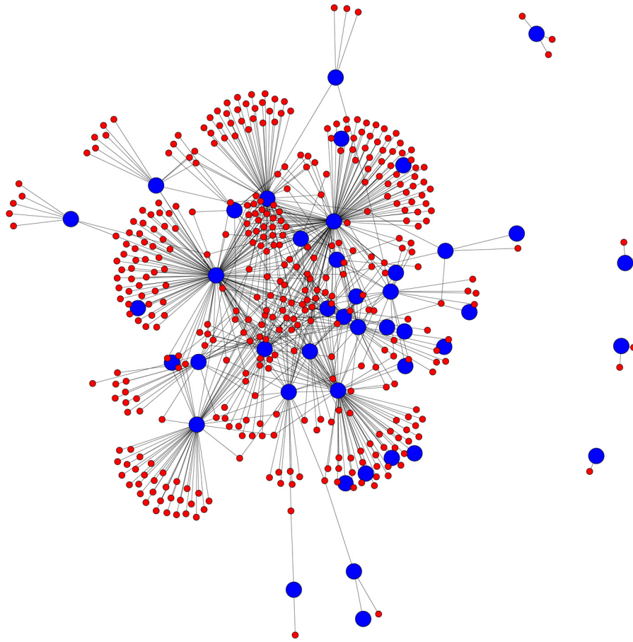
Fig. 1. Bank-asset bipartite network of the Mexican financial system on a particular day. Nodes in the network represent banks (blue) and assets (red). Links between an asset and a bank exist if the bank holds the asset in its portfolio. (For interpretation of the references to color in this figure legend, the reader is referred to the web version of this article.)
