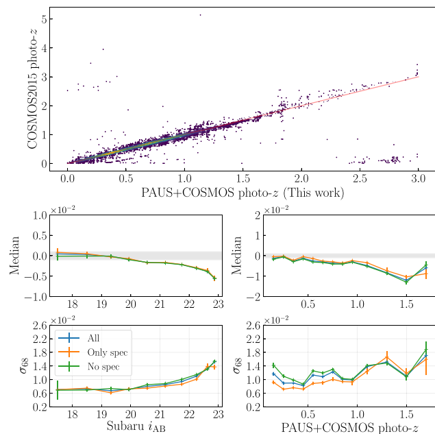
Figure 11. Performance of the complete sample. The top row shows the scatter plot between the photo- z from PAUS + COSMOS and the photo- z from (Laigle et al. 2016). The middle and bottom row show the median and \sigma_{68} of the quantity \Delta_z \equiv (z_{\text{COSMOS2015}} - z_{\text{P+C}})/(1 + z_{\text{P+C}}) , where z_{\text{COSMOS2015}} and z_{\text{P+C}} are the photo- z from COSMOS2015 and PAUS + COSMOS, as a function of the Subaru i -band (left-hand panels) and the PAUS + COSMOS photo- z (right-hand panels). In the bottom panels, the blue lines show results for all objects in the catalogue, the orange lines for the subset that has spectra, and the green lines for the subset that does not have spectra.
