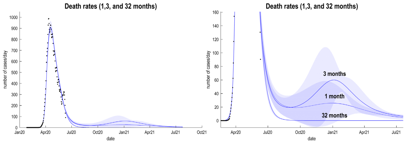
Figure 5. Second waves. This figure reports the expected death rates as a function of time for the effective United Kingdom population. The three trajectories (blue lines) and accompanying 90% Bayesian credible intervals (shaded areas) correspond to posterior predictions with a loss of immunity over 1, 3 and 32 months. These represent the smallest, most likely and longest period of immunity considered in the Bayesian model comparison (summarised in the previous figure). The black dots correspond to empirical data, after smoothing with a four-day Gaussian kernel. The right panel reproduces the data in the left panel with a focus on the second wave peaking in January of next year.
