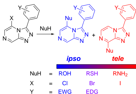
Figure 10: Summary of ipso - and tele -substitution reactions observed with 5-halo-1,2,4-triazolo[4,3- a ]pyrazines. Increased levels of tele -substitution observed (i) when X = I > Br > Cl, and (ii) when NuH = RNH 2 > RSH > ROH.
