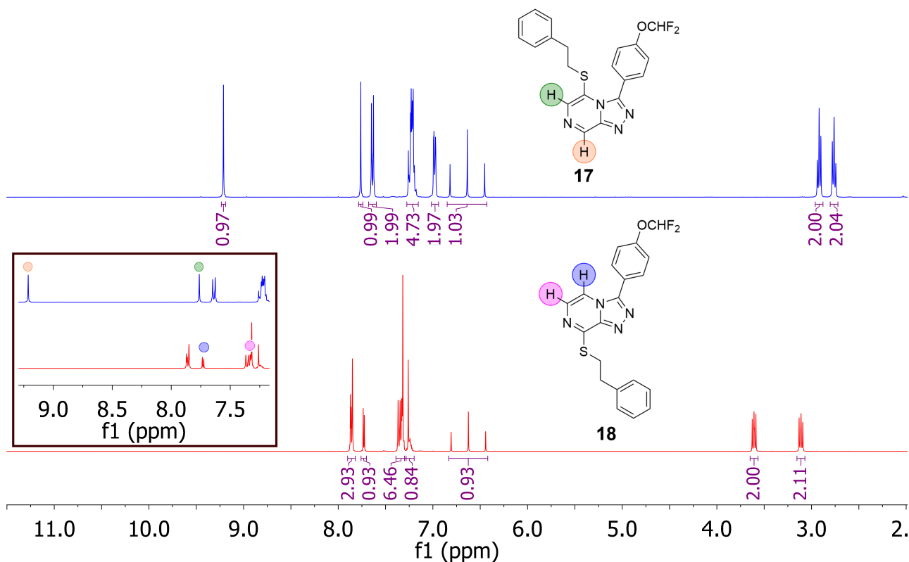
Figure 4: 1 H NMR spectra of 17 and 18 in CDCl 3 . The hydrogen atoms on the pyrazine ring for the 5-substituted isomers (highlighted in green and orange in 17 ) give rise to sharp singlets ( \delta \sim 7.5 and \sim 9.0 ppm), while those in the 8-substituted isomers (highlighted in pink and blue in 18 ) give well-defined doublets ( \delta \sim 7.2 – 7.7 ppm, J = 4.6 Hz).
