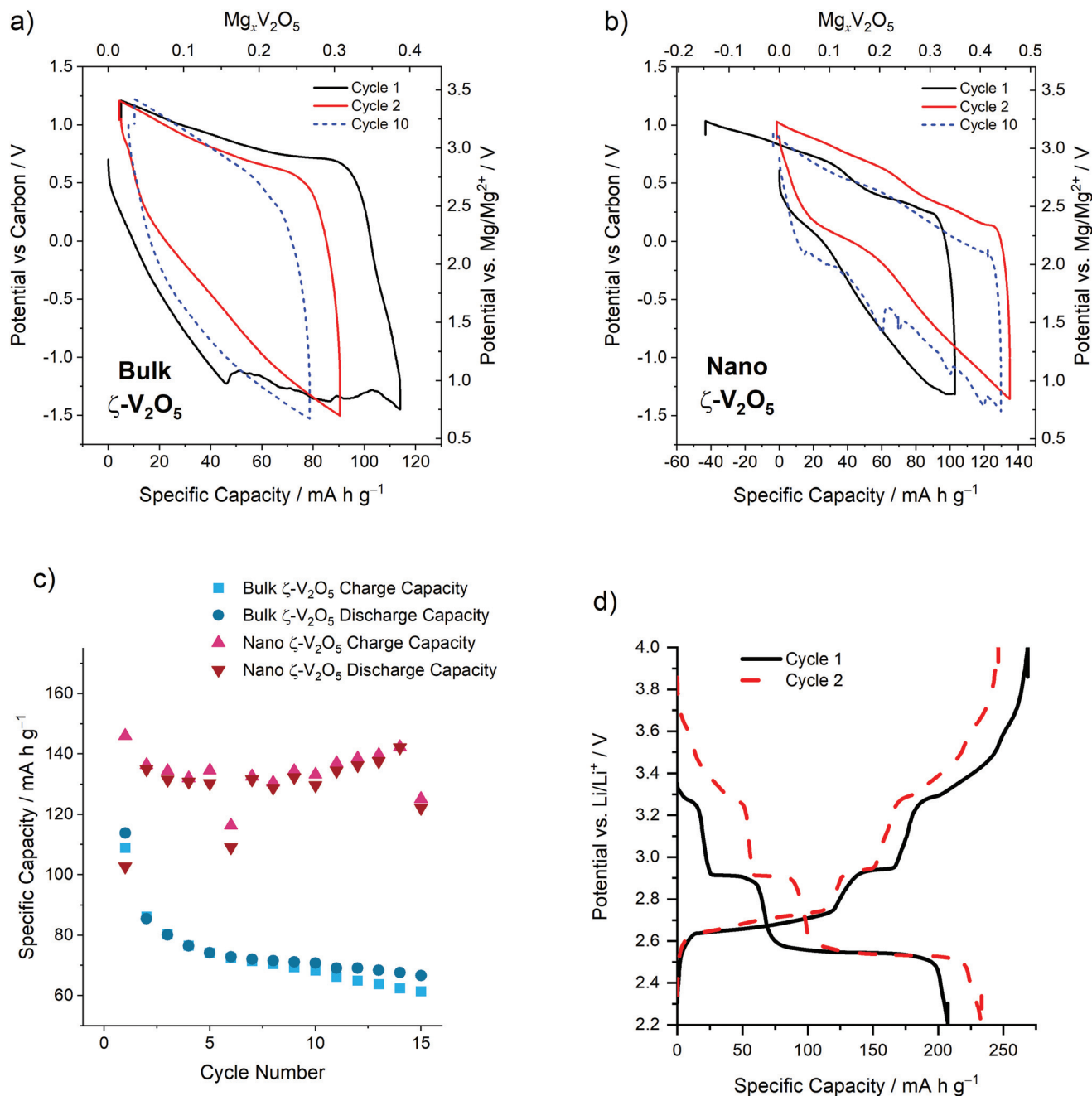
Fig. 2 Electrochemical measurements performed at an elevated temperature of 110 °C: (a) the first, second and tenth cycles of Bulk \zeta\text{-V}_2\text{O}_5 cycled in the range 1.2 to -1.7 V (vs. ACC) in an Mg-ion cell, (b) the first, second and tenth cycles of Nano \zeta\text{-V}_2\text{O}_5 cycled in the range 1.2 to -1.7 V (vs. ACC) in an Mg-ion cell, (c) comparison of the charge and discharge capacities of Bulk and Nano \zeta\text{-V}_2\text{O}_5 in Mg-ion cells as a function of cycle number, (d) the first two cycles of Nano \zeta\text{-V}_2\text{O}_5 cycled in the range 4.0 to 2.2 V (vs. Li/Li + ) at a C/10 charge/discharge rate in a Li-ion cell at room temperature.
