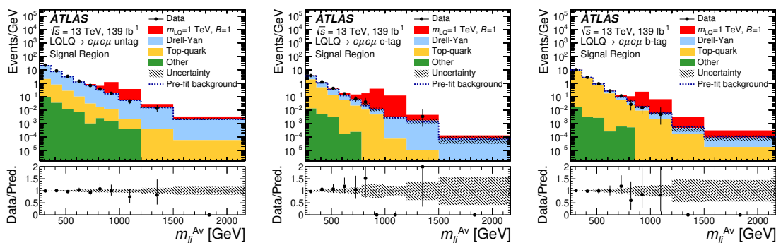
Figure 5. Post-fit distributions of m_{l_j}^{Av} in the c\mu signal regions: untagged (left), c -tag (middle), and b -tag (right). The expected signals, shown for m_{LQ} = 1 TeV and \mathcal{B}(LQ \rightarrow c\mu) = 1 , are shown for illustrative purposes. The category ‘Top-quark’ refers to t\bar{t} and single-top-quark processes. The category ‘Other’ refers to diboson and W +jet production. The hatched band represents the total uncertainty in the background predictions.
