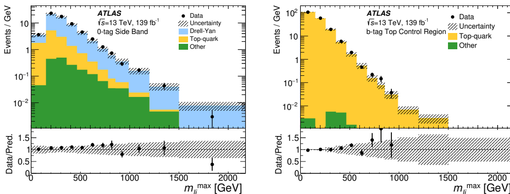
Figure 2. Distributions of m_{\ell j}^{\max} in the combined b\bar{e} and b\mu 0-tag SB for the b\bar{l} channels (left) and the b -tag Top CR for the c\bar{l} channels (right). The total modelling uncertainty combined with the MC statistical error is shown as the hatched band as explained in section 7. The category ‘Other’ represents the sum of all SM background contributions except those from top-quark processes ( t\bar{t} and single-top) and, for the 0-tag SB distribution, Drell-Yan processes.
