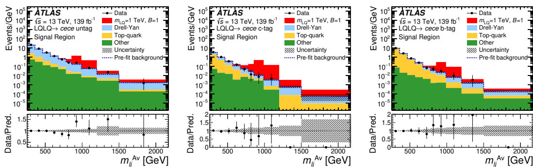
Figure 4. Post-fit distributions of m_{l_j}^{Av} in the ce signal regions: untagged (left), c -tag (middle), and b -tag (right). The expected signals, shown for m_{LQ} = 1 TeV and \mathcal{B}(LQ \rightarrow ce) = 1 , are shown for illustrative purposes. The category ‘Top-quark’ refers to t\bar{t} and single-top-quark processes. The category ‘Other’ refers to diboson and W +jet production. The hatched band represents the total uncertainty in the background predictions.
