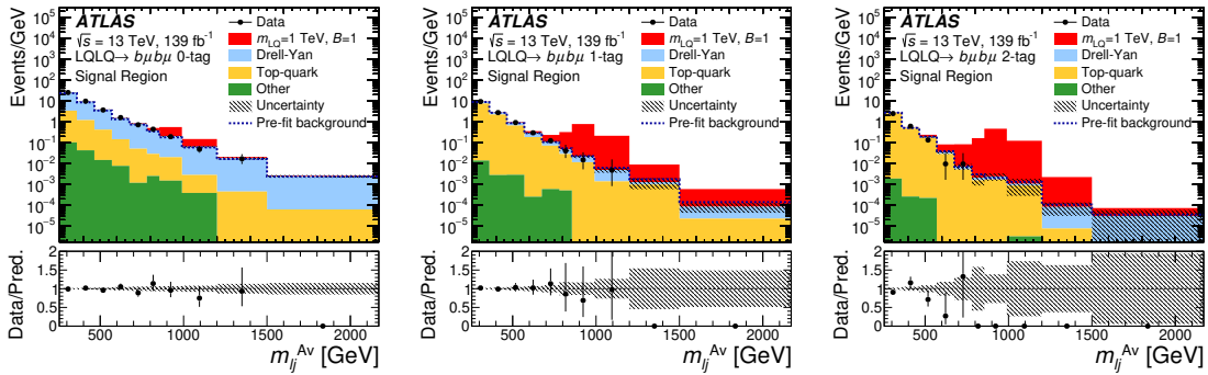
Figure 7. Post-fit distributions of m_{l_j}^{Av} in the b\mu signal regions: 0-tag (left), 1-tag (middle), and 2-tag (right). The expected signals, shown for m_{LQ} = 1 TeV and \mathcal{B}(LQ \rightarrow b\mu) = 1 , are shown for illustrative purposes. The category ‘Top-quark’ refers to t\bar{t} and single-top-quark processes. The category ‘Other’ refers to diboson and W +jet production. The hatched band represents the total uncertainty in the background predictions.
