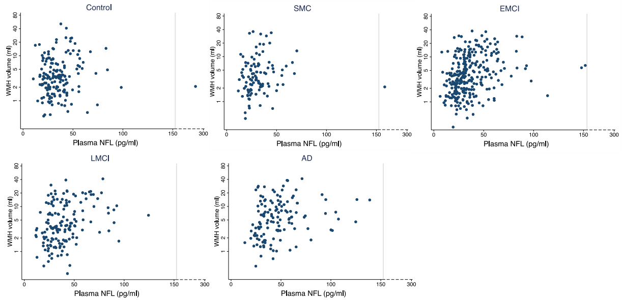
Figure 1: Scatter plots showing the relationship between WMH and plasma NFL in controls, significant memory concern (SMC), early mild cognitive impairment (EMCI), late mild cognitive impairment (LMCI), Alzheimer’s disease (AD) groups. WMH volume is shown on a log scale and is unadjusted for any covariates. There is an x-axis break to show to show the one NFL outlier in both the control and SMC groups.
