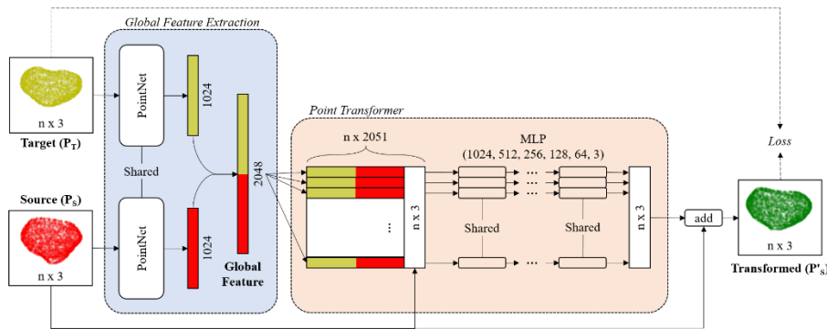
Fig. 1. Schematic representation of the FPT architecture for non-rigid point-set registration.
