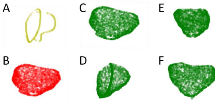
Fig. 4. Registration results from the second experiment on a sparse target (a) and source (b) point-set using ICP (c), CPD (d), FPT (e), and FPT after fine-tuning (f). The complete surface of (a) is identical to Figure 3a.
