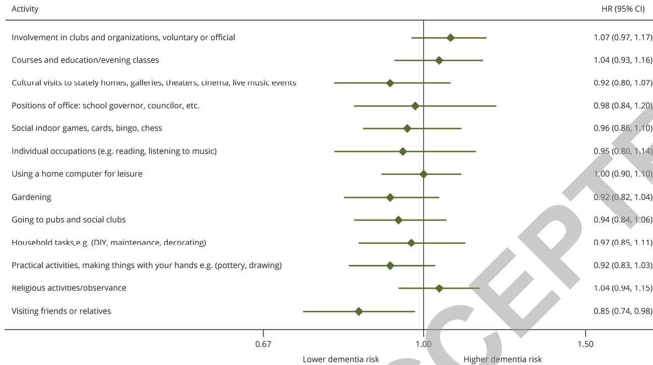
Figure 2. Association of each leisure activity in 1997-99 with subsequent incident dementia
