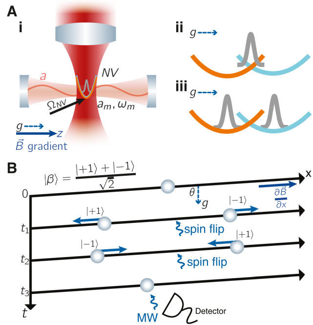
Figure 3: Spin-oscillator coupling has been proposed as a gravimetry technique, whereby a spatial superposition is created through the interaction of an embedded two-level-system such as an NV centre with an external magnetic field gradient. Variations of (A) have been proposed in [68–70]. A MW pulse can be applied to split the spin states of the internal NV centre in a trapped quantum nanosphere (i), which in turn creates a spatial superposition that can be viewed as the splitting of the optical trap (ii) into a superposition (iii). Note that the cavity is used to prepare the nanosphere in the ground state and can be switched off during (ii and iii). (B) Allowing for free evolution increases the spatial size of the superposition, created and probed in a Ramsey-type interferometer, as proposed by [74]. Here, the coupled NV-nanosphere superposition is prepared with a MW pulse at time t_1 , undergoing free-fall until the spins are flipped at t_2 to enable matter-wave interferometry at t_3 .
