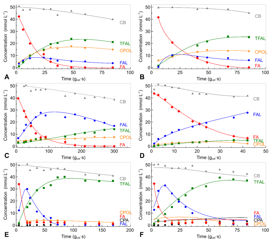
Fig. 7 Concentration profiles for furfural (FA) hydrogenation and the formation of furfuryl alcohol (FAL), tetrahydrofurfuryl alcohol (TFAL), cyclopentanol (CPOL) and cyclopentanone (CPA) as well as the carbon balance (CB). Hydrogenation of a 100 mM FA solution over the Pd/SiO 2 catalyst at (A) 50 °C and 30 bar; (B) 50 °C and 50 bar; (C) 100 °C and 10 bar; (D) 100 °C and 50 bar; (E) 150 °C and 30 bar; (F) 150 °C and 50 bar.
