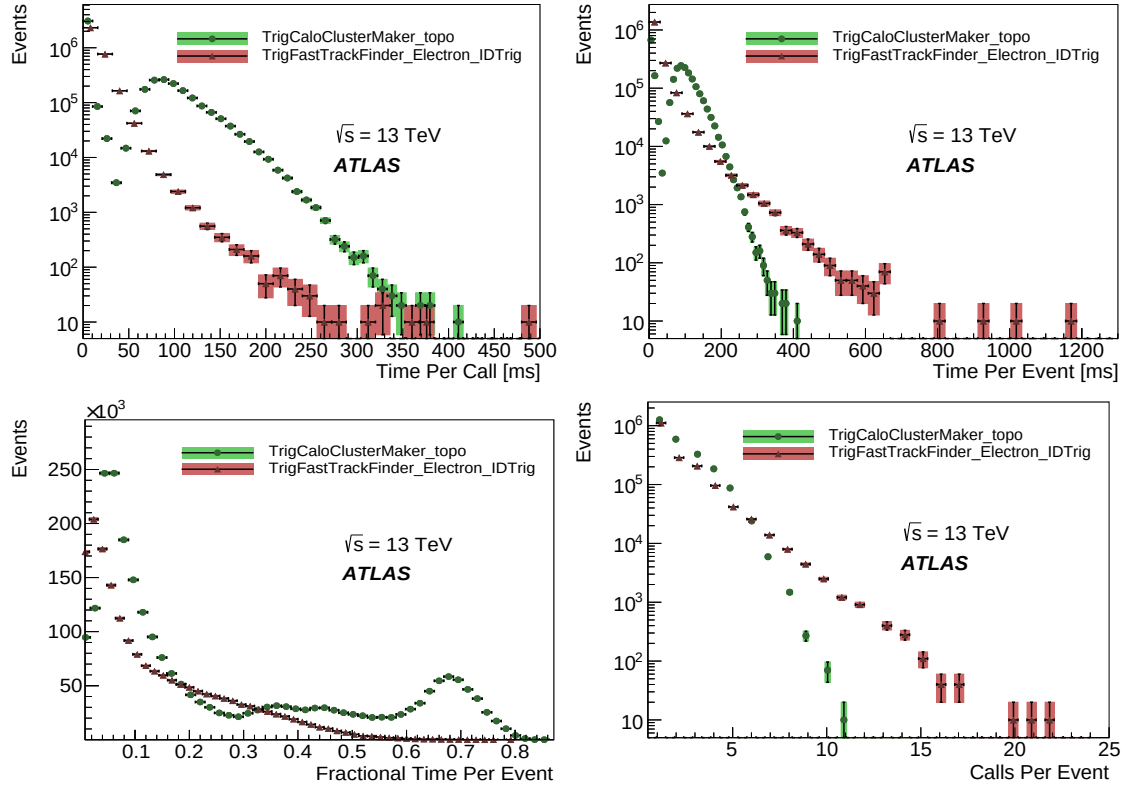
Figure 5. Cost monitoring distributions for two HLT algorithms [42]: the topological clustering of calorimeter data (TrigoClusterMaker_topo) is shown in green and the inner-detector electron track identification (TrigFastTrackFinder_Electron_IDTrig) is shown in red. Presented are the execution time (top) per call (left) and per event (right), as well as the execution time expressed as a fraction of the total execution time of all algorithms (bottom) in the event (left) and number of executions per event (right). Only statistical uncertainties are shown.
