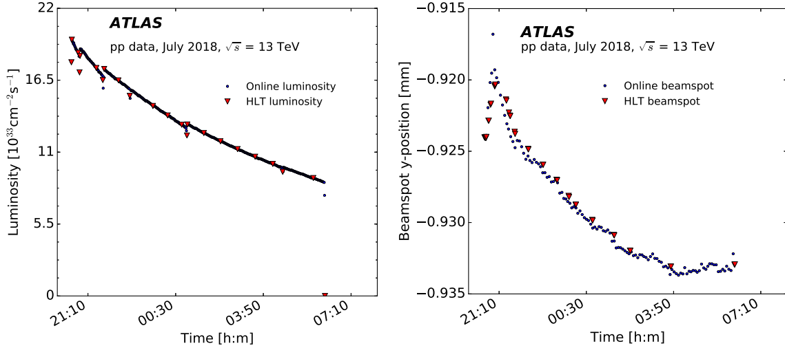
Figure 9. The live values (blue circles) and values used in the HLT (red triangles) of the luminosity (left) and the y-position of the beam spot (right) for a typical pp run. The sudden increases in the luminosity are from the LHC re-optimisation of the colliding beams.
