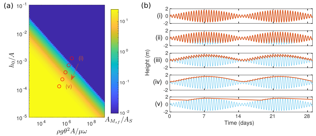
Figure 3. (a) Phase diagram showing the relative amplitudes of the 14-day ( A_{M_{sf}} ) to 12-h ( A_S ) components present in the grounding-line position, as a function of dimensionless downslope gravity \rho g \theta^2 A / \mu \omega and till permeability h_0 / A . (Reduced model, forced by two sinusoidal frequencies with \omega_M / \omega_S = 12.42 / 12 and A_M / A_S = 1.5 ). The points marked with open circles are shown in (b): Blue, tidal height, and red, grounding-line height. For very low permeability, the grounding line is pinned at the point of highest tide. As permeability increases, the high frequency components are more weakly filtered.
