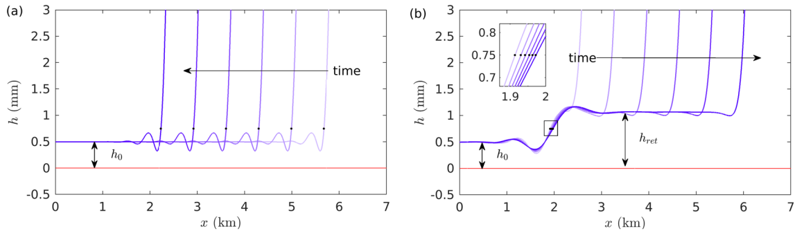
Figure 2. Results of a full numerical simulation for ocean height changing at constant speed of 2 \times 10^{-4} \text{ ms}^{-1} over a bedslope of \theta = 10^{-3} with h_0 = 0.5 \text{ mm} , B = 10^{16} \text{ kgm}^2 \text{ s}^{-2} . Color gradient represents passage of time, profiles shown at 1 h intervals. Black dots show the position of the grounding line. (a) As the ocean height rises, the grounding line migrates upwards at the same speed. At the grounding line, we observe flexural waves ahead of the peeling front. (b) As the ocean height falls, the majority of the water is able to drain out, but close to the grounding line, we find that a thin film of water is retained. The top-most extent of the film begins to slowly drain in a manner governed by Equation 8—see inset.
