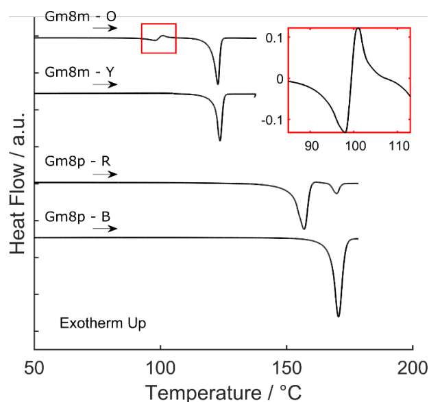
Figure 6 Differential scanning calorimetry thermograms of Gm8m – O and Gm8m – Y (top) and Gm8p – R and Gm8p – B (Bottom). Inset shows an enlarged thermogram of the phase transition of Gm8m – O to Gm8m – Y, vertical axis units are \text{J}\cdot\text{g}^{-1} . The heating rate for Gm8m samples was 5^\circ\text{C}\cdot\text{min}^{-1} and 10^\circ\text{C}\cdot\text{min}^{-1} for Gm8p samples.
