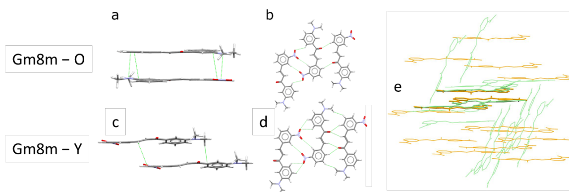
Figure 3. Packing motifs in \text{Gm8m} - \text{O} and \text{Gm8m} - \text{Y} (major component) with close contacts highlighted: a) the double 1-3 ring stacked dimer motif in \text{Gm8m} - \text{O} ; b) cyclic \text{CH}\cdots\text{O}=\text{C} and \text{CH}\cdots\text{NO}_2 motifs in \text{Gm8m} - \text{O} ; c) half-stacking motif in \text{Gm8m} - \text{Y} ; d) cyclic \text{CH}\cdots\text{O}=\text{C} and \text{CH}\cdots\text{NO}_2 motifs in \text{Gm8m} - \text{Y} ; e) 15-molecule overlay of \text{Gm8m} - \text{Y} (in green) and \text{Gm8m} - \text{O} (in orange), with the 3 overlaid molecules in thicker stick representation.
