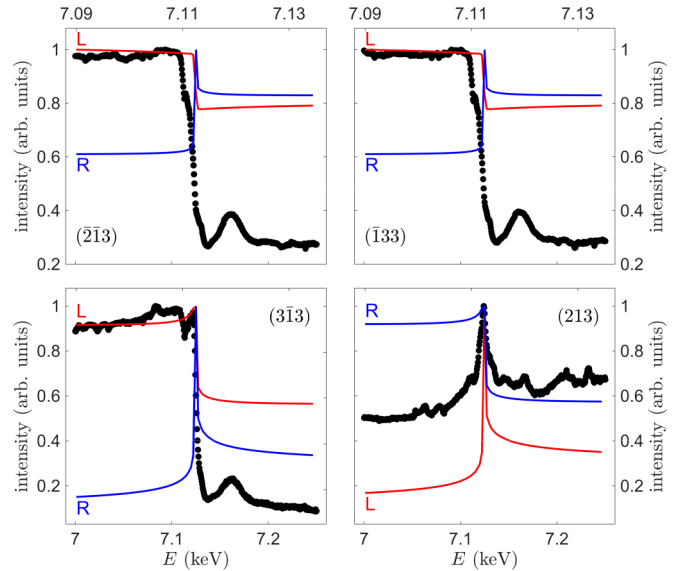
FIG. 9. The behavior of four noncoplanar reflections shows great contrast in the simulations for the left-handed (red lines) and right-handed (blue lines) enantiomers. Black circles represent the renormalized experimental intensity of the four reflections measured in the center of our specimen at room temperature. As is immediately evident, only simulations with the left-handed structure match the trend of the experimental data. No attempt was made to simulate the subtle feature shown by the experimental data across the transition.
