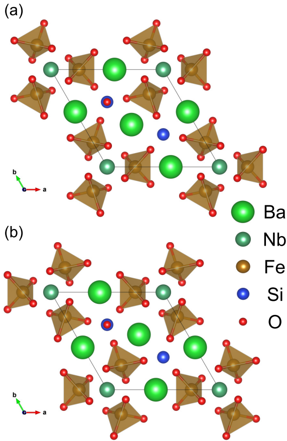
FIG. 1. (a) Left-handed and (b) right-handed crystal structure of \text{Ba}_3\text{NbFe}_3\text{Si}_2\text{O}_{14} . The atomic positions of the left-handed structure [e.g., Fe atom at (0.249\ 0\ 0.5) ] are taken from Ref. [11] and have been inverted for the right-handed structure.
