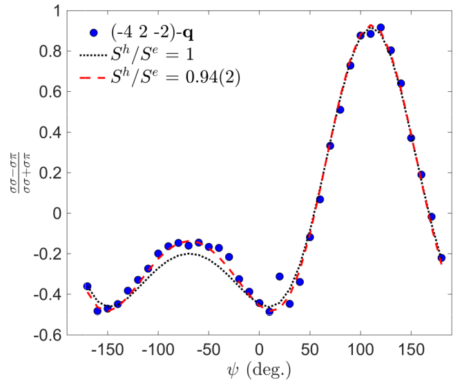
FIG. 11. Azimuthal scan with incident polarization perpendicular to the scattering plane under the nonresonant condition on the (-4\ 2\ -2)-\mathbf{q} reflection. The ellipticity is given by the ratio of the spin component along the hard axis ( S^h ) to that along the easy axis ( S^e ) of the envelope.
