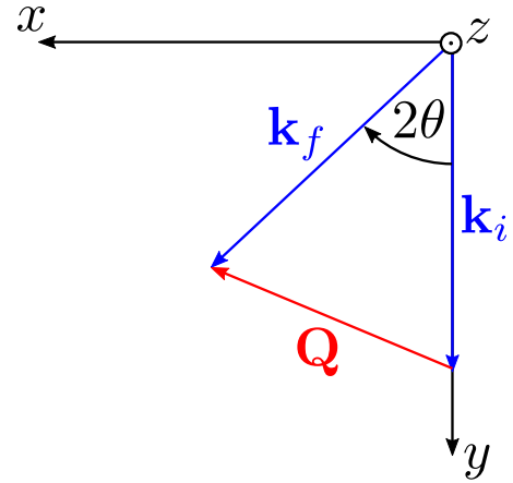
FIG. 3. Definition of the momentum transfer for the formalism presented here. We define the scattering angle in the horizontal plane to be positive for scattering to the right of the incoming beam when viewed from the top.
