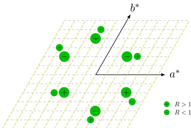
FIG. 6. Sketch of the reciprocal space showing the flipping ratios R of selected Bragg reflections. The observed asymmetries are proportional to the size of the symbols.
