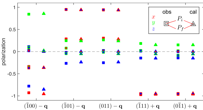
FIG. 8. Observed (squares) and calculated (triangles) polarization values P_{if} for incident neutrons polarized along P_i (inner symbol color) and polarization analysis along P_f (symbol edge color) for the three directions x (red symbols), y (green symbols), and z (blue symbols).
