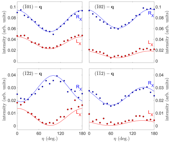
FIG. 10. The x-ray dichroic intensity as a function of the deviation angle \eta of the linear polarization analyzer from the scattering plane for four different magnetic Bragg reflections at T = 5 K. Red circles represent data taken with a photon beam of left-handed polarization; blue squares, data measured with a photon beam of right-handed polarization. The calculated intensities (fitted with a global scale factor) are based on a left-handed enantiomer and are shown as solid lines in the corresponding colors.
