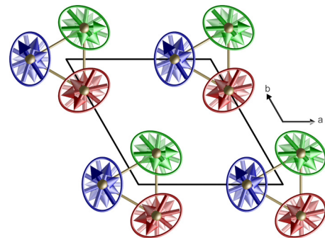
FIG. 7. Visualization of the resulting magnetic structure from the refinement to the polarimetry data. The envelope of the spin modulation along the c axis (decreasing transparency corresponds to an increasing c component) is elliptical, with the main axis perpendicular to the twofold rotation axis being larger than the one along it. This results in a site anisotropy expressed by S^h/S^e = 0.91(3) , which has been exaggerated by a factor of 3 for visibility.
