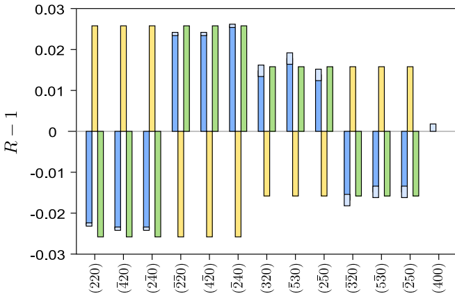
FIG. 5. Bar chart of the observed flipping ratios ( R - 1 ) shown in the left bar of each (hkl) reflection [blue; lighter area represents (R - 1) \pm \sigma ] compared to the calculated values for a left-handed structure (middle bar of each (hkl) reflection; yellow) and a right-handed structure (right bar of each (hkl) reflection; green).
