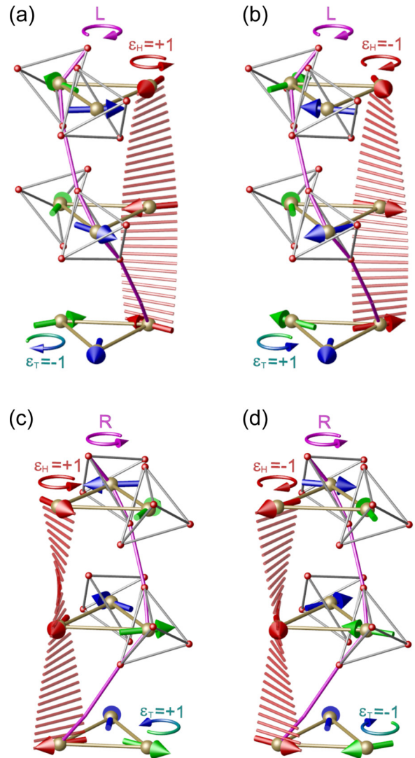
FIG. 2. Four different configurations which all yield the same nuclear and magnetic structure factors. A part of the structure is depicted focusing on a triangular plaquette consisting of three symmetry-equivalent Fe ions at z = \frac{1}{2} which repeat after a translation along c . (a, b) A left-handed (L) crystal structure which is characterized by the antitrigonometric twist of the Fe-O-O-Fe superexchange pathways (shown in magenta). The helical chirality \epsilon_H (rotating cylinders between the spins serve as a guide for the eye) is symbolized by curved arrows on top of the helix. The triangular chirality \epsilon_T is symbolized by a clockwise (negative chirality, \epsilon_T = -1 ) or counterclockwise (positive chirality, \epsilon_T = +1 ) arrow positioned between two spins within a triangle. (c, d) The left-handed structural analogs.
