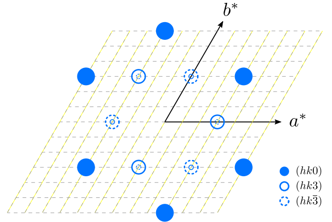
FIG. 4. Sketch of the reciprocal space showing nuclear Bragg reflections \{330\} , \{303\} , and \{033\} . The observed intensities are proportional to the size of the symbols.
